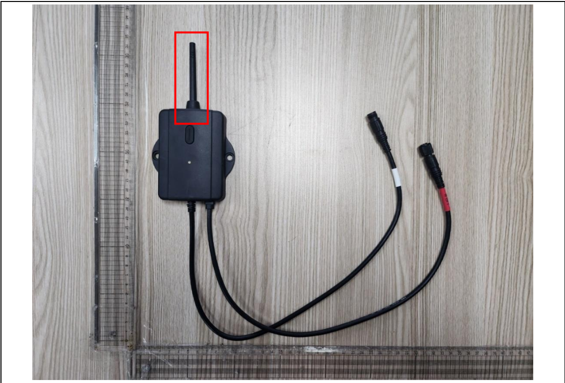
Antenna(2.4GHz ANT)
