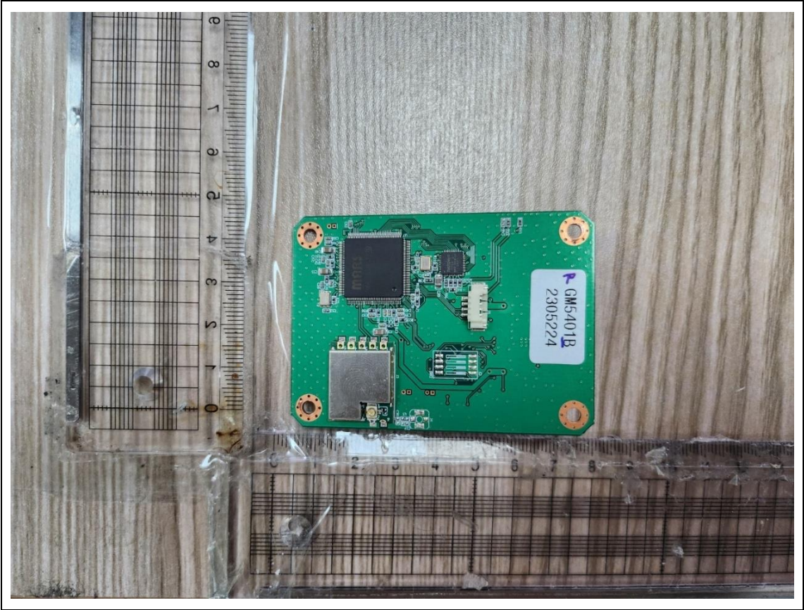
Board-Front(remove shield)
