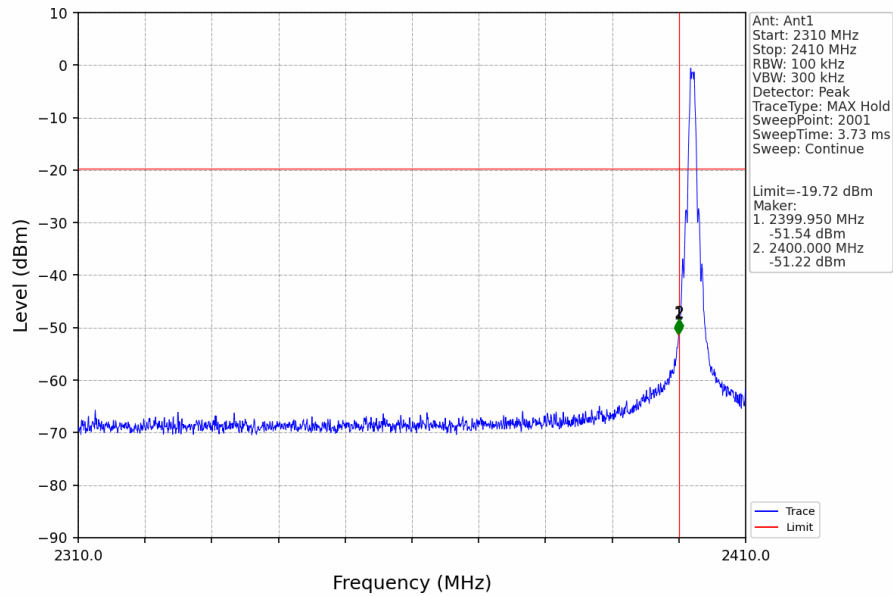
1M_LCH_2402MHz_Ant1_NTNV
