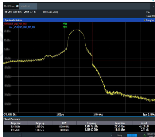
Band25-1.4MHz-QPSK-26683-1RB#5-PASS
