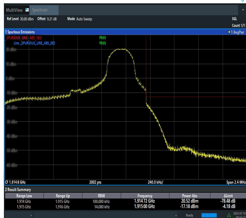
Band25-1.4MHz-16QAM-26683-1RB#5-PASS
