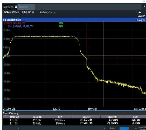
Band25-1.4MHz-QPSK-26683-6RB#0-PASS
