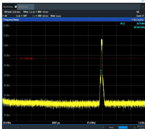
Band12-10MHz-QPSK-23060-50RB#0-30~1000- PASS
