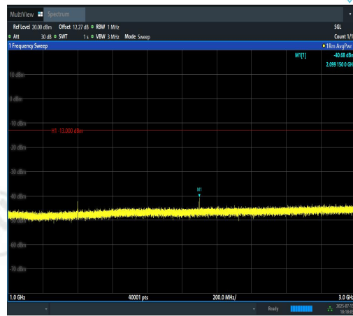
Band12-10MHz-QPSK-23060-1RB#0-1000~300 0-PASS
