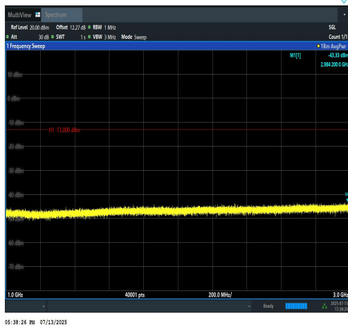
Band12-5MHz-16QAM-23155-25RB#0-1000~30 00-PASS
