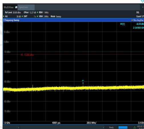
Band12-10MHz-16QAM-23060-1RB#49-1000~3000-PASS
