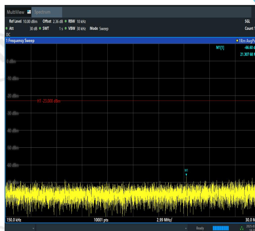
Band12-10MHz-QPSK-23060-50RB#0-0.15~30- PASS
