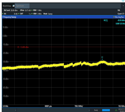
Band12-10MHz-16QAM-23060-1RB#49-3000~10000-PASS
