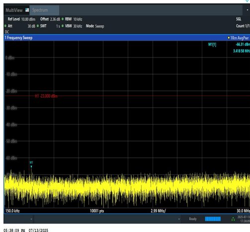
Band12-5MHz-16QAM-23155-25RB#0-0.15~30- PASS
