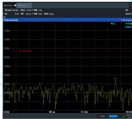
Band12-10MHz-16QAM-23060-1RB#0-0.009~0.15-PASS
