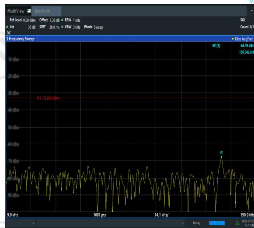
Band12-10MHz-QPSK-23060-1RB#49-0.009~0. 15-PASS
