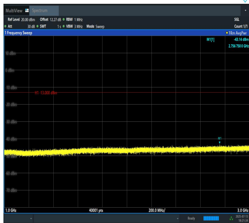
Band12-10MHz-16QAM-23060-50RB#0-1000~3 000-PASS
