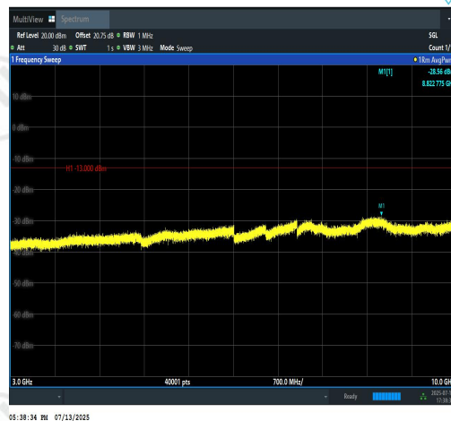
Band12-5MHz-16QAM-23155-25RB#0-3000~10 000-PASS
