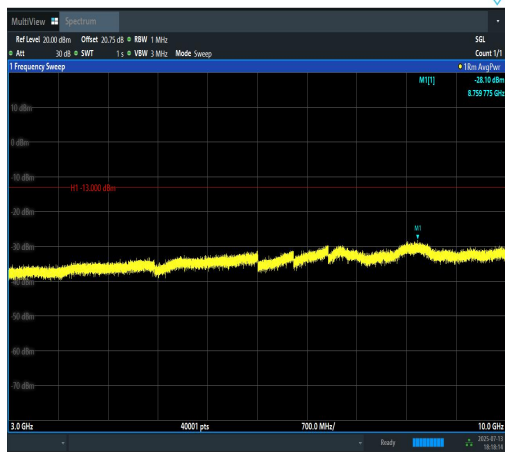
Band12-10MHz-QPSK-23060-1RB#0-3000~100 00-PASS
