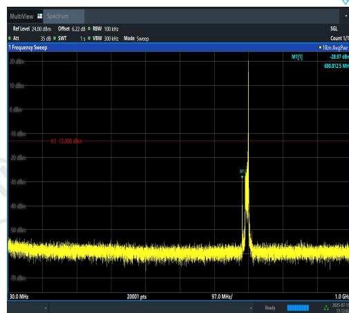
Band12-10MHz-QPSK-23060-1RB#49-30~1000- PASS
