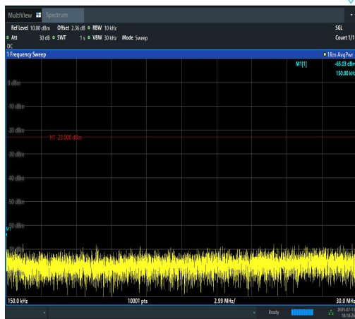
Band12-10MHz-16QAM-23060-1RB#0-0.15~30-PASS
