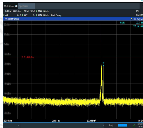
Band12-10MHz-16QAM-23060-1RB#0-30~1000-PASS
