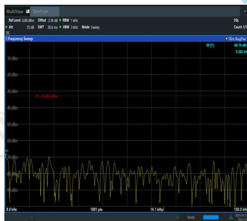
Band12-10MHz-16QAM-23060-50RB#0-0.009~0.15-PASS
