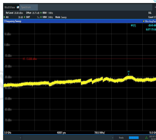
Band12-10MHz-16QAM-23060-1RB#0-3000~10000-PASS
