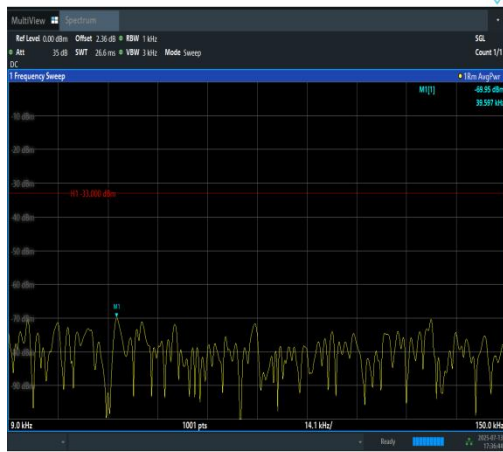
Band12-5MHz-16QAM-23155-1RB#24-0.009~0.15-PASS
