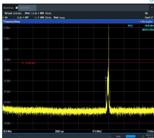
Band12-10MHz-16QAM-23060-1RB#49-30~1000-PASS
