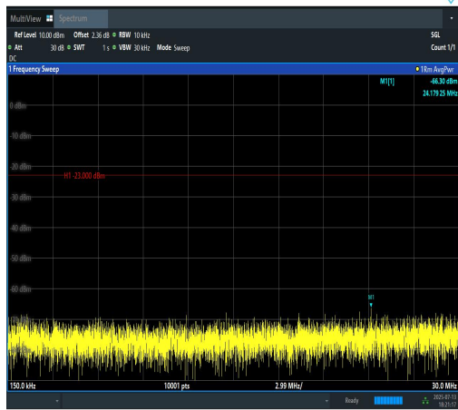
Band12-10MHz-16QAM-23060-50RB#0-0.15~30 -PASS
