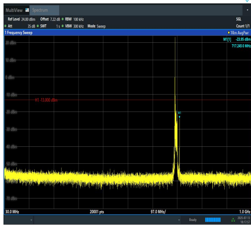
Band12-10MHz-QPSK-23060-1RB#0-30~1000-P ASS
