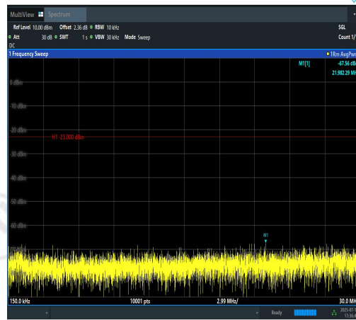
Band12-5MHz-16QAM-23155-1RB#24-0.15~30-PASS
