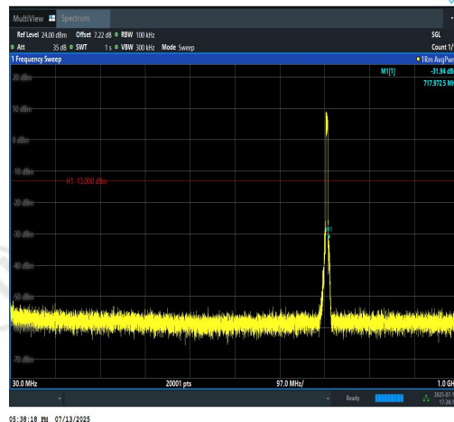
Band12-5MHz-16QAM-23155-25RB#0-30~1000- PASS
