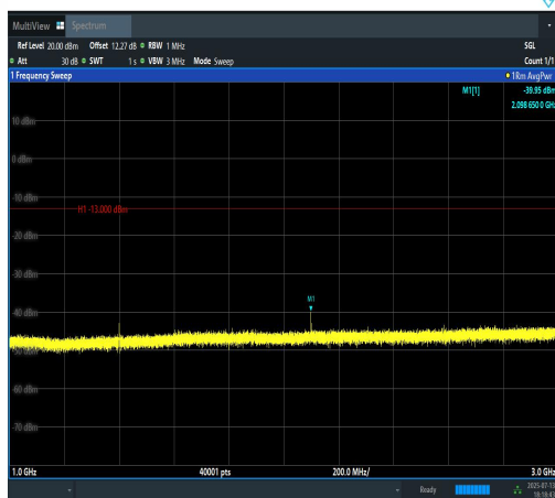
Band12-10MHz-16QAM-23060-1RB#0-1000~3000-PASS
