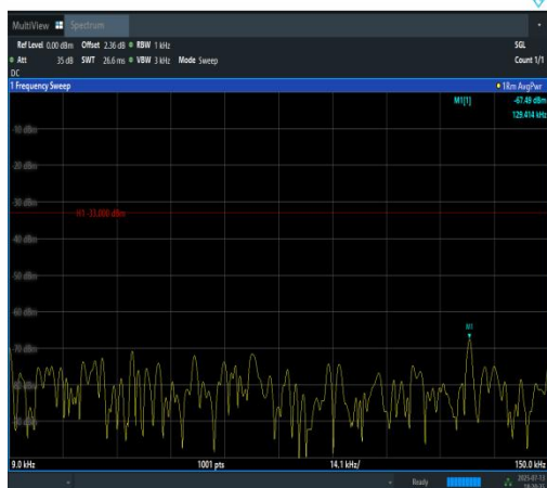
Band12-10MHz-QPSK-23060-50RB#0-0.009~0. 15-PASS
