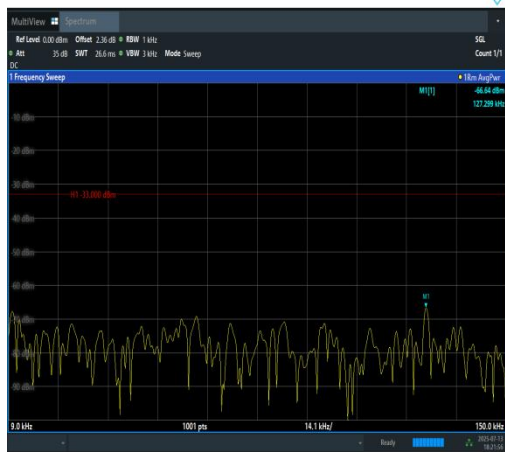
Band12-10MHz-QPSK-23095-1RB#0-0.009~0.1 5-PASS
