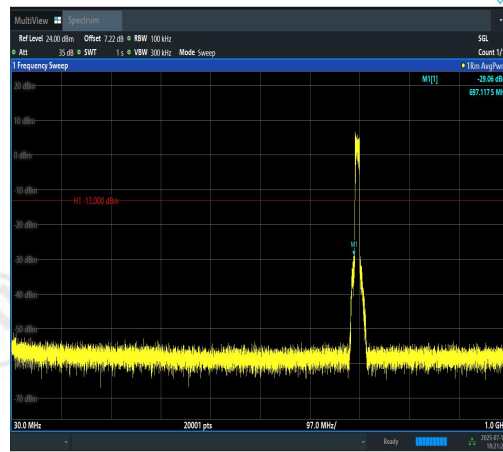
Band12-10MHz-16QAM-23060-50RB#0-30~100 0-PASS
