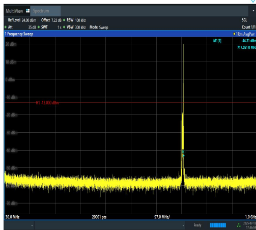
Band12-5MHz-16QAM-23155-1RB#24-30~1000-PASS
