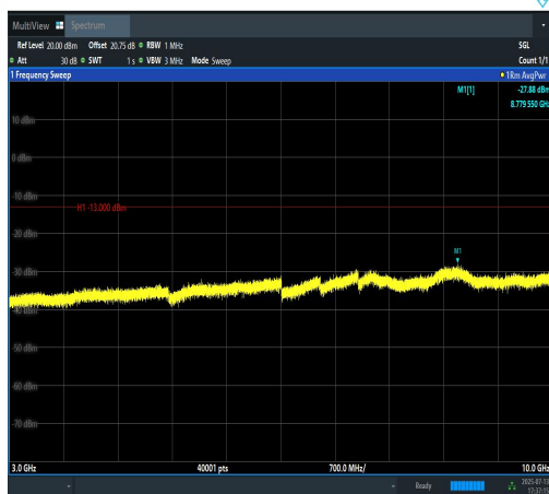
Band12-5MHz-16QAM-23155-1RB#24-3000~10000-PASS
