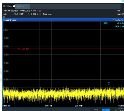
Band12-10MHz-16QAM-23060-1RB#49-0.15~30-PASS
