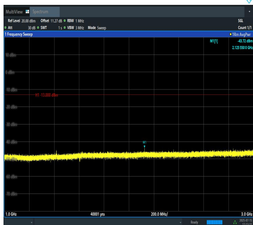
Band12-10MHz-QPSK-23060-1RB#49-1000~30 00-PASS
