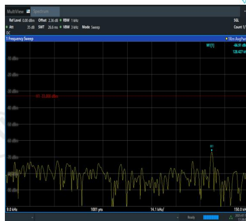
Band12-5MHz-16QAM-23155-25RB#0-0.009~0.15-PASS
