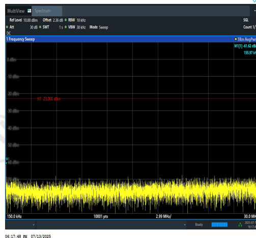
Band12-10MHz-QPSK-23060-1RB#0-0.15~30-P ASS
