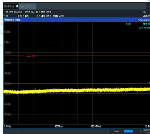
Band12-5MHz-16QAM-23155-1RB#24-1000~3000-PASS
