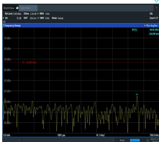
Band12-10MHz-16QAM-23060-1RB#49-0.009~0.15-PASS
