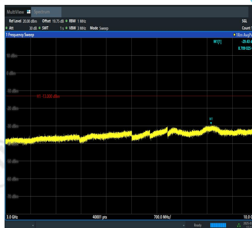
Band12-10MHz-QPSK-23060-1RB#49-3000~10 000-PASS
