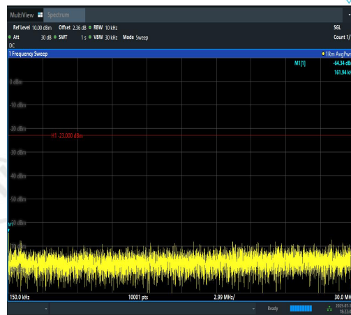
Band12-10MHz-QPSK-23095-1RB#0-0.15~30-P ASS
