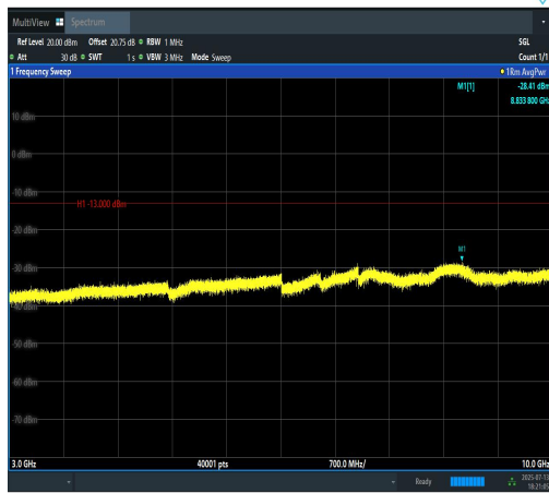
Band12-10MHz-QPSK-23060-50RB#0-3000~10000-PASS
