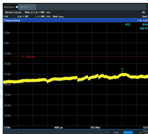
Band12-5MHz-QPSK-23155-1RB#24-3000~100 00-PASS
