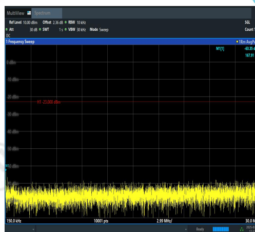
Band12-5MHz-16QAM-23095-1RB#24-0.15~30-PASS
