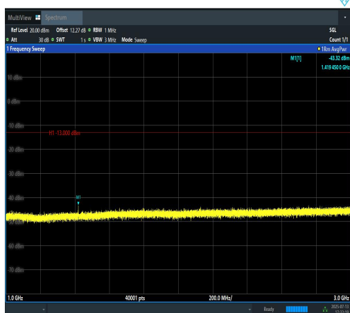
Band12-5MHz-QPSK-23095-1RB#24-1000~300 0-PASS
