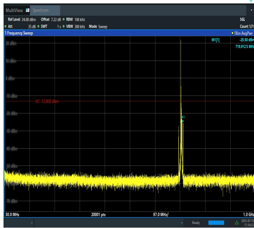
Band12-5MHz-QPSK-23155-1RB#0-30~1000-P ASS
