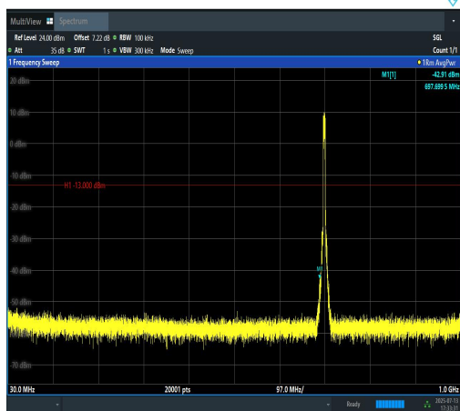
Band12-5MHz-QPSK-23095-25RB#0-30~1000-P ASS
