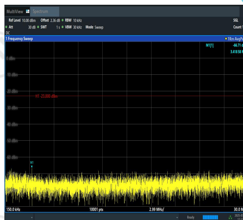
Band12-5MHz-QPSK-23155-25RB#0-0.15~30-P ASS
