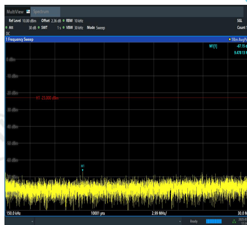
Band12-5MHz-QPSK-23155-1RB#0-0.15~30-PA SS
