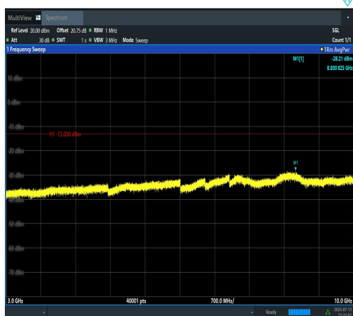
Band12-5MHz-QPSK-23095-25RB#0-3000~100 00-PASS
