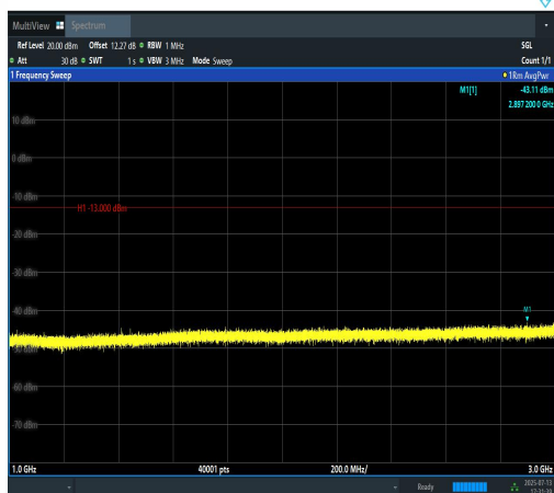
Band12-5MHz-16QAM-23095-1RB#0-1000~300 0-PASS
