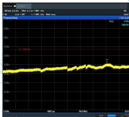
Band12-5MHz-16QAM-23095-1RB#0-3000~100 00-PASS
