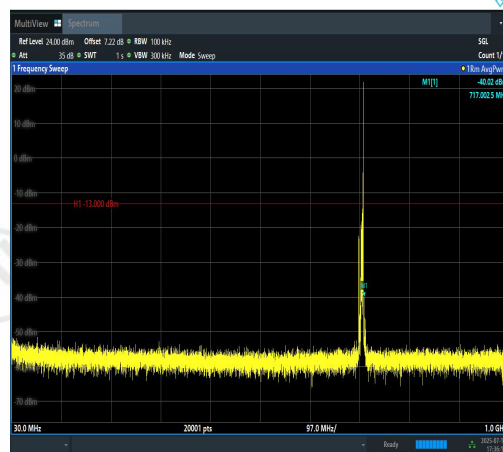
Band12-5MHz-QPSK-23155-1RB#24-30~1000-P ASS
