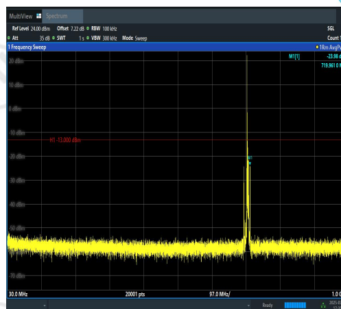
Band12-5MHz-16QAM-23155-1RB#0-30~1000-P ASS
