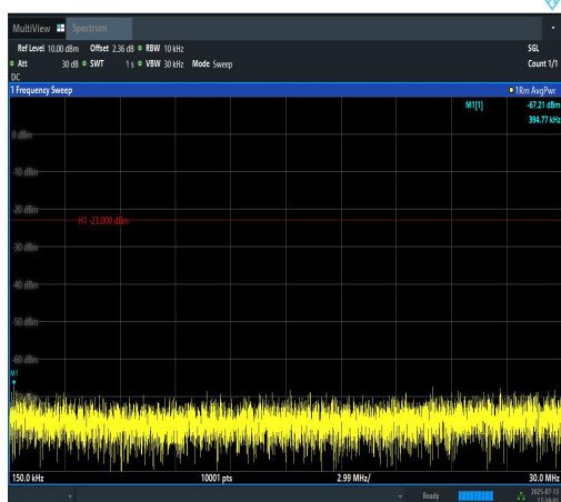
Band12-5MHz-16QAM-23095-25RB#0-0.15~30- PASS
