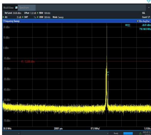
Band12-5MHz-16QAM-23095-1RB#24-30~1000-PASS
