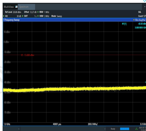
Band12-5MHz-QPSK-23095-25RB#0-1000~300 0-PASS
