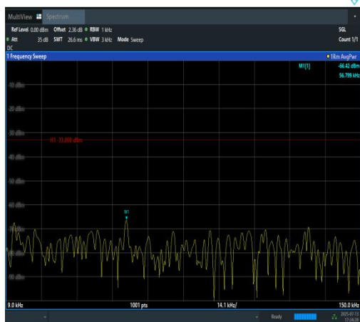
Band12-5MHz-QPSK-23155-1RB#0-0.009~0.15- PASS
