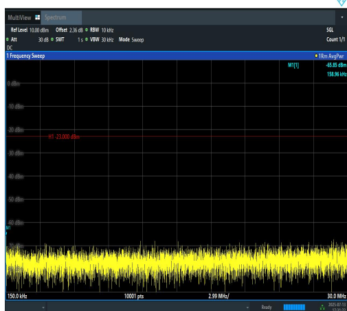
Band12-5MHz-16QAM-23095-1RB#0-0.15~30-P ASS
