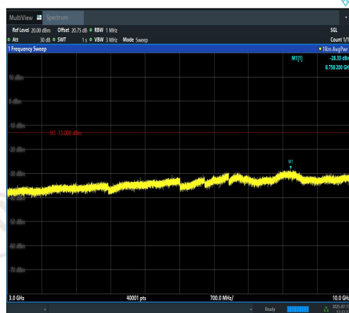
Band12-5MHz-QPSK-23095-1RB#24-3000~100 00-PASS
