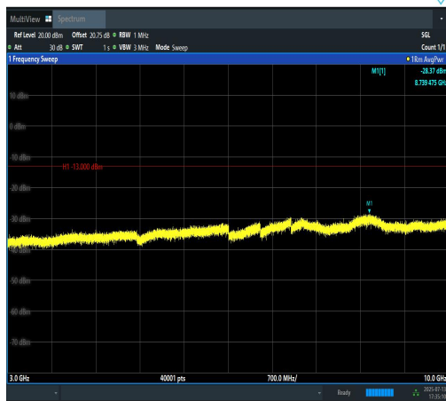
Band12-5MHz-QPSK-23155-1RB#0-3000~1000 0-PASS
