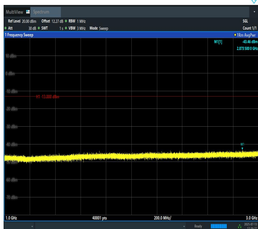
Band12-5MHz-QPSK-23155-1RB#24-1000~300 0-PASS
