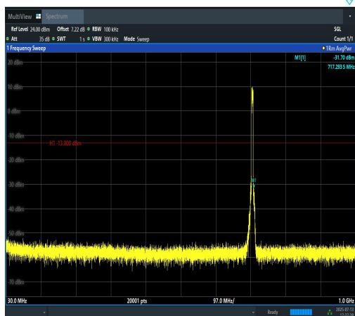
Band12-5MHz-QPSK-23155-25RB#0-30~1000-P ASS
