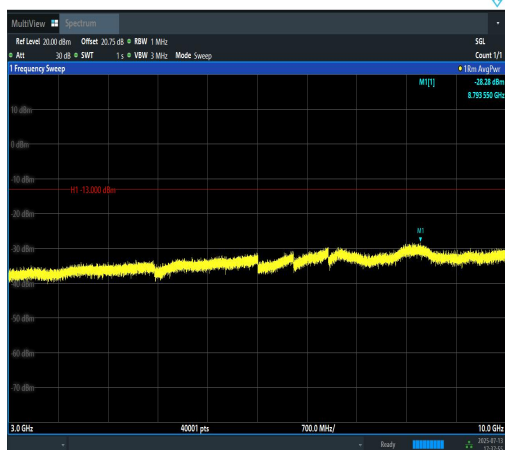
Band12-5MHz-QPSK-23155-25RB#0-3000~100 00-PASS
