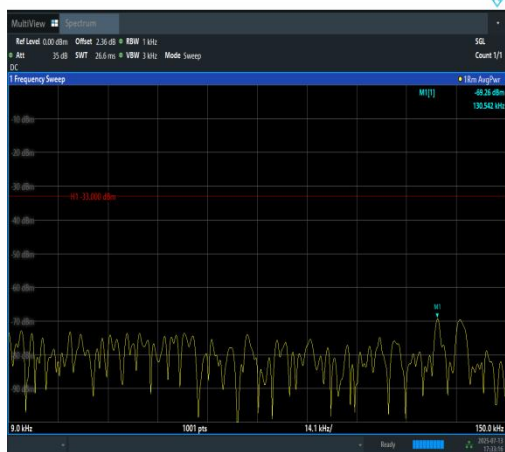
Band12-5MHz-QPSK-23095-25RB#0-0.009~0.1 5-PASS
