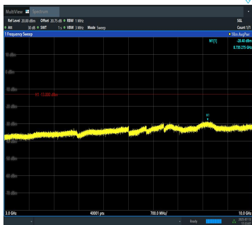
Band12-5MHz-16QAM-23095-1RB#24-3000~10000-PASS
