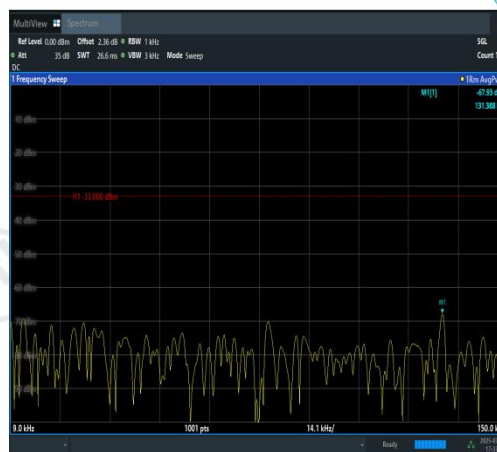
Band12-5MHz-16QAM-23095-25RB#0-0.009~0.15-PASS
