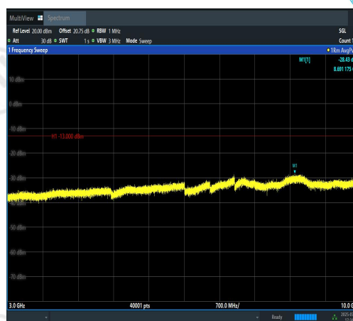
Band12-5MHz-16QAM-23095-25RB#0-3000~10 000-PASS
