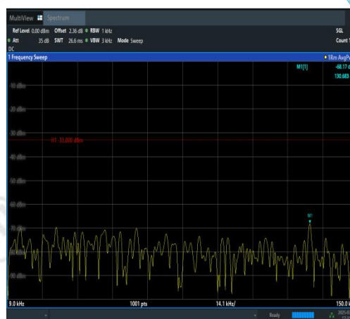
Band12-5MHz-16QAM-23095-1RB#0-0.009~0.1 5-PASS
