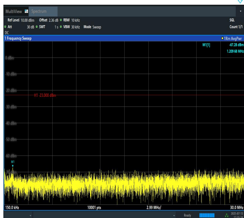
Band12-5MHz-16QAM-23155-1RB#0-0.15~30-P ASS
