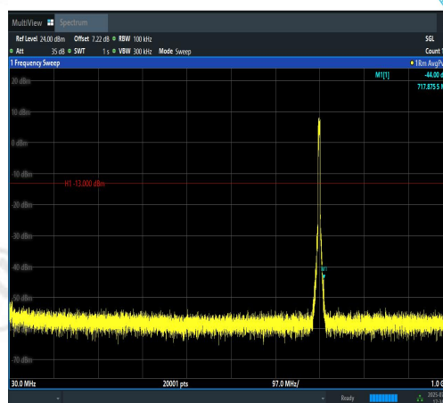
Band12-5MHz-16QAM-23095-25RB#0-30~1000- PASS
