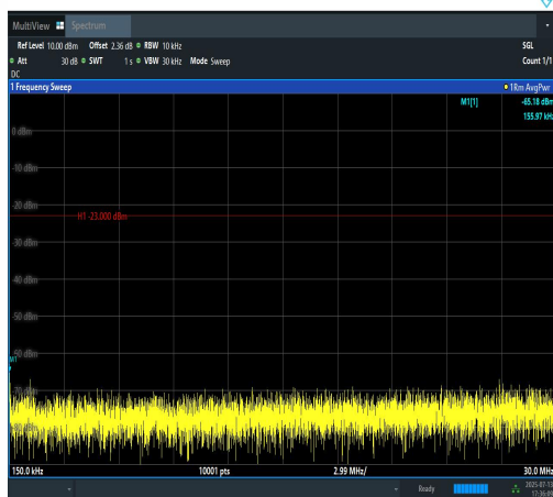
Band12-5MHz-QPSK-23155-1RB#24-0.15~30-P ASS
