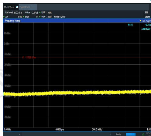
Band12-5MHz-QPSK-23155-25RB#0-1000~300 0-PASS
