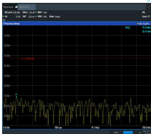
Band12-5MHz-QPSK-23155-25RB#0-0.009~0.1 5-PASS
