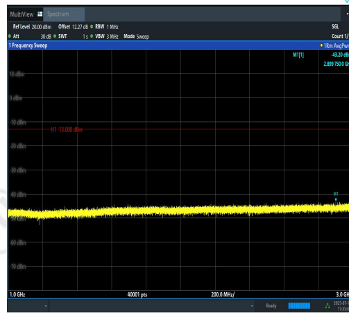
Band12-5MHz-QPSK-23155-1RB#0-1000~3000-P PASS
