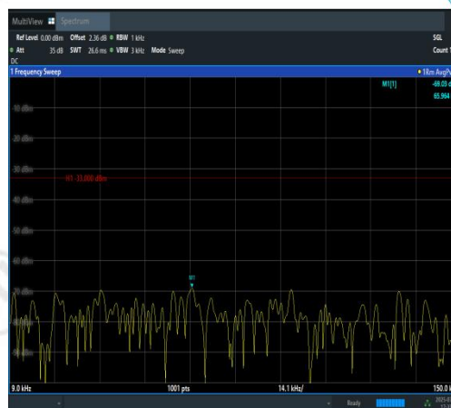
Band12-5MHz-16QAM-23155-1RB#0-0.009~0.1 5-PASS
