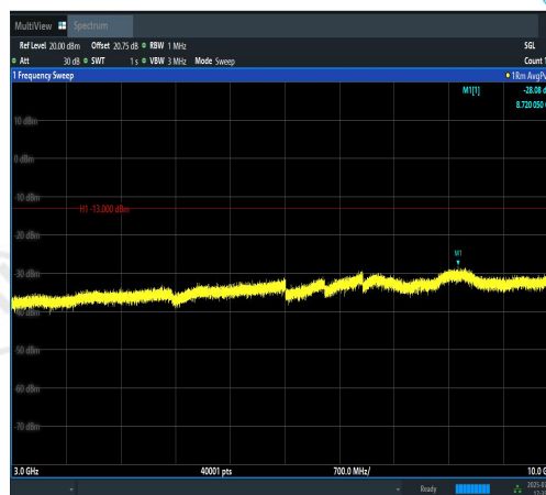
Band12-5MHz-16QAM-23155-1RB#0-3000~100 00-PASS
