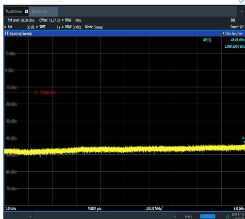
Band12-5MHz-16QAM-23155-1RB#0-1000~300 0-PASS
