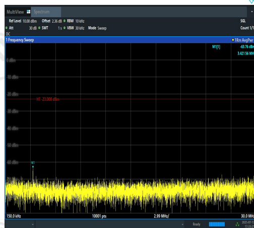
Band12-5MHz-QPSK-23095-25RB#0-0.15~30-P ASS
