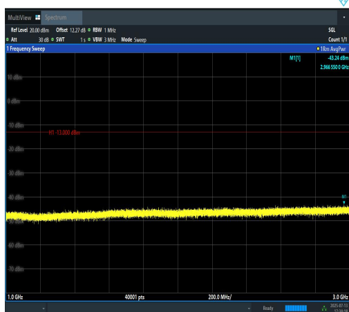
Band12-5MHz-16QAM-23095-25RB#0-1000~30 00-PASS
