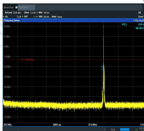
Band12-5MHz-16QAM-23095-1RB#0-30~1000-P ASS
