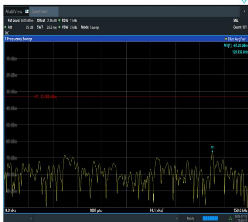
Band12-5MHz-QPSK-23035-1RB#0-0.009~0.15- PASS
