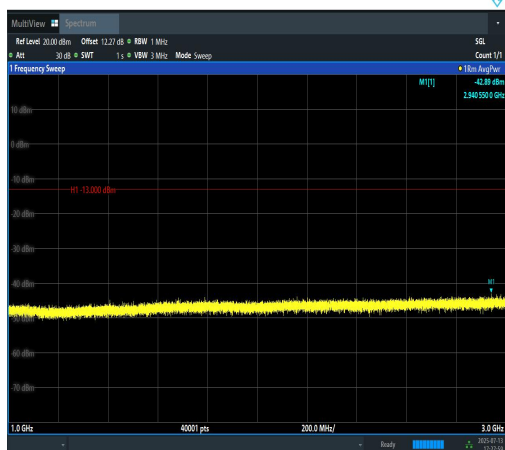
Band12-5MHz-QPSK-23035-1RB#24-1000~300 0-PASS
