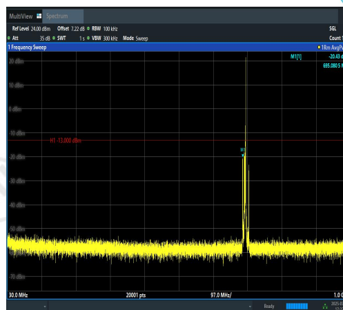
Band12-5MHz-QPSK-23035-1RB#24-30~1000-P ASS
