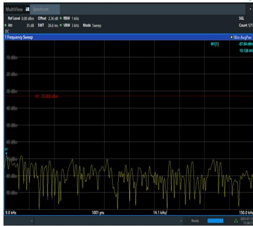
Band12-5MHz-16QAM-23035-1RB#24-0.009~0. 15-PASS
