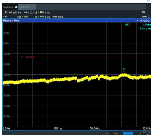
Band12-5MHz-QPSK-23035-1RB#0-3000~1000 0-PASS
