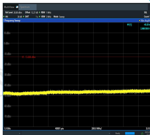
Band12-5MHz-QPSK-23035-25RB#0-1000~300 0-PASS
