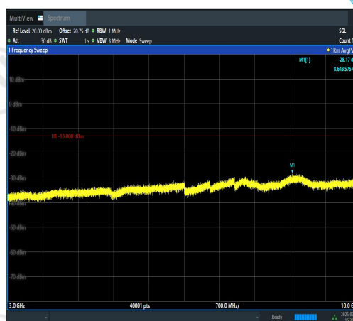
Band12-3MHz-16QAM-23165-15RB#0-3000~10 000-PASS
