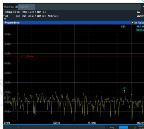
Band12-5MHz-16QAM-23035-1RB#0-0.009~0.1 5-PASS
