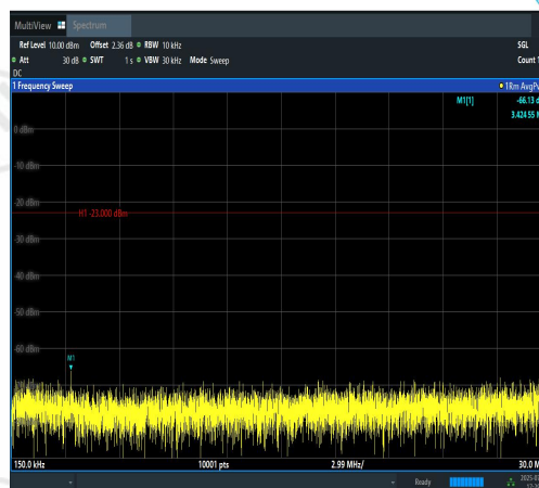
Band12-5MHz-QPSK-23035-25RB#0-0.15~30-P ASS
