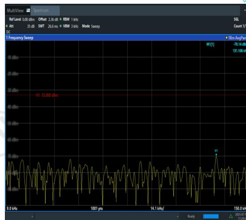
Band12-5MHz-16QAM-23035-25RB#0-0.009~0. 15-PASS
