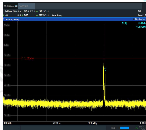
Band12-5MHz-QPSK-23095-1RB#24-30~1000-P ASS
