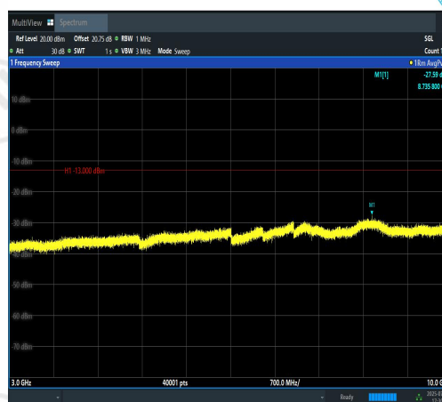
Band12-5MHz-16QAM-23035-25RB#0-3000~10 000-PASS
