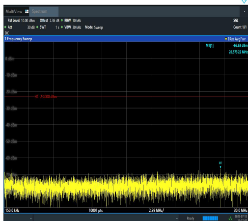
Band12-5MHz-QPSK-23035-1RB#24-0.15~30-P ASS
