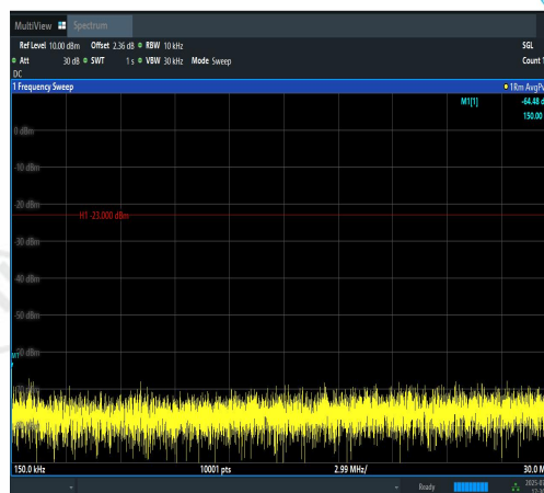
Band12-5MHz-QPSK-23095-1RB#0-0.15~30-PA SS
