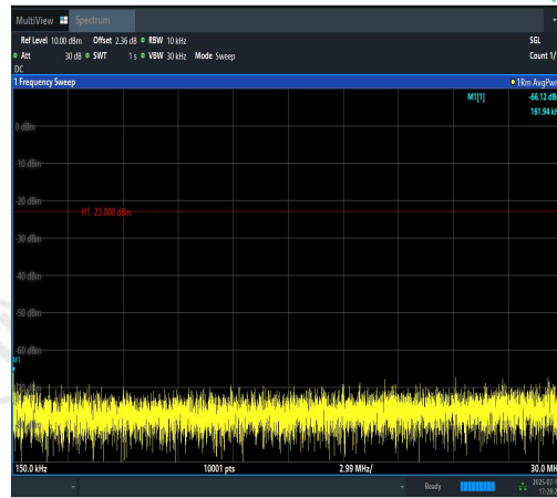
Band12-5MHz-16QAM-23035-1RB#24-0.15~30- PASS
