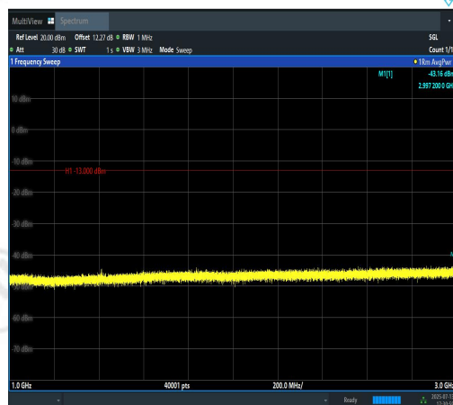
Band12-5MHz-QPSK-23095-1RB#0-1000~3000-PASS
