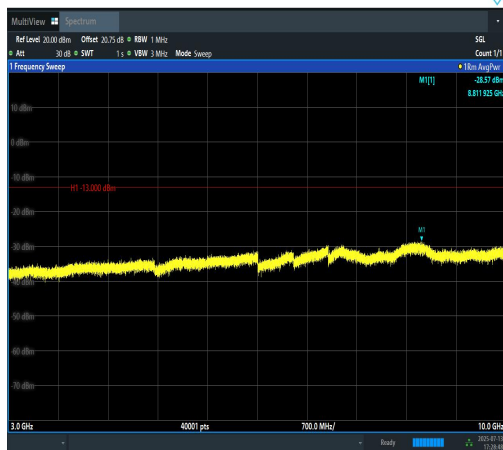
Band12-5MHz-16QAM-23035-1RB#24-3000~10000- PASS
