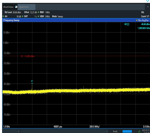
Band12-5MHz-16QAM-23035-1RB#0-1000~300 0-PASS
