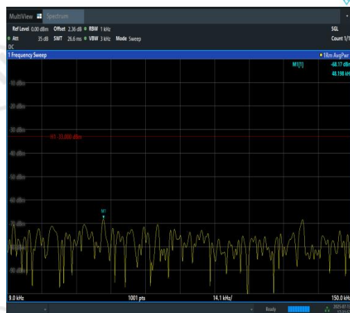
Band12-5MHz-QPSK-23095-1RB#24-0.009~0.1 5-PASS
