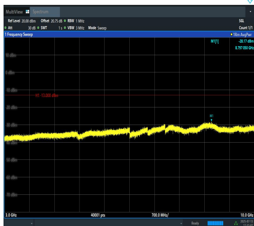
Band12-5MHz-QPSK-23095-1RB#0-3000~1000 0-PASS
