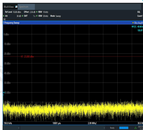
Band12-5MHz-QPSK-23035-1RB#0-0.15~30-PA SS
