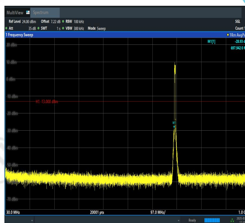
Band12-5MHz-16QAM-23035-25RB#0-30~1000- PASS
