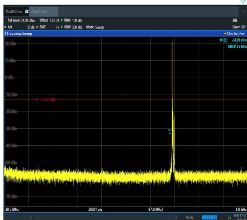
Band12-5MHz-QPSK-23035-1RB#0-30~1000-P ASS
