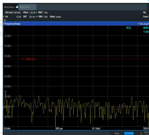
Band12-5MHz-QPSK-23035-1RB#24-0.009~0.1 5-PASS
