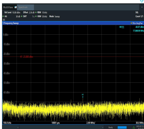
Band12-3MHz-16QAM-23165-15RB#0-0.15~30- PASS
