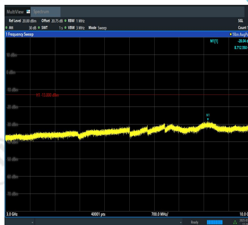
Band12-5MHz-QPSK-23035-1RB#24-3000~100 00-PASS
