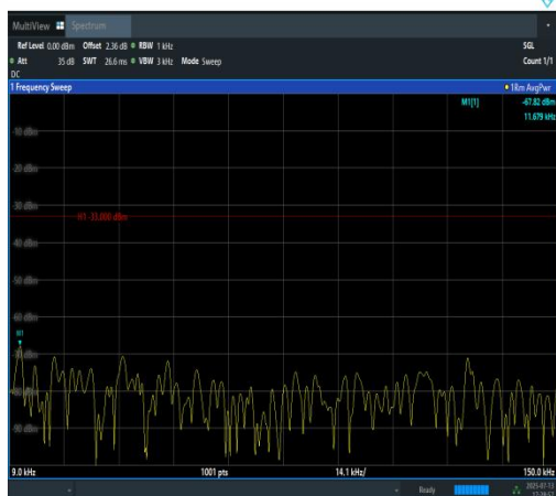
Band12-5MHz-QPSK-23035-25RB#0-0.009~0.1 5-PASS
