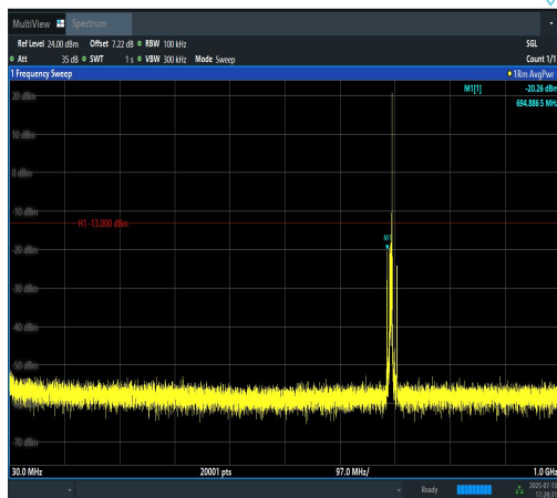
Band12-5MHz-16QAM-23035-1RB#24-30~1000- PASS
