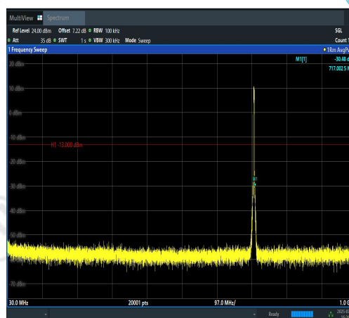
Band12-3MHz-16QAM-23165-15RB#0-30~1000- PASS
