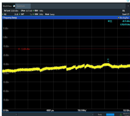
Band12-5MHz-QPSK-23035-25RB#0-3000~100 00-PASS
