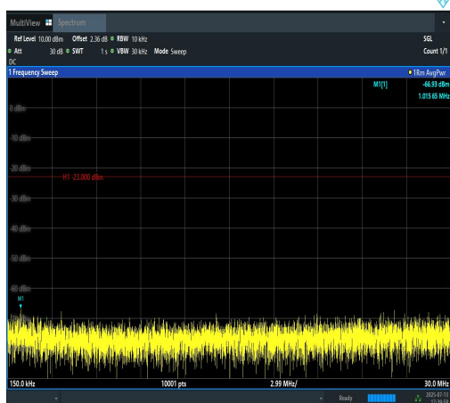
Band12-5MHz-16QAM-23035-25RB#0-0.15~30- PASS
