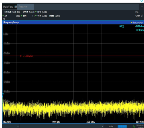
Band12-5MHz-16QAM-23035-1RB#0-0.15~30-P ASS
