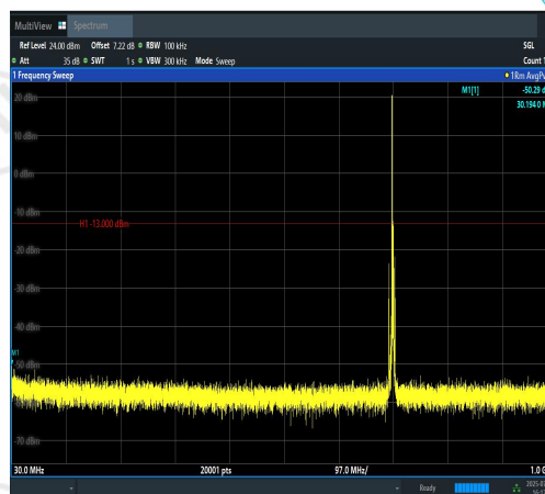
Band12-3MHz-16QAM-23095-1RB#0-30~1000-P ASS
