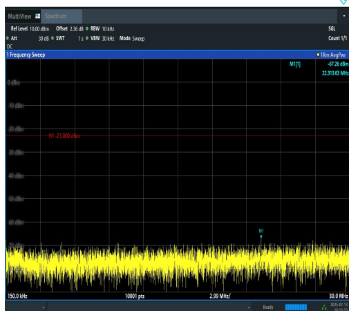
Band12-3MHz-16QAM-23095-1RB#0-0.15~30-P ASS
