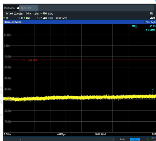
Band12-3MHz-QPSK-23165-1RB#0-1000~3000-PASS
