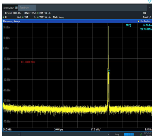
Band12-3MHz-16QAM-23165-1RB#14-30~1000-PASS
