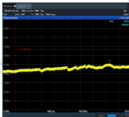
Band12-3MHz-16QAM-23095-1RB#0-3000~100 00-PASS
