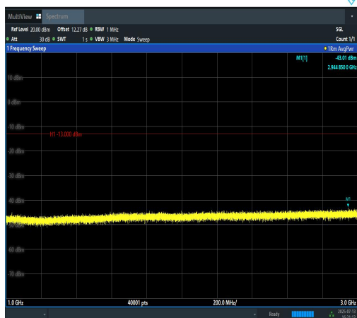
Band12-3MHz-16QAM-23165-1RB#0-1000~300 0-PASS
