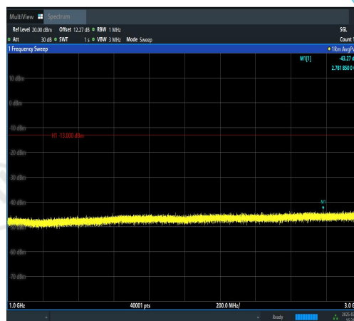
Band12-3MHz-QPSK-23165-15RB#0-1000~300 0-PASS
