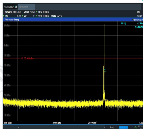
Band12-3MHz-QPSK-23165-1RB#14-30~1000-P ASS
