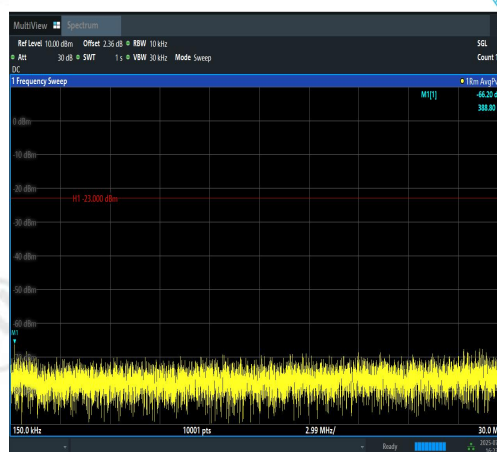
Band12-3MHz-16QAM-23165-1RB#14-0.15~30-PASS
