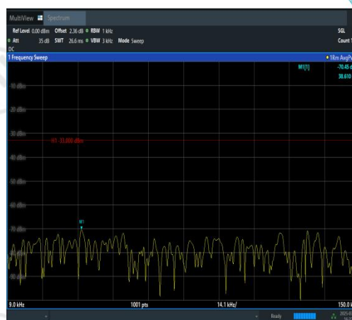
Band12-3MHz-QPSK-23165-1RB#14-0.009~0.1 5-PASS
