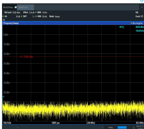
Band12-3MHz-16QAM-23165-1RB#0-0.15~30-P ASS
