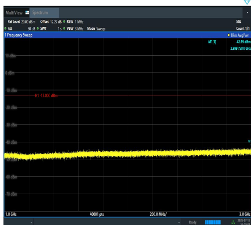
Band12-3MHz-16QAM-23095-15RB#0-1000~3000-PASS
