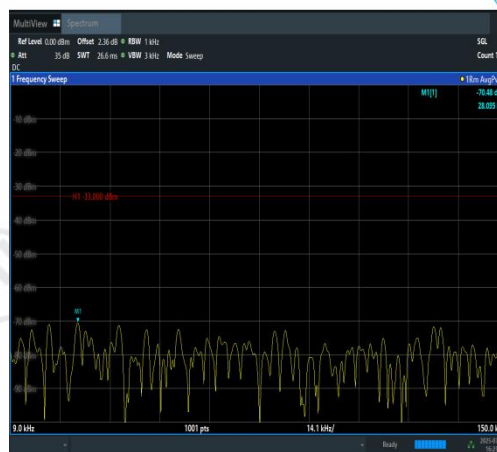
Band12-3MHz-16QAM-23165-15RB#0-0.009~0.15-PASS
