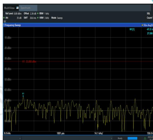
Band12-3MHz-16QAM-23165-1RB#0-0.009~0.1 5-PASS
