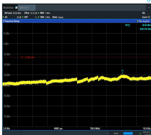
Band12-3MHz-QPSK-23165-1RB#0-3000~1000 0-PASS
