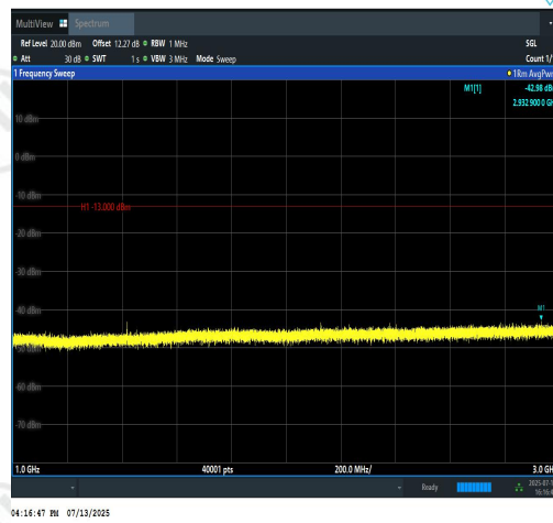
Band12-3MHz-16QAM-23095-1RB#14-1000~3000- PASS
