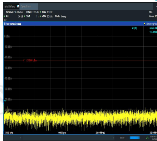
Band12-3MHz-16QAM-23095-1RB#14-0.15~30- PASS
