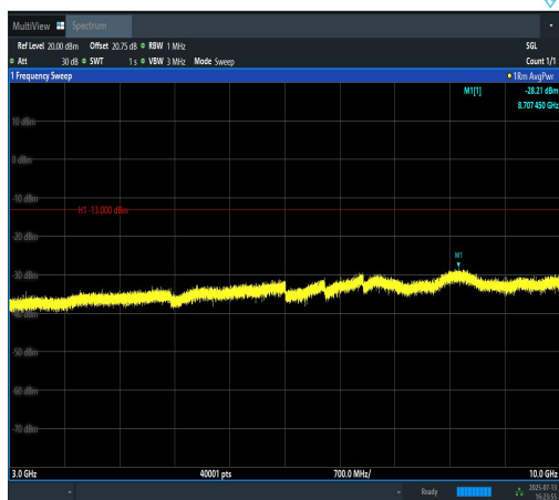
Band12-3MHz-16QAM-23165-1RB#14-3000~10000-PASS
