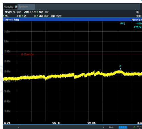
Band12-3MHz-16QAM-23165-1RB#0-3000~100 00-PASS
