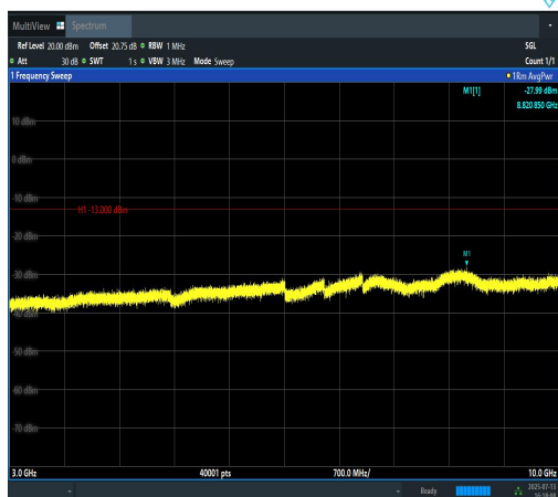
Band12-3MHz-QPSK-23095-15RB#0-3000~100 00-PASS
