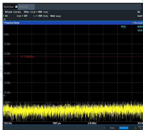
Band12-3MHz-QPSK-23165-1RB#0-0.15~30-PASS
