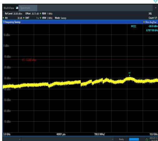
Band12-3MHz-QPSK-23165-15RB#0-3000~100 00-PASS
