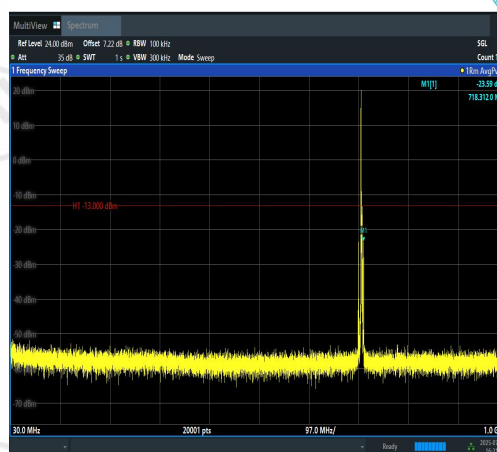
Band12-3MHz-16QAM-23165-1RB#0-30~1000-P ASS
