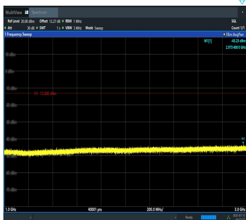
Band12-3MHz-QPSK-23165-1RB#14-1000~300 0-PASS
