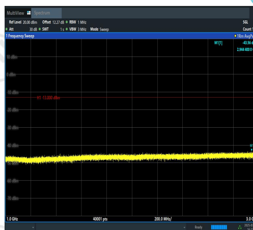
Band12-3MHz-16QAM-23165-1RB#14-1000~3000-PASS
