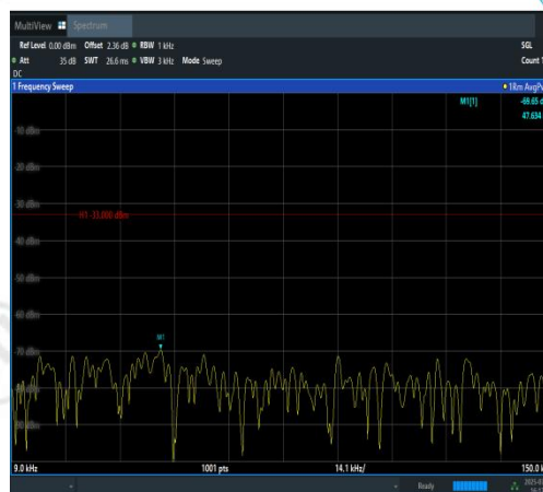
Band12-3MHz-16QAM-23095-1RB#0-0.009~0.1 5-PASS
