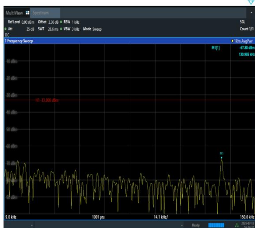
Band12-3MHz-QPSK-23165-15RB#0-0.009~0.1 5-PASS
