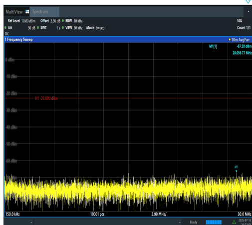
Band12-3MHz-QPSK-23165-1RB#14-0.15~30-P ASS
