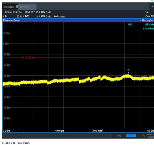
Band12-3MHz-16QAM-23095-1RB#14-3000~10000- PASS
