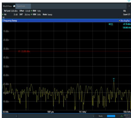
Band12-3MHz-QPSK-23165-1RB#0-0.009~0.15-PASS
