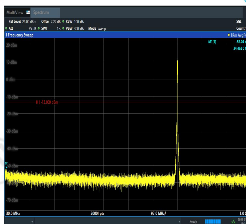
Band12-3MHz-16QAM-23095-15RB#0-30~1000-PASS
