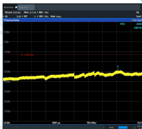
Band12-3MHz-16QAM-23095-15RB#0-3000~10000-PASS
