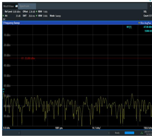
Band12-3MHz-16QAM-23095-1RB#14-0.009~0. 15-PASS
