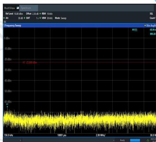
Band12-3MHz-QPSK-23165-15RB#0-0.15~30-P ASS
