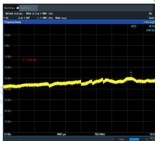
Band12-3MHz-QPSK-23165-1RB#14-3000~100 00-PASS
