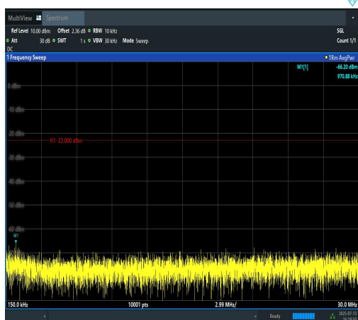
Band12-3MHz-16QAM-23095-15RB#0-0.15~30-PASS
