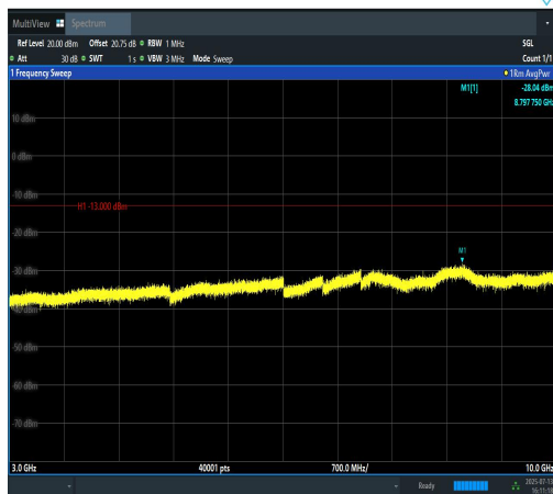
Band12-3MHz-QPSK-23095-1RB#0-3000~1000 0-PASS
