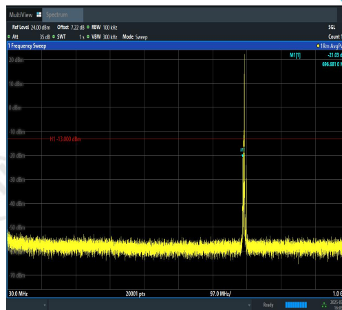
Band12-3MHz-QPSK-23025-1RB#14-30~1000-P ASS
