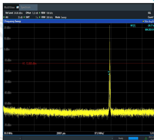
Band12-3MHz-16QAM-23025-1RB#0-30~1000-P ASS
