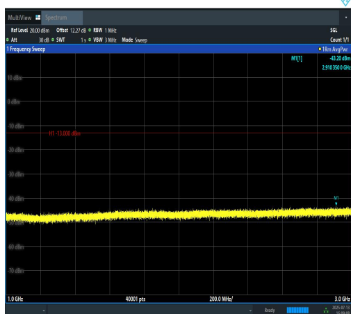
Band12-3MHz-16QAM-23025-15RB#0-1000~30 00-PASS
