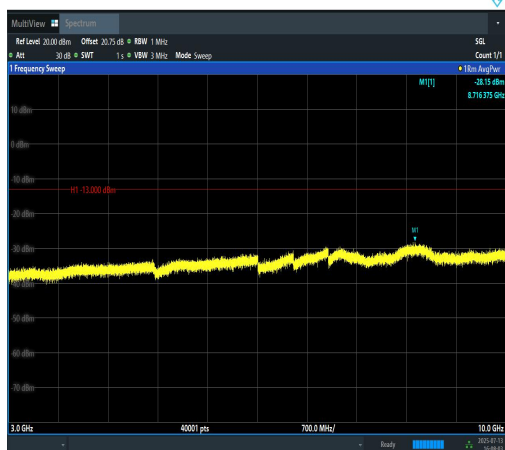
Band12-3MHz-QPSK-23025-15RB#0-3000~100 00-PASS
