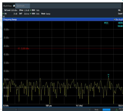
Band12-3MHz-QPSK-23025-1RB#14-0.009~0.1 5-PASS
