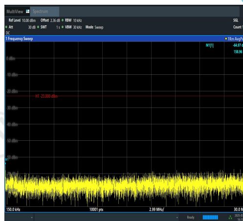
Band12-3MHz-QPSK-23095-1RB#0-0.15~30-PA SS
