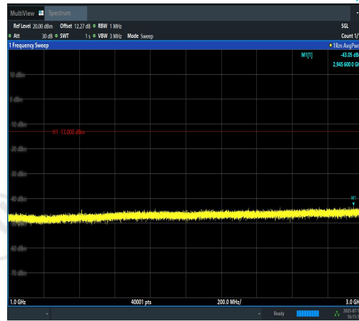
Band12-3MHz-QPSK-23095-1RB#0-1000~3000-P PASS
