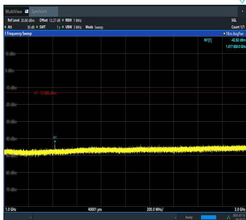
Band12-3MHz-QPSK-23095-1RB#14-1000~300 0-PASS
