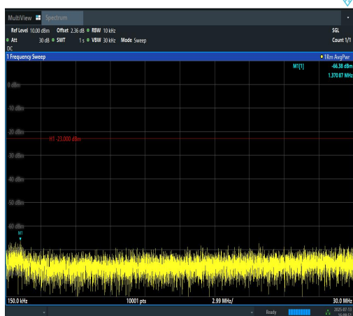
Band12-3MHz-16QAM-23025-15RB#0-0.15~30- PASS
