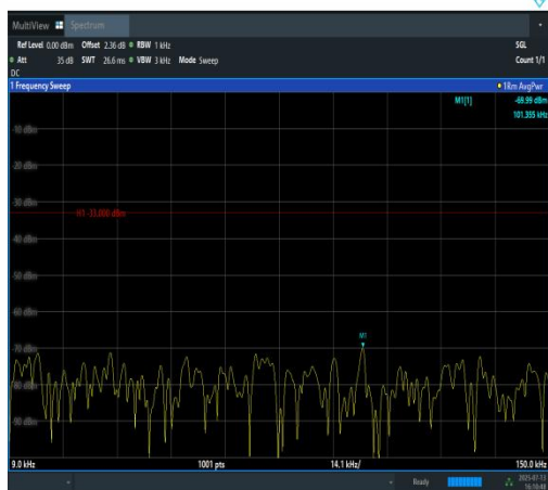
Band12-3MHz-QPSK-23095-1RB#0-0.009~0.15- PASS
