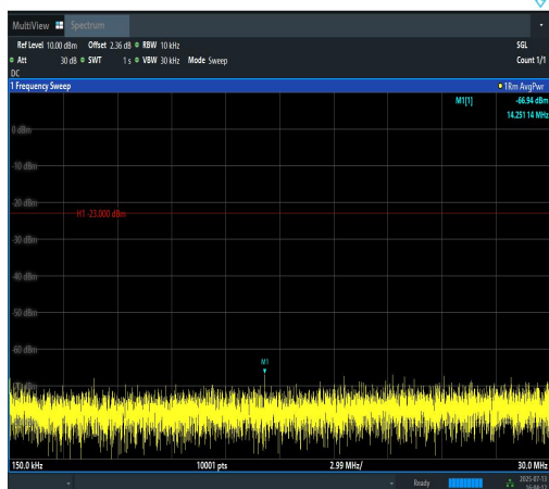
Band12-3MHz-16QAM-23025-1RB#0-0.15~30-P ASS
