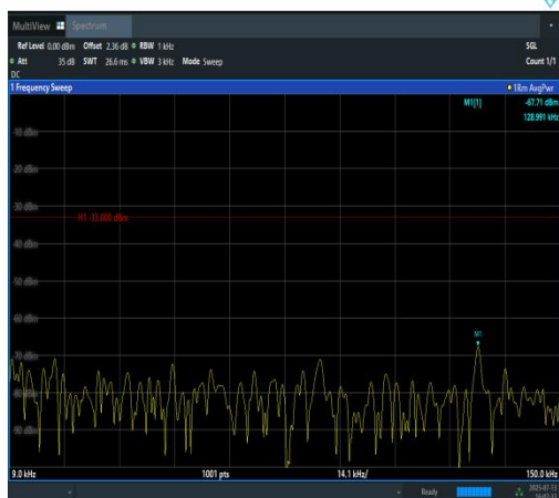
Band12-3MHz-QPSK-23025-15RB#0-0.009~0.1 5-PASS
