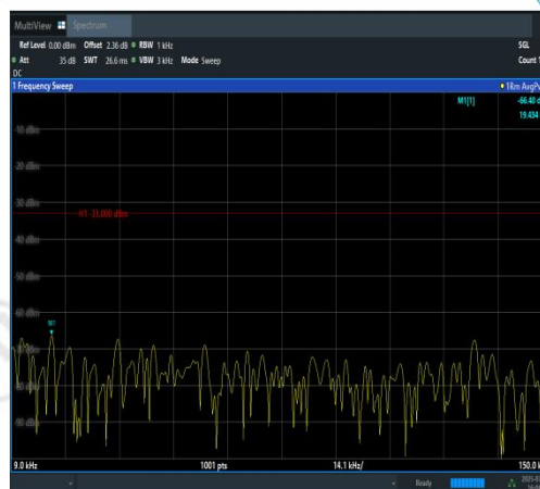
Band12-3MHz-16QAM-23025-1RB#0-0.009~0.1 5-PASS
