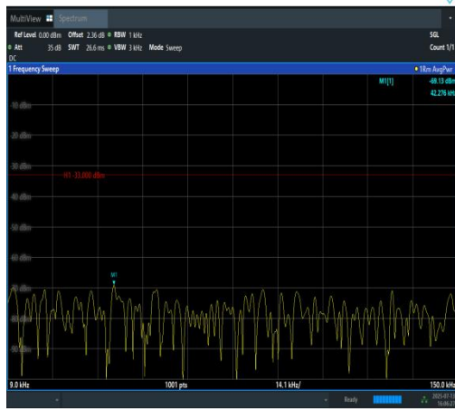
Band12-3MHz-16QAM-23025-1RB#14-0.009~0.15-PASS
