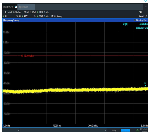
Band12-3MHz-QPSK-23025-1RB#14-1000~300 0-PASS
