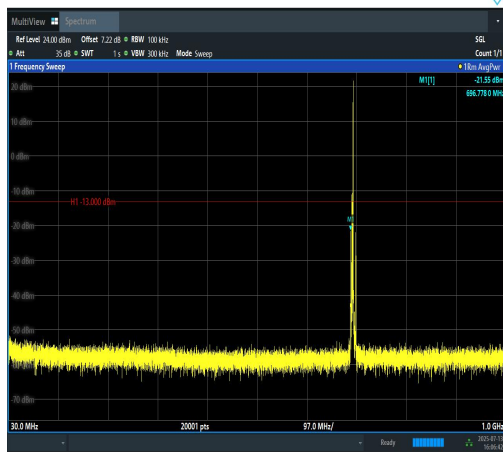
Band12-3MHz-16QAM-23025-1RB#14-30~1000-PASS
