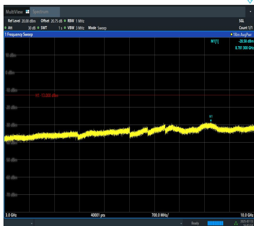
Band12-3MHz-QPSK-23025-1RB#0-3000~1000 0-PASS
