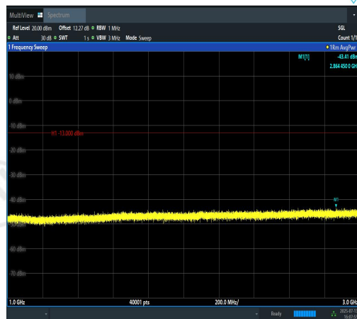
Band12-3MHz-QPSK-23025-15RB#0-1000~300 0-PASS
