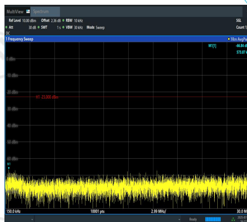
Band12-3MHz-QPSK-23095-15RB#0-0.15~30-P ASS
