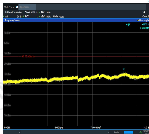
Band12-3MHz-QPSK-23095-1RB#14-3000~100 00-PASS
