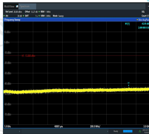
Band12-3MHz-16QAM-23025-1RB#14-1000~3000-PASS
