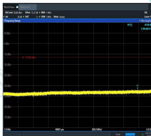
Band12-3MHz-QPSK-23095-15RB#0-1000~300 0-PASS
