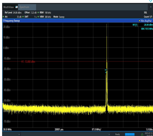
Band12-3MHz-QPSK-23025-1RB#0-30~1000-P ASS
