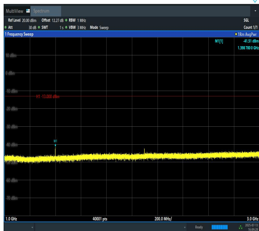
Band12-3MHz-16QAM-23025-1RB#0-1000~300 0-PASS
