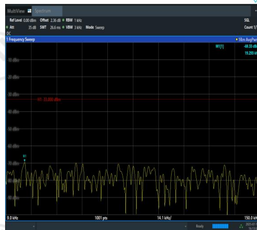
Band12-3MHz-QPSK-23095-1RB#14-0.009~0.1 5-PASS
