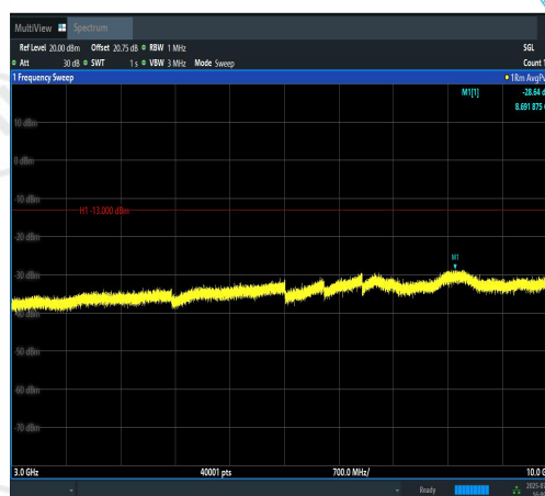
Band12-3MHz-16QAM-23025-15RB#0-3000~10 000-PASS
