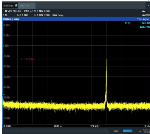
Band12-3MHz-QPSK-23095-1RB#0-30~1000-P ASS
