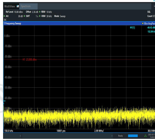
Band12-3MHz-16QAM-23025-1RB#14-0.15~30-PASS
