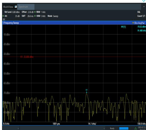
Band12-3MHz-QPSK-23095-15RB#0-0.009~0.1 5-PASS
