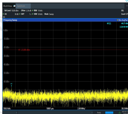
Band12-3MHz-QPSK-23025-15RB#0-0.15~30-P ASS
