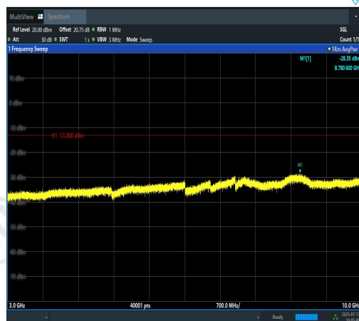
Band12-3MHz-QPSK-23025-1RB#14-3000~100 00-PASS
