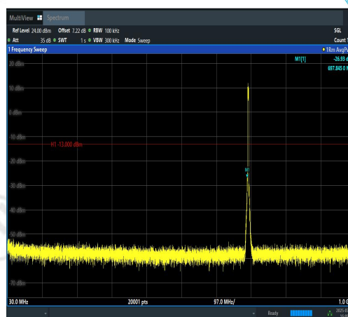
Band12-3MHz-16QAM-23025-15RB#0-30~1000- PASS
