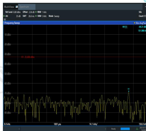
Band12-3MHz-16QAM-23025-15RB#0-0.009~0.15-PASS
