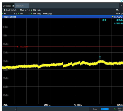
Band12-3MHz-16QAM-23025-1RB#14-3000~10000-PASS
