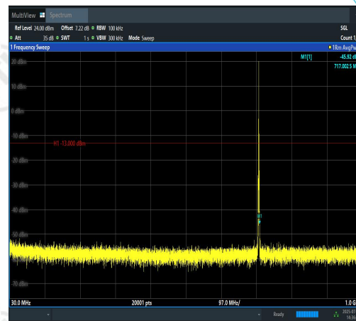
Band12-1.4MHz-16QAM-23173-1RB#0-30~1000 -PASS
