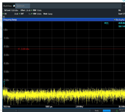
Band12-1.4MHz-QPSK-23173-6RB#0-0.15~30-P ASS
