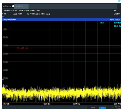
Band12-1.4MHz-16QAM-23173-6RB#0-0.15~30- PASS
