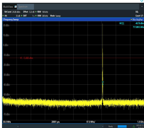
Band12-1.4MHz-QPSK-23173-1RB#0-30~1000-PASS
