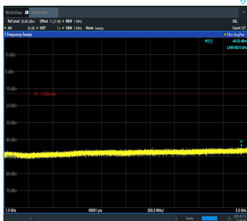
Band12-1.4MHz-16QAM-23173-6RB#0-1000~30 00-PASS
