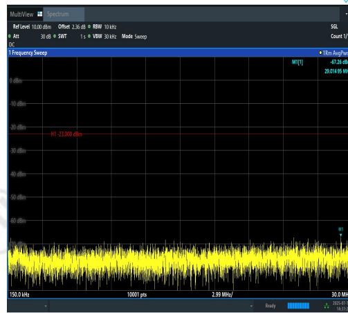
Band12-1.4MHz-16QAM-23173-1RB#5-0.15~30- PASS
