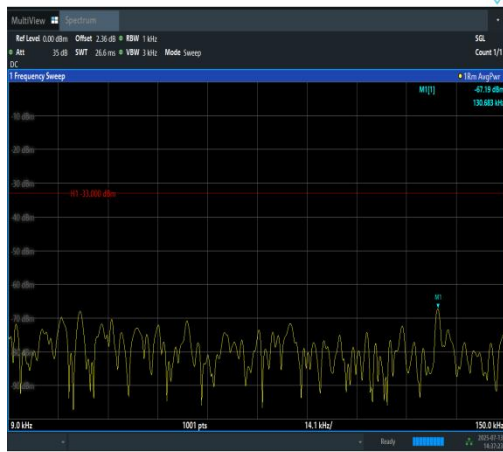
Band12-1.4MHz-16QAM-23173-1RB#5-0.009~0. 15-PASS
