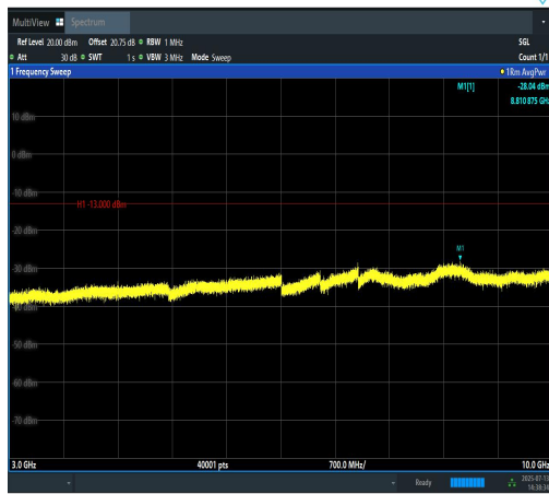
Band12-1.4MHz-QPSK-23173-6RB#0-3000~100 00-PASS
