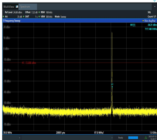
Band12-1.4MHz-QPSK-23173-6RB#0-30~1000- PASS
