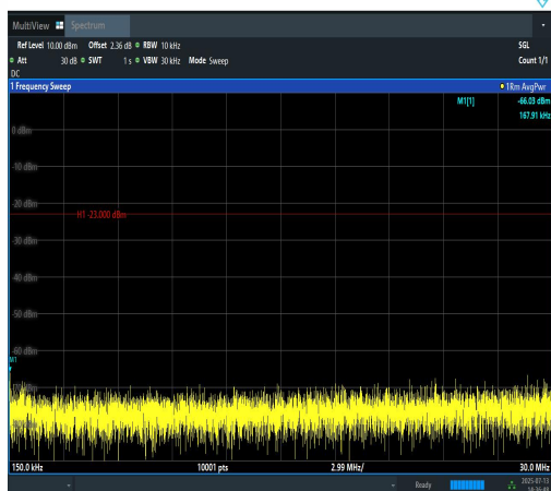
Band12-1.4MHz-QPSK-23173-1RB#5-0.15~30-PASS
