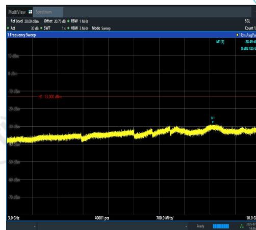
Band12-1.4MHz-16QAM-23173-1RB#0-3000~10 000-PASS
