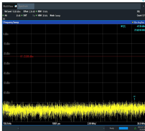
Band12-1.4MHz-16QAM-23173-1RB#0-0.15~30- PASS
