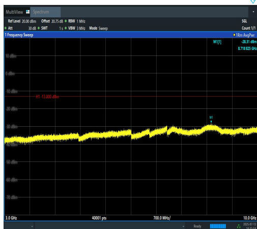
Band12-1.4MHz-QPSK-23173-1RB#0-3000~10000-PASS
