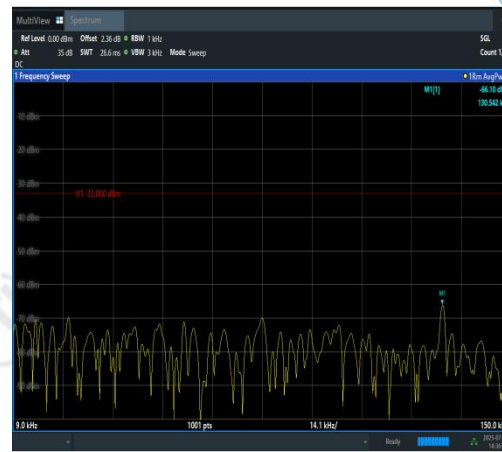
Band12-1.4MHz-16QAM-23173-1RB#0-0.009~0. 15-PASS
