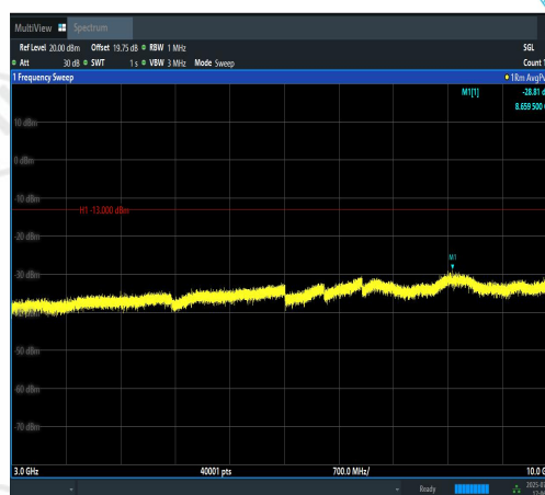
Band12-1.4MHz-16QAM-23173-6RB#0-3000~10 000-PASS
