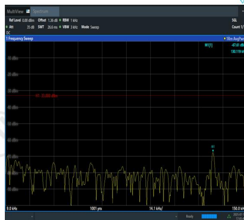
Band12-1.4MHz-16QAM-23173-6RB#0-0.009~0. 15-PASS
