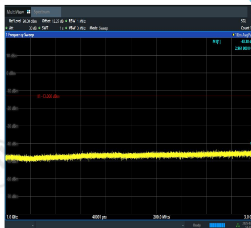
Band12-1.4MHz-QPSK-23173-1RB#0-1000~3000-PASS
