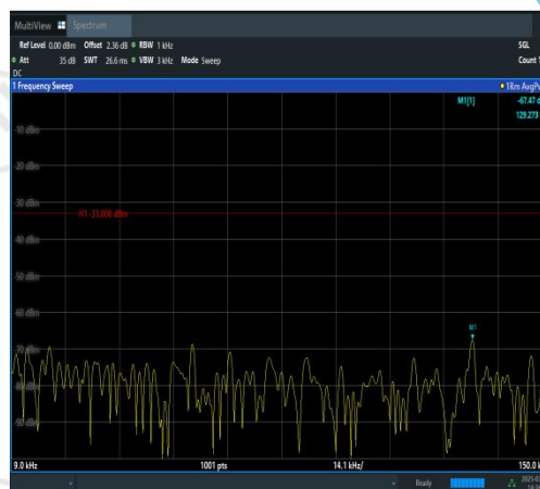
Band12-1.4MHz-QPSK-23173-1RB#5-0.009~0.15-PASS
