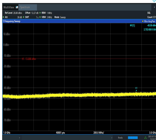
Band12-1.4MHz-16QAM-23173-1RB#0-1000~30 00-PASS
