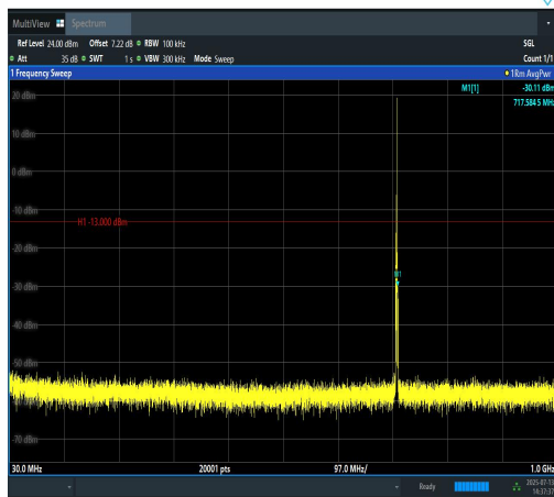
Band12-1.4MHz-16QAM-23173-1RB#5-30~1000 -PASS
