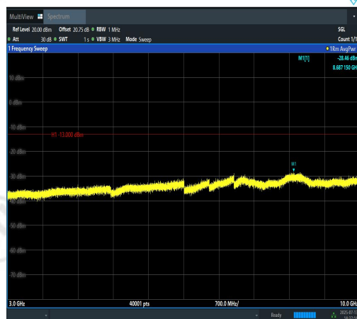
Band12-1.4MHz-QPSK-23173-1RB#5-3000~100 00-PASS
