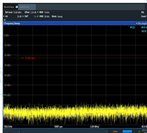
Band12-3MHz-QPSK-23025-1RB#0-0.15~30-PA SS
