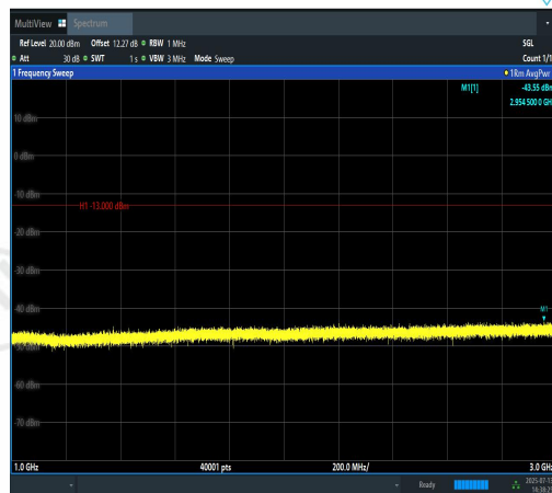
Band12-1.4MHz-QPSK-23173-6RB#0-1000~300 0-PASS
