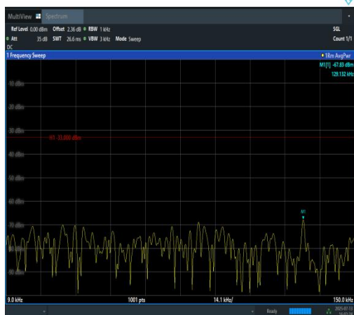
Band12-3MHz-QPSK-23025-1RB#0-0.009~0.15- PASS
