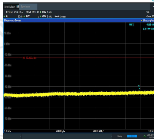
Band12-1.4MHz-16QAM-23173-1RB#5-1000~30 00-PASS
