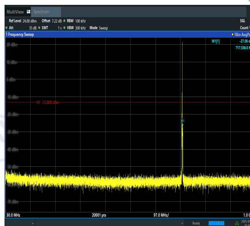
Band12-1.4MHz-QPSK-23173-1RB#5-30~1000-PASS
