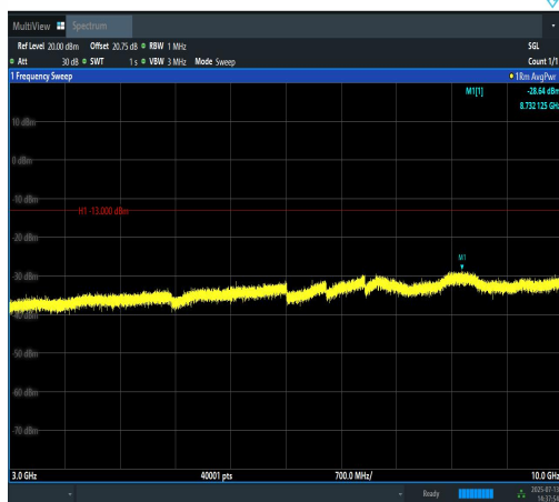
Band12-1.4MHz-16QAM-23173-1RB#5-3000~10 000-PASS
