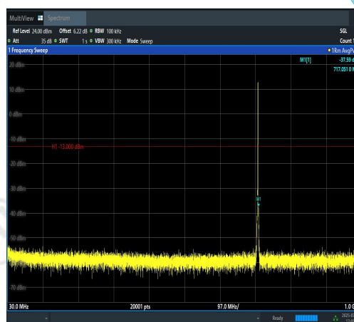
Band12-1.4MHz-16QAM-23173-6RB#0-30~1000- -PASS
