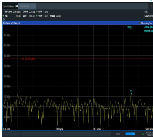
Band12-1.4MHz-16QAM-23017-1RB#5-0.009~0. 15-PASS
