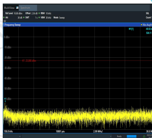
Band12-1.4MHz-QPSK-23095-6RB#0-0.15~30-P ASS
