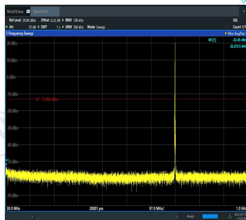
Band12-1.4MHz-QPSK-23095-1RB#5-30~1000-PASS
