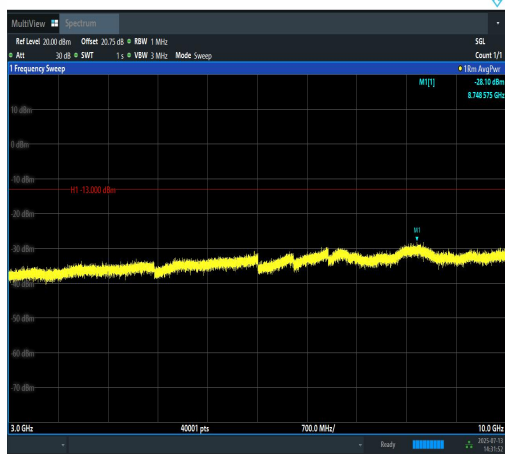
Band12-1.4MHz-QPSK-23095-1RB#0-3000~10000-PASS
