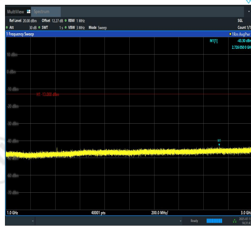
Band12-1.4MHz-QPSK-23095-1RB#0-1000~3000-PASS
