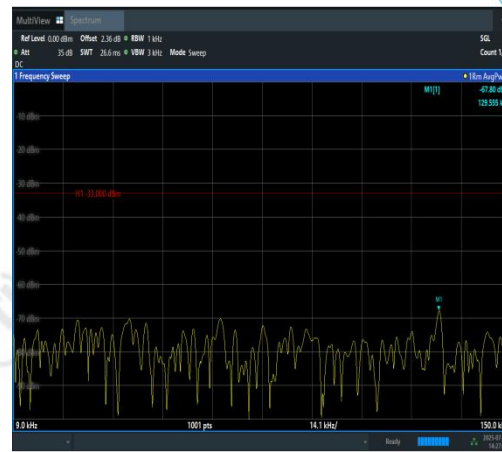
Band12-1.4MHz-16QAM-23017-1RB#0-0.009~0. 15-PASS
