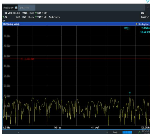
Band12-1.4MHz-QPSK-23095-6RB#0-0.009~0.1 5-PASS
