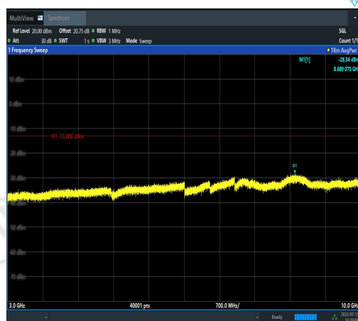
Band12-1.4MHz-QPSK-23017-1RB#5-3000~100 00-PASS
