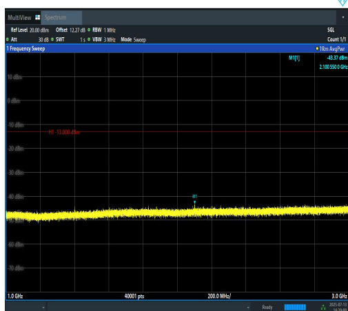
Band12-1.4MHz-QPSK-23017-1RB#5-1000~300 0-PASS
