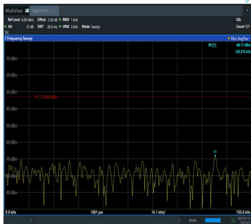
Band12-1.4MHz-QPSK-23095-1RB#0-0.009~0.1 5-PASS
