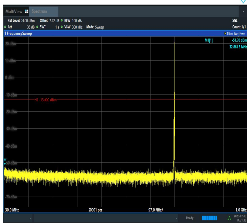
Band12-1.4MHz-QPSK-23095-1RB#0-30~1000-PASS
