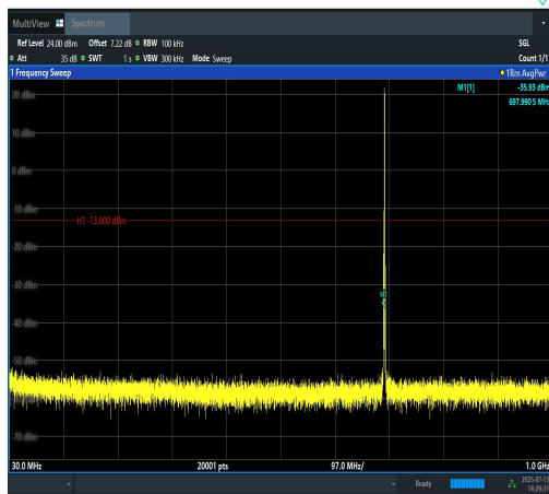
Band12-1.4MHz-16QAM-23017-1RB#5-30~1000 -PASS
