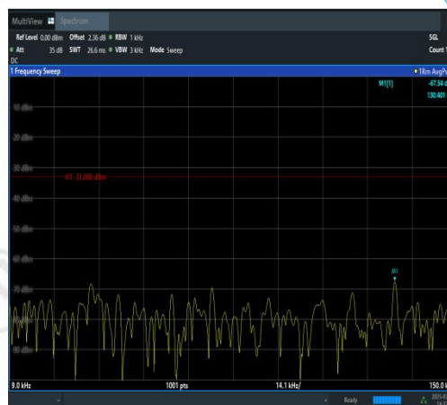
Band12-1.4MHz-16QAM-23095-1RB#0-0.009~0. 15-PASS
