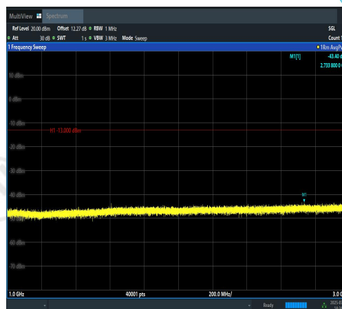
Band12-1.4MHz-QPSK-23095-6RB#0-1000~300 0-PASS
