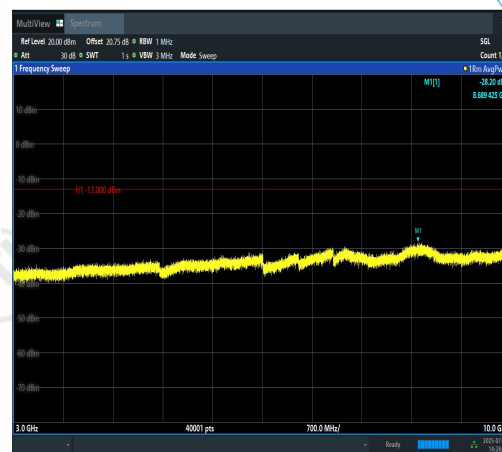
Band12-1.4MHz-16QAM-23017-1RB#0-3000~10 000-PASS
