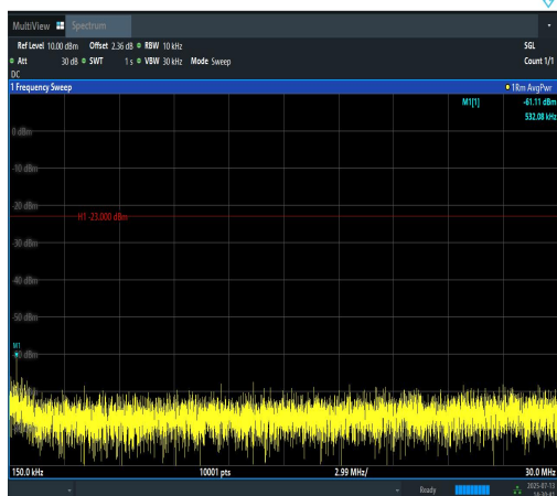
Band12-1.4MHz-16QAM-23017-6RB#0-0.15~30- PASS
