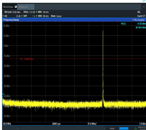
Band12-1.4MHz-QPSK-23095-6RB#0-30~1000- PASS
