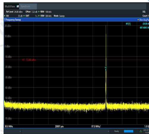
Band12-1.4MHz-16QAM-23017-1RB#0-30~1000 -PASS
