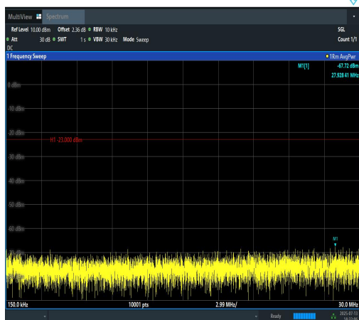
Band12-1.4MHz-16QAM-23095-1RB#0-0.15~30- PASS
