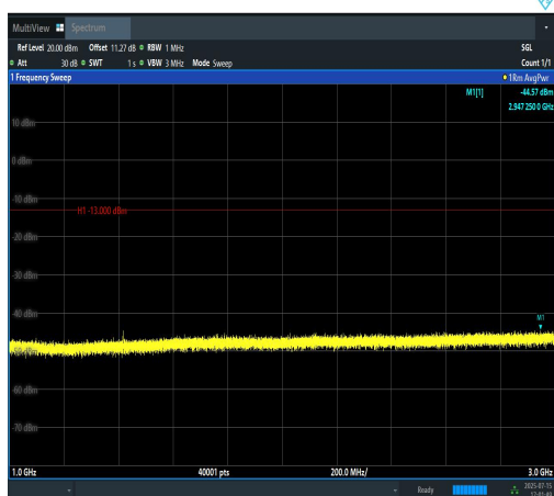
Band12-1.4MHz-QPSK-23095-1RB#5-1000~300 0-PASS
