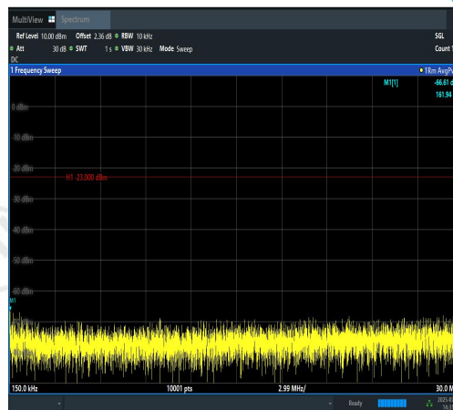
Band12-1.4MHz-QPSK-23095-1RB#0-0.15~30-P ASS
