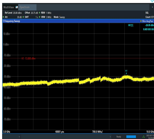
Band12-1.4MHz-16QAM-23017-1RB#5-3000~10000- 000-PASS
