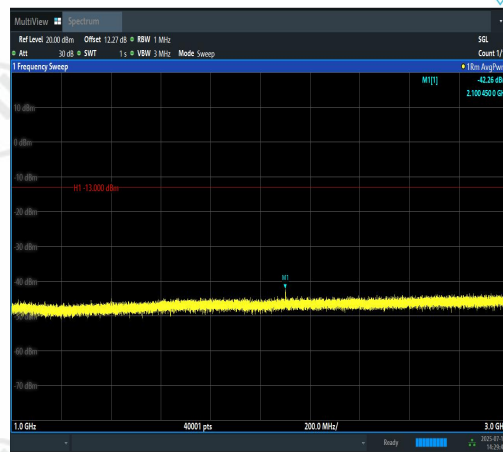
Band12-1.4MHz-16QAM-23017-1RB#5-1000~3000- 00-PASS
