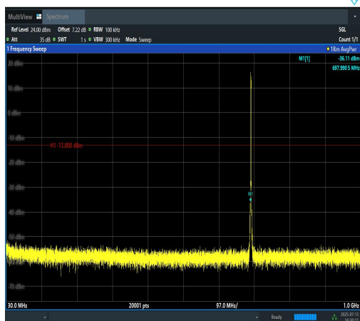
Band12-1.4MHz-QPSK-23017-6RB#0-30~1000- PASS
