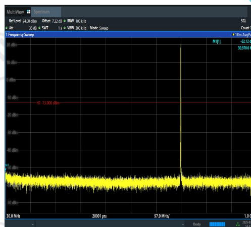
Band12-1.4MHz-16QAM-23095-1RB#0-30~1000 -PASS
