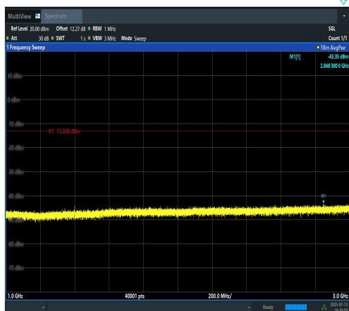
Band12-1.4MHz-16QAM-23017-6RB#0-1000~30 00-PASS
