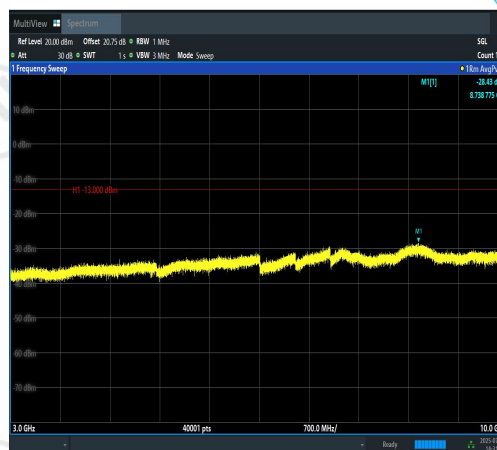
Band12-1.4MHz-16QAM-23017-6RB#0-3000~10 000-PASS
