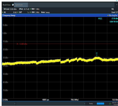
Band12-1.4MHz-QPSK-23017-6RB#0-3000~100 00-PASS
