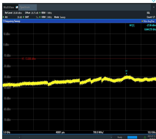
Band12-1.4MHz-QPSK-23095-6RB#0-3000~100 00-PASS
