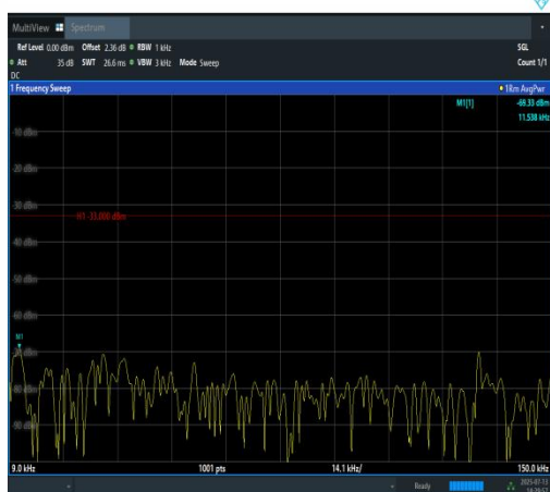
Band12-1.4MHz-QPSK-23017-6RB#0-0.009~0.1 5-PASS
