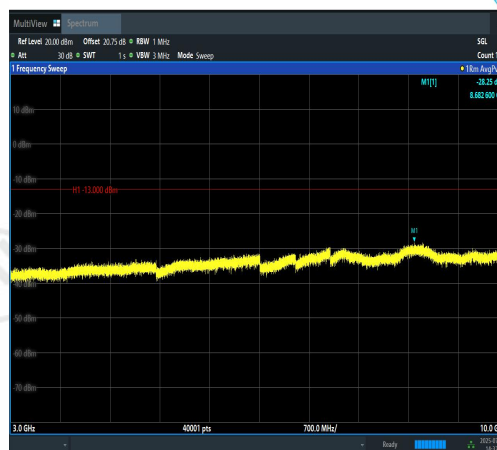
Band12-1.4MHz-16QAM-23095-1RB#0-3000~10 000-PASS
