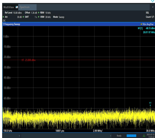
Band12-1.4MHz-QPSK-23095-1RB#5-0.15~30-PASS
