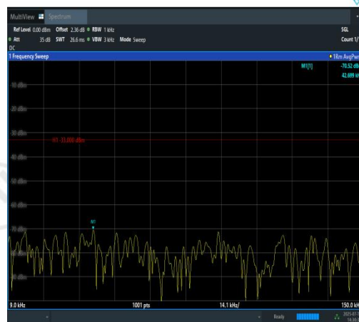
Band12-1.4MHz-16QAM-23017-6RB#0-0.009~0. 15-PASS
