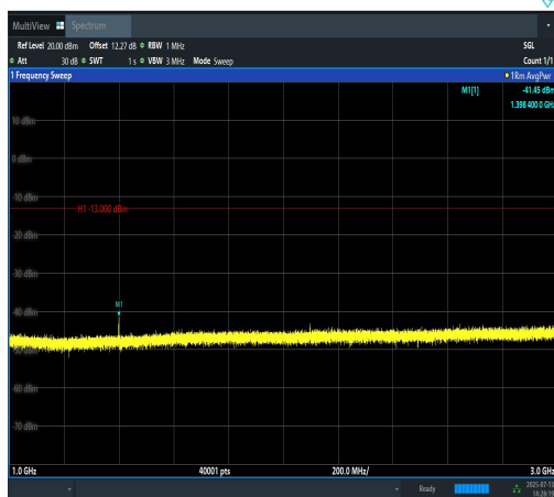
Band12-1.4MHz-16QAM-23017-1RB#0-1000~30 00-PASS
