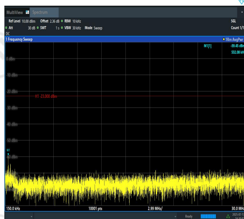
Band12-1.4MHz-QPSK-23017-6RB#0-0.15~30-P ASS
