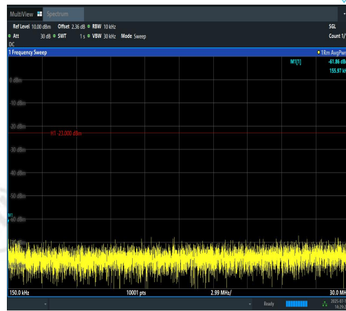
Band12-1.4MHz-16QAM-23017-1RB#5-0.15~30- PASS
