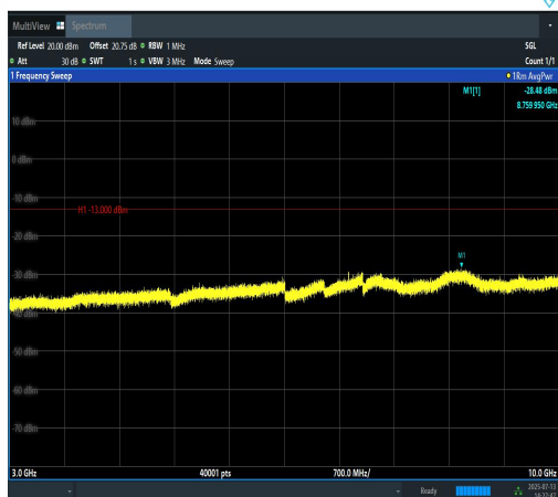
Band12-1.4MHz-QPSK-23017-1RB#0-3000~10000-PASS
