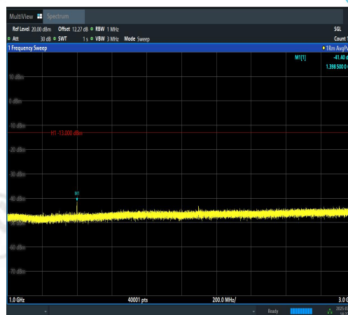
Band12-1.4MHz-QPSK-23017-1RB#0-1000~3000-PASS
