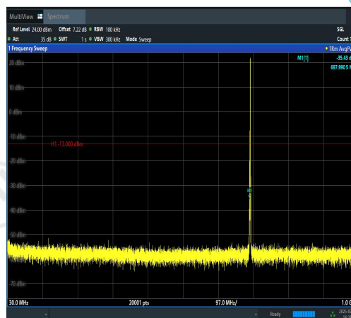
Band12-1.4MHz-QPSK-23017-1RB#5-30~1000-PASS
