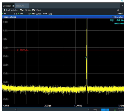
Band12-1.4MHz-QPSK-23017-1RB#0-30~1000-PASS
