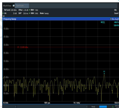
Band12-1.4MHz-QPSK-23017-1RB#5-0.009~0.15-PASS
