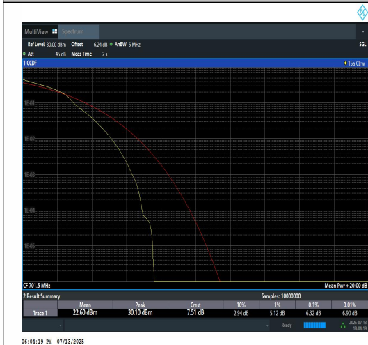
Band12-5MHz-16QAM-23035-1RB#0-PASS
