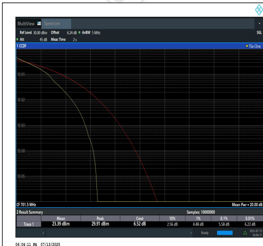
Band12-5MHz-QPSK-23035-1RB#0-PASS
