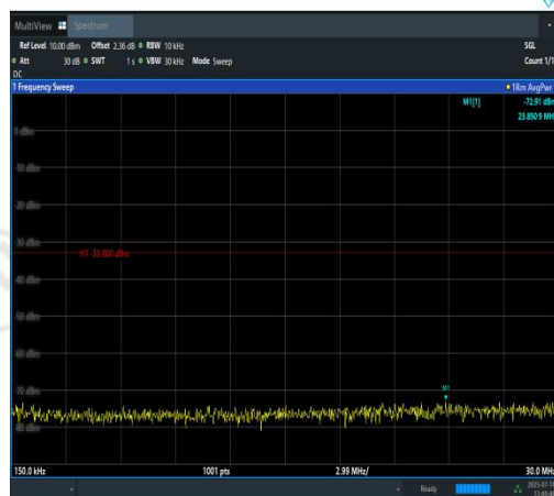
Band4-10MHz-16QAM-20350-1RB#49-0.15~30- PASS
