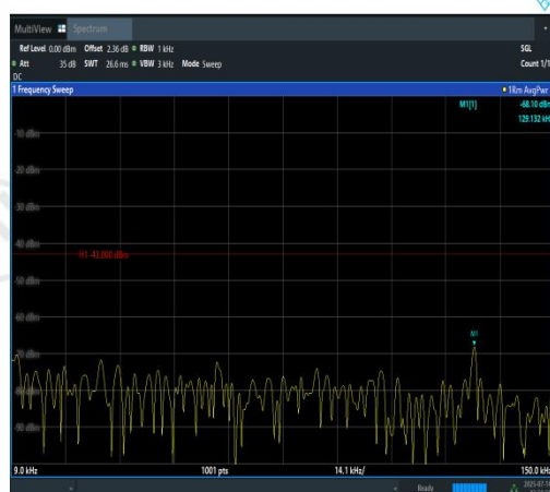
Band4-10MHz-16QAM-20350-50RB#0-0.009~0. 15-PASS
