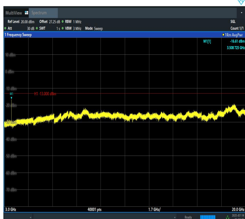
Band4-10MHz-16QAM-20350-1RB#49-3000~20000- 000-PASS
