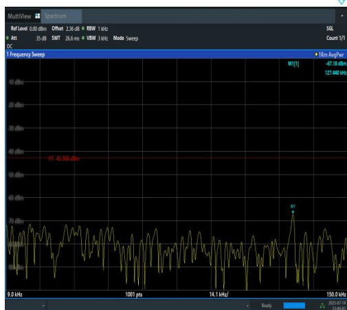
Band4-10MHz-16QAM-20350-1RB#49-0.009~0. 15-PASS
