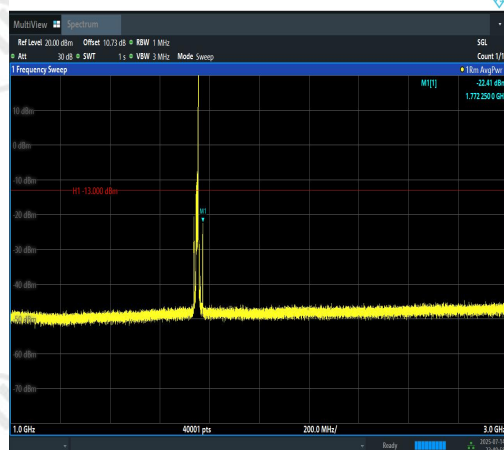
Band4-10MHz-16QAM-20350-1RB#49-1000~3000- 00-PASS
