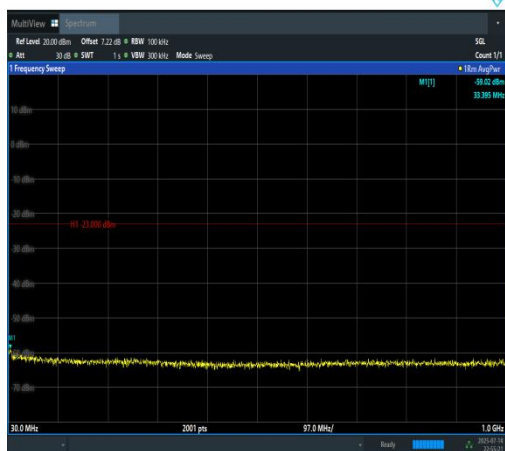
Band4-5MHz-QPSK-20375-1RB#0-30~1000-PA SS
