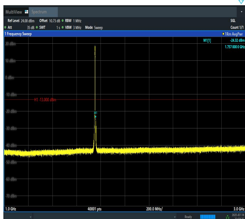
Band4-5MHz-16QAM-20375-25RB#0-1000~300 0-PASS
