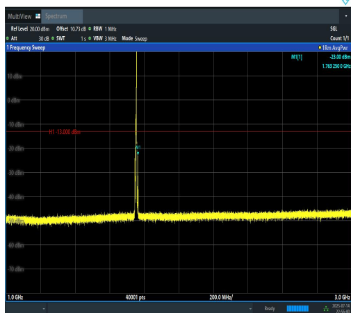
Band4-5MHz-QPSK-20375-1RB#24-1000~3000- PASS
