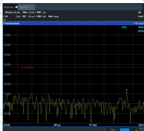
Band4-5MHz-QPSK-20375-1RB#24-0.009~0.15- PASS
