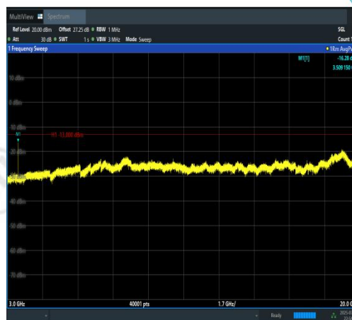
Band4-5MHz-QPSK-20375-1RB#24-3000~2000 0-PASS
