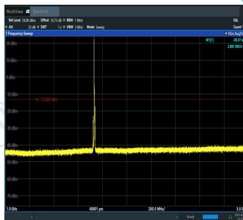
Band4-5MHz-QPSK-20175-1RB#0-1000~3000-P ASS
