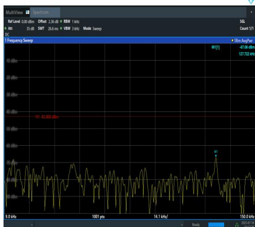
Band4-5MHz-QPSK-20375-25RB#0-0.009~0.15- PASS
