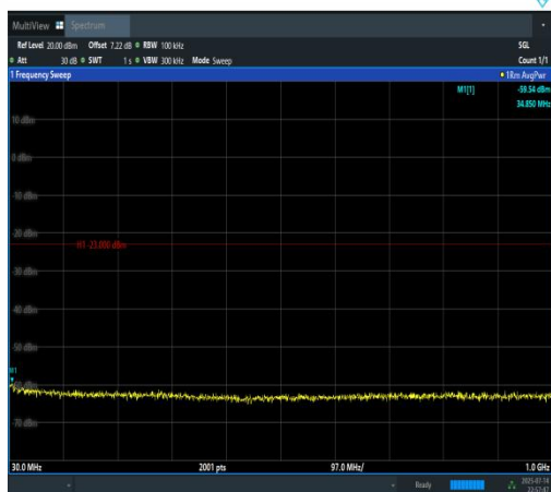
Band4-5MHz-QPSK-20375-25RB#0-30~1000-P ASS
