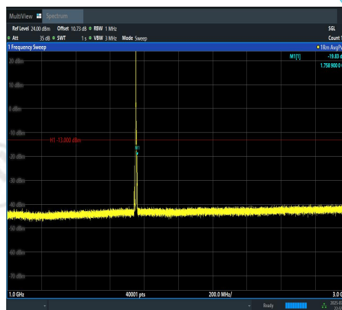
Band4-5MHz-QPSK-20375-1RB#0-1000~3000-P ASS
