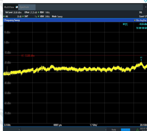
Band4-5MHz-16QAM-19975-25RB#0-3000~200 00-PASS
