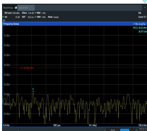
Band4-10MHz-QPSK-20000-1RB#0-0.009~0.15- PASS
