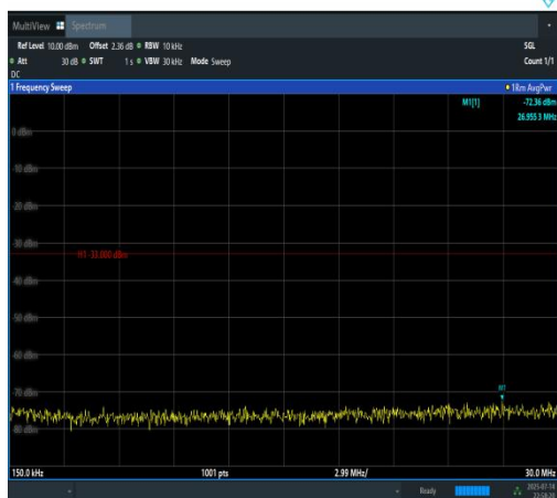
Band4-5MHz-16QAM-20375-25RB#0-0.15~30-P ASS
