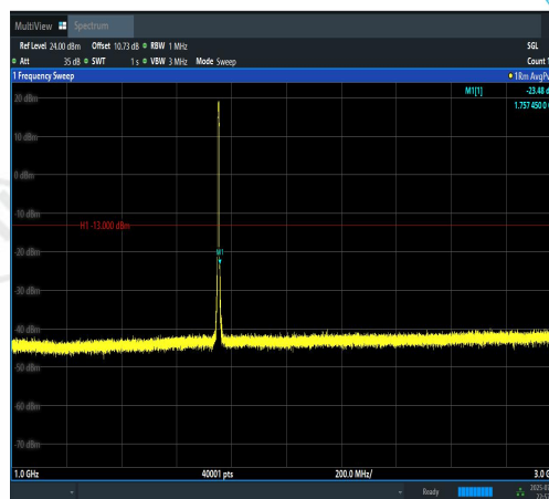
Band4-5MHz-QPSK-20375-25RB#0-1000~3000- PASS
