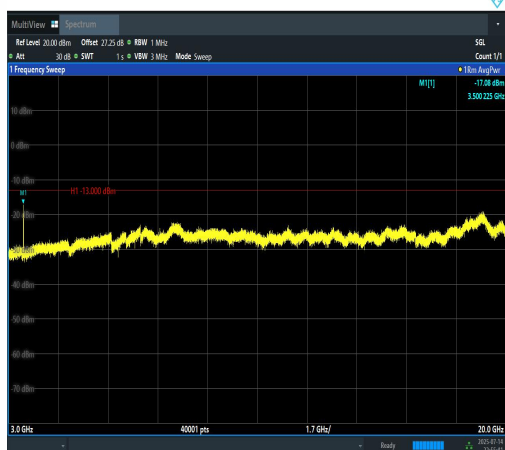
Band4-5MHz-QPSK-20375-1RB#0-3000~20000- PASS
