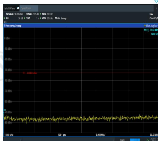
Band4-10MHz-QPSK-20000-1RB#0-0.15~30-PA SS
