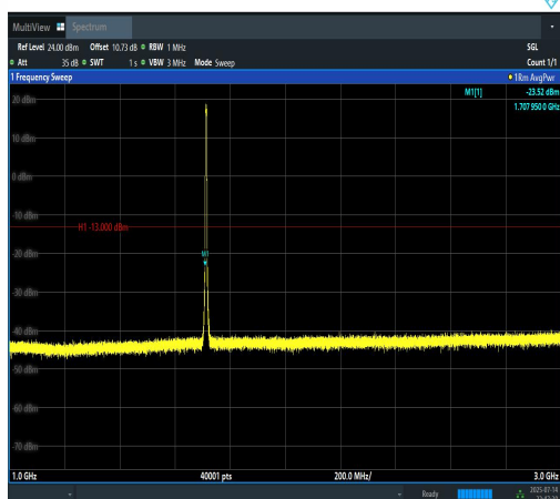
Band4-5MHz-16QAM-19975-25RB#0-1000~300 0-PASS
