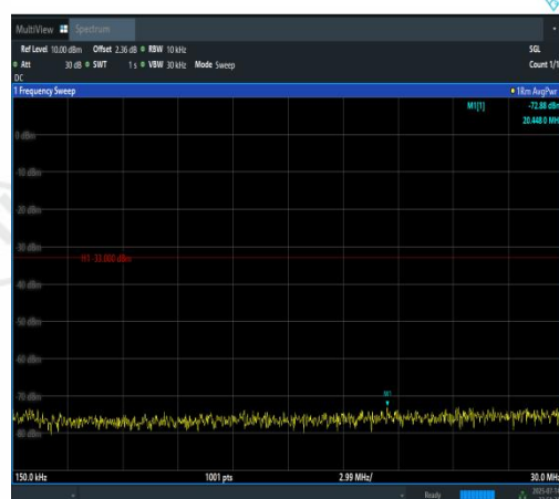
Band4-5MHz-QPSK-20175-1RB#0-0.15~30-PAS S
