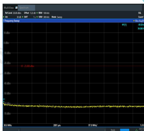
Band4-5MHz-QPSK-20175-1RB#24-30~1000-P ASS
