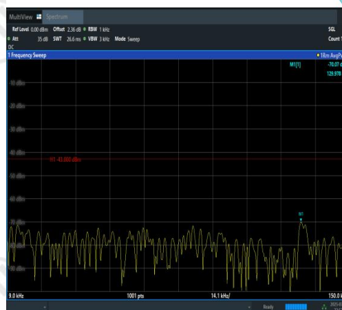
Band4-5MHz-QPSK-20175-1RB#24-0.009~0.15- PASS
