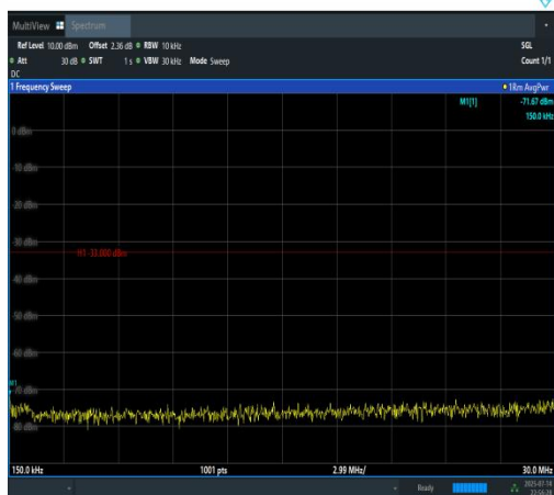
Band4-5MHz-QPSK-20375-1RB#24-0.15~30-PA SS
