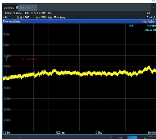
Band4-5MHz-QPSK-20175-1RB#0-3000~20000- PASS
