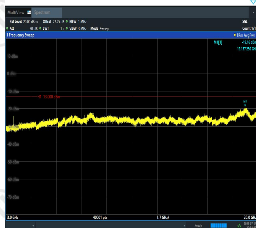
Band4-5MHz-16QAM-20375-25RB#0-3000~200 00-PASS
