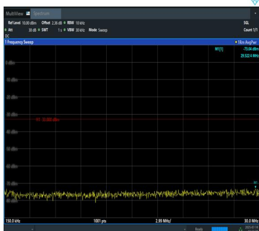
Band4-5MHz-QPSK-20175-1RB#24-0.15~30-PA SS
