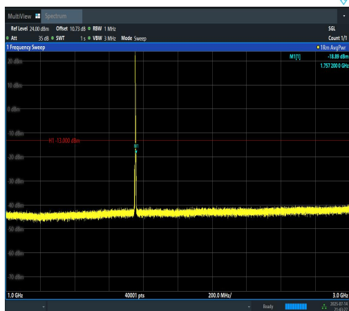
Band4-3MHz-16QAM-20385-1RB#0-1000~3000- PASS
