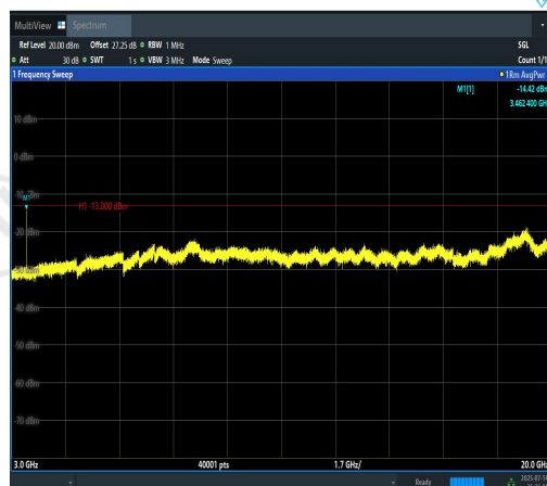
Band4-3MHz-16QAM-20175-1RB#0-3000~2000 0-PASS
