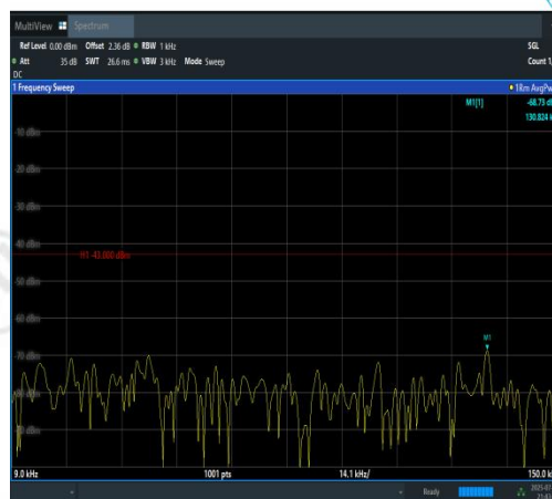
Band4-3MHz-16QAM-20385-1RB#0-0.009~0.15- PASS
