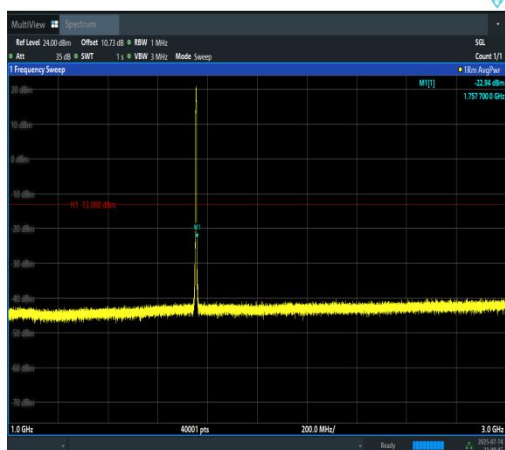
Band4-3MHz-16QAM-20385-15RB#0-1000~300 0-PASS
