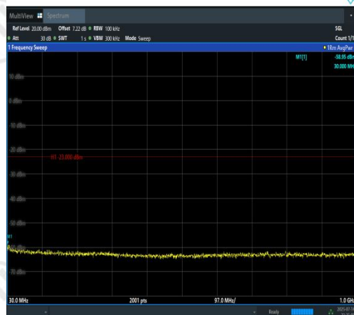
Band4-3MHz-16QAM-20175-1RB#0-30~1000-P ASS
