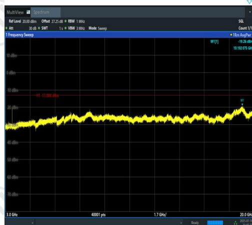
Band4-3MHz-16QAM-20175-15RB#0-3000~200 00-PASS
