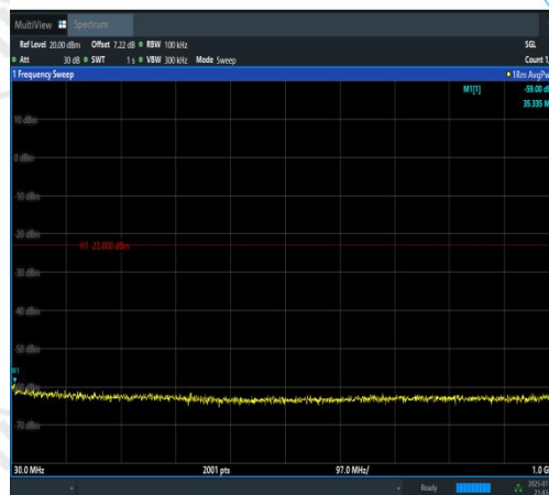
Band4-3MHz-16QAM-20385-1RB#0-30~1000-P ASS
