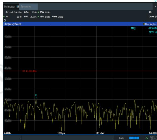
Band4-3MHz-16QAM-20175-1RB#0-0.009~0.15- PASS
