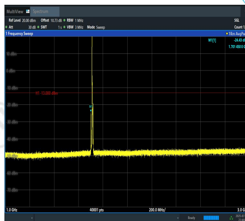
Band4-5MHz-QPSK-19975-1RB#0-1000~3000-P ASS
