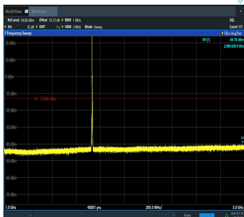
Band4-3MHz-16QAM-20175-1RB#0-1000~3000- PASS
