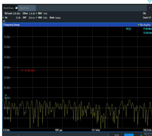
Band4-3MHz-QPSK-20385-1RB#0-0.009~0.15-P ASS
