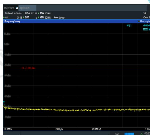
Band4-5MHz-QPSK-19975-1RB#24-30~1000-P ASS
