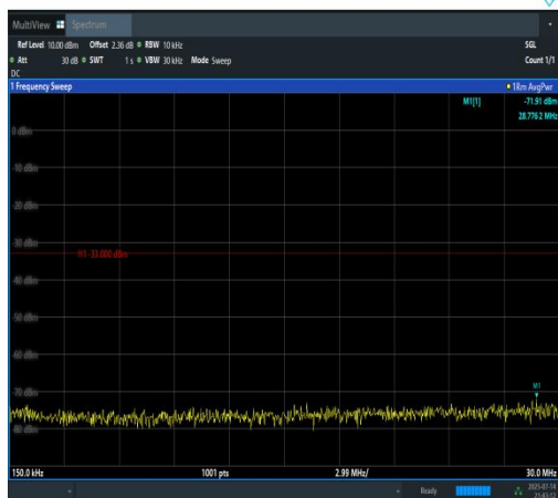
Band4-3MHz-16QAM-20385-1RB#0-0.15~30-PA SS
