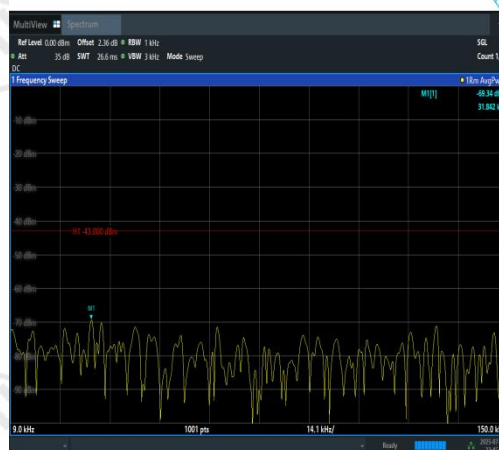
Band4-5MHz-QPSK-19975-1RB#24-0.009~0.15- PASS
