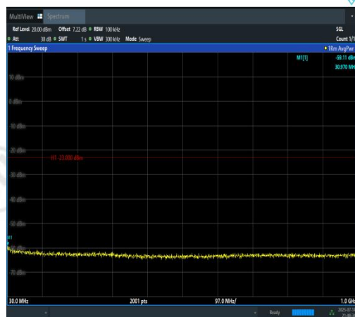
Band4-3MHz-16QAM-20385-15RB#0-30~1000-P ASS
