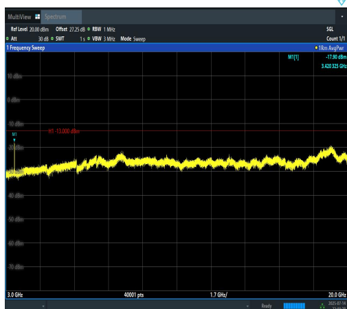
Band4-5MHz-QPSK-19975-1RB#0-3000~20000- PASS
