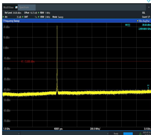
Band4-3MHz-16QAM-20175-15RB#0-1000~300 0-PASS
