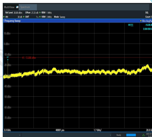
Band4-3MHz-16QAM-20385-1RB#0-3000~2000 0-PASS
