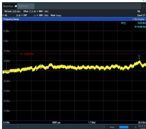
Band4-3MHz-QPSK-20175-15RB#0-3000~2000 0-PASS
