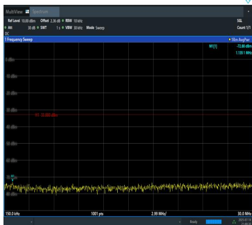
Band4-3MHz-16QAM-20385-15RB#0-0.15~30-P ASS
