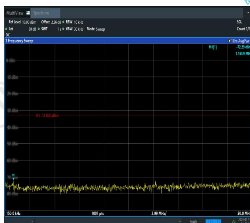
Band4-3MHz-QPSK-20385-1RB#0-0.15~30-PAS S
