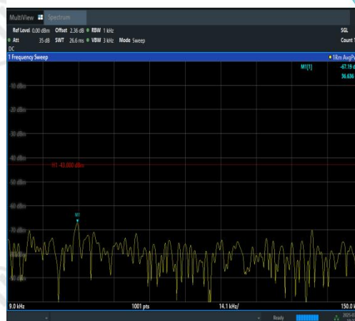
Band4-1.4MHz-QPSK-20175-1RB#5-0.009~0.15 -PASS
