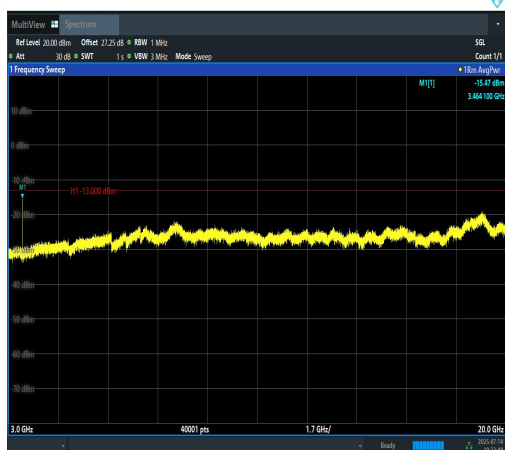
Band4-1.4MHz-QPSK-20175-1RB#0-3000~2000 0-PASS
