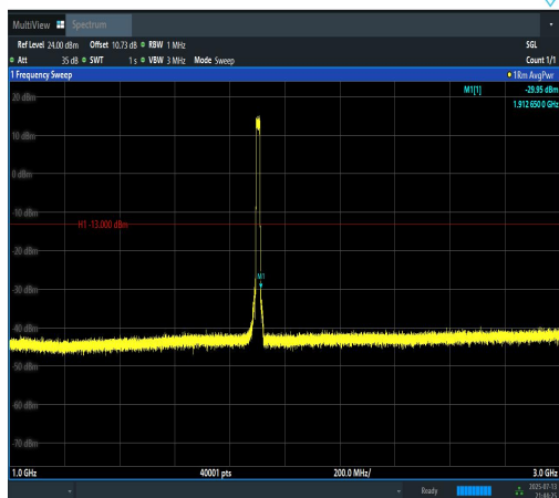
Band2-15MHz-16QAM-19125-75RB#0-1000~30 00-PASS
