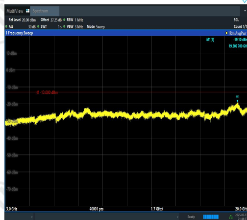
Band2-15MHz-16QAM-19125-75RB#0-3000~20 000-PASS
