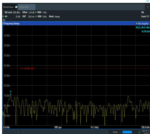
Band2-20MHz-QPSK-18700-1RB#0-0.009~0.15- PASS
