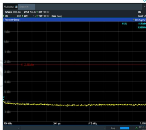
Band2-15MHz-16QAM-19125-75RB#0-30~1000- PASS
