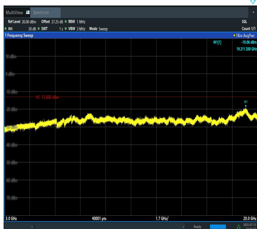
Band2-15MHz-QPSK-19125-1RB#0-3000~2000 0-PASS
