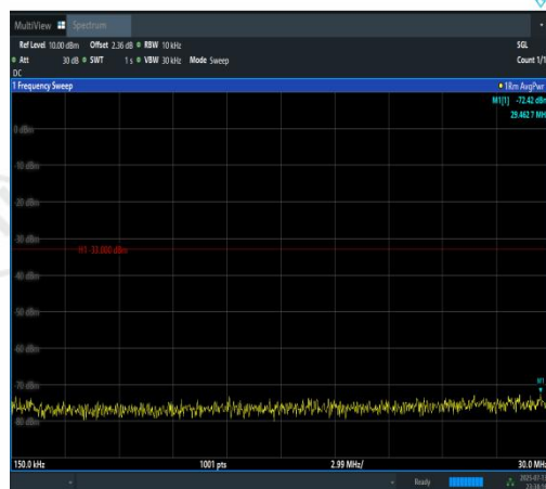
Band2-20MHz-QPSK-18700-1RB#0-0.15~30-PA SS
