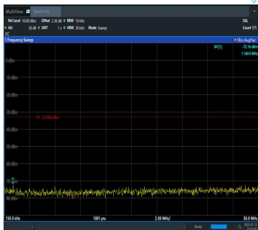
Band2-15MHz-16QAM-19125-1RB#0-0.15~30-P ASS
