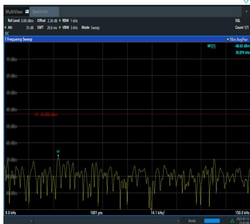
Band2-15MHz-QPSK-19125-1RB#0-0.009~0.15-PASS
