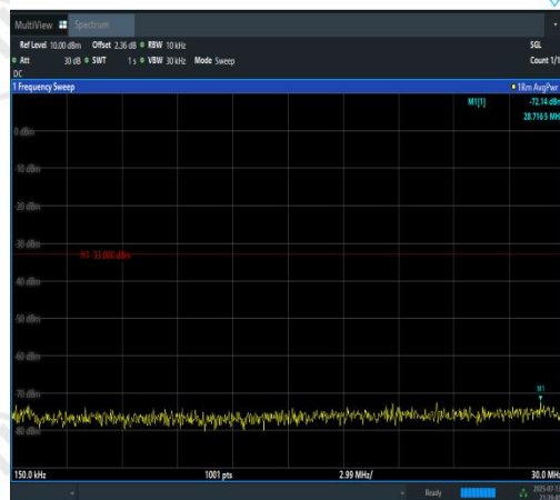
Band2-15MHz-QPSK-18900-75RB#0-0.15~30-P ASS
