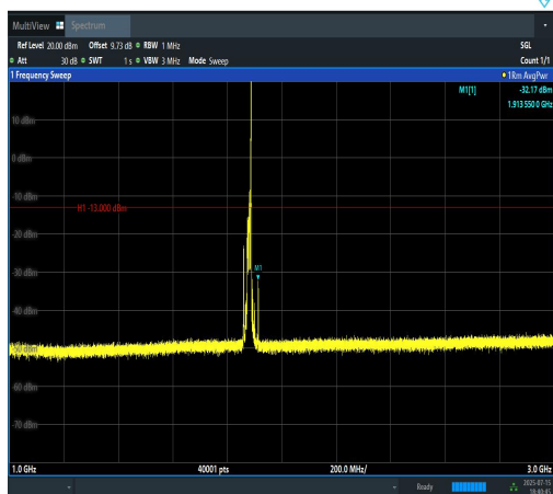
Band2-15MHz-QPSK-18900-1RB#74-1000~300 0-PASS
