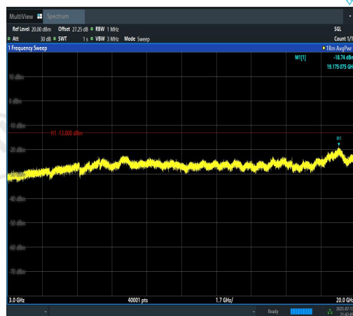
Band2-15MHz-16QAM-19125-1RB#0-3000~200 00-PASS
