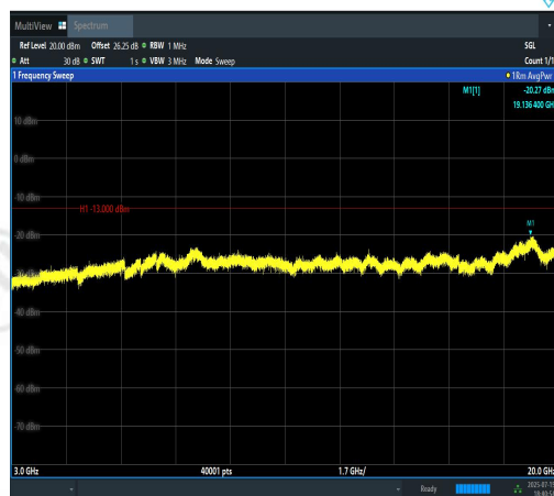
Band2-15MHz-QPSK-18900-1RB#74-3000~200 00-PASS
