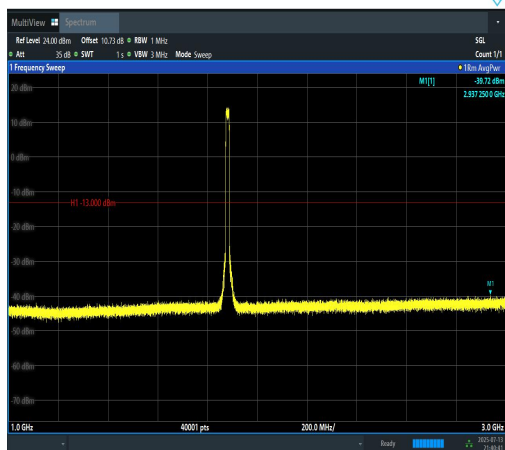
Band2-15MHz-16QAM-18900-75RB#0-1000~3000-PASS
