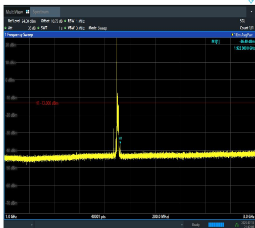
Band2-15MHz-16QAM-19125-1RB#0-1000~300 0-PASS
