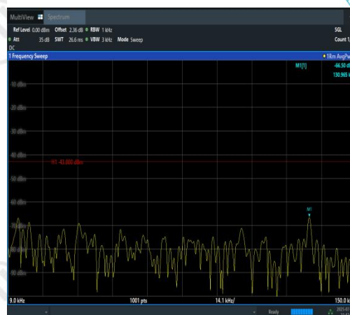
Band2-15MHz-QPSK-19125-1RB#74-0.009~0.1 5-PASS
