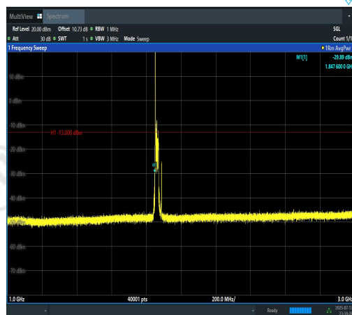
Band2-20MHz-QPSK-18700-1RB#0-1000~3000- PASS
