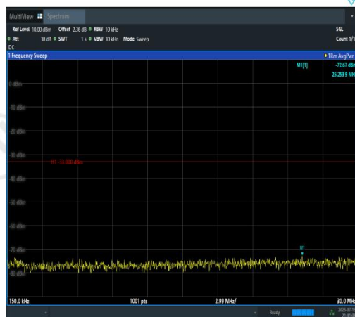
Band2-15MHz-QPSK-19125-1RB#0-0.15~30-PASS
