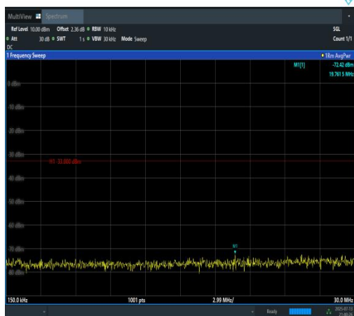
Band2-15MHz-16QAM-18900-75RB#0-0.15~30-PASS
