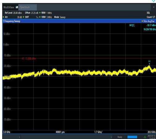
Band2-15MHz-QPSK-19125-75RB#0-3000~200 00-PASS
