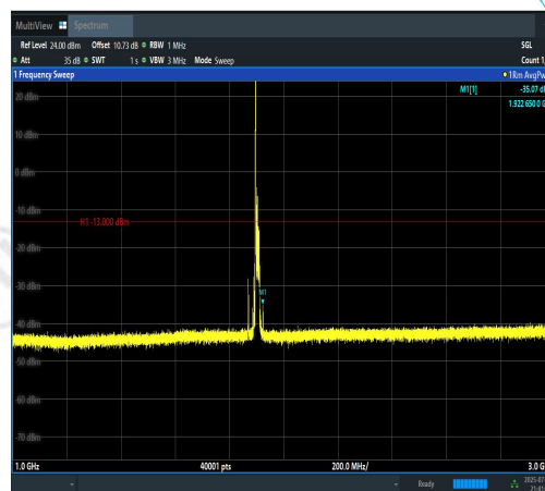
Band2-15MHz-QPSK-19125-1RB#0-1000~3000- PASS
