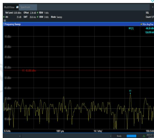
Band2-15MHz-16QAM-19125-1RB#0-0.009~0.1 5-PASS
