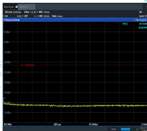
Band2-15MHz-16QAM-18900-75RB#0-30~1000-PASS
