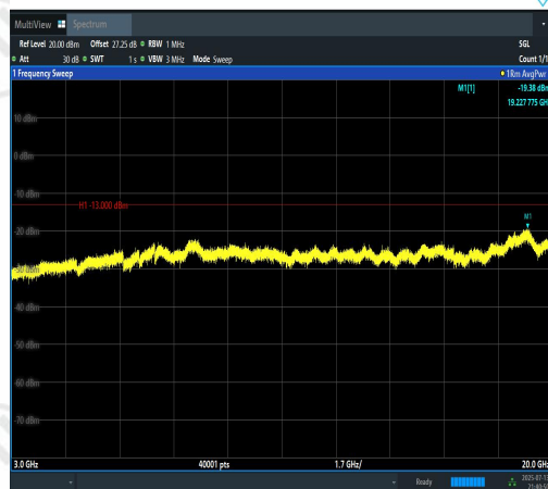
Band2-15MHz-16QAM-18900-75RB#0-3000~20000-PASS
