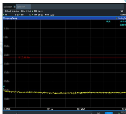
Band2-15MHz-QPSK-19125-1RB#74-30~1000-P ASS
