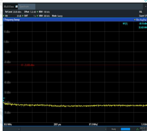
Band2-15MHz-16QAM-19125-1RB#0-30~1000-P ASS
