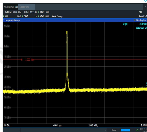
Band2-15MHz-QPSK-18900-75RB#0-1000~300 0-PASS
