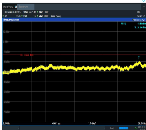
Band2-10MHz-16QAM-19150-1RB#49-3000~20000- 000-PASS
