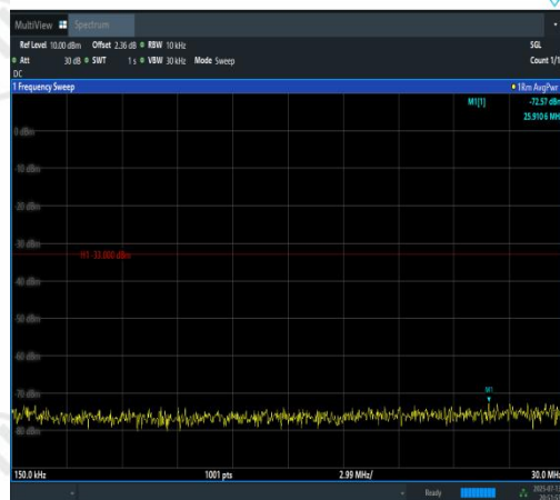
Band2-10MHz-QPSK-19150-50RB#0-0.15~30-P ASS
