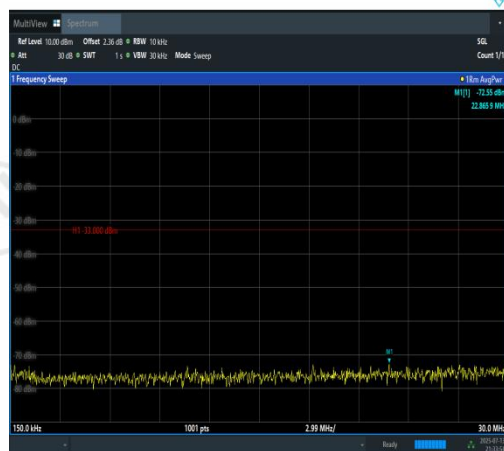
Band2-15MHz-QPSK-18675-1RB#0-0.15~30-PA SS
