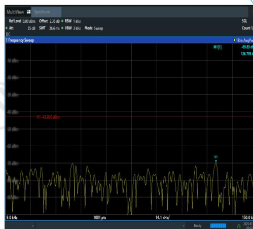
Band2-10MHz-16QAM-19150-50RB#0-0.009~0. 15-PASS
