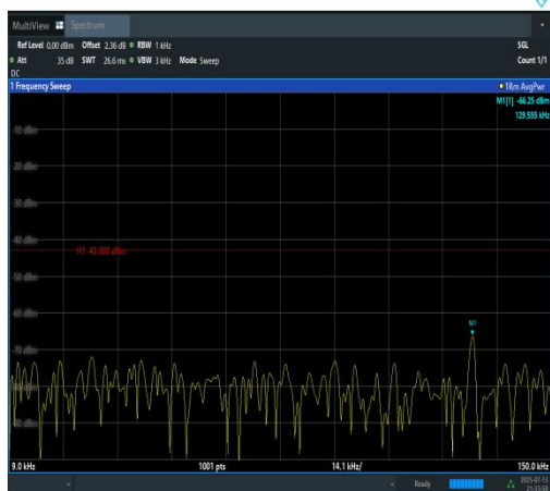
Band2-15MHz-QPSK-18675-1RB#0-0.009~0.15- PASS
