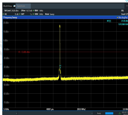
Band2-10MHz-QPSK-19150-50RB#0-1000~300 0-PASS
