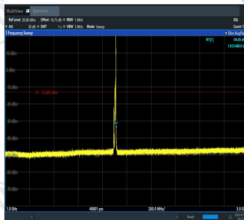
Band2-10MHz-16QAM-19150-1RB#49-1000~3000- 00-PASS
