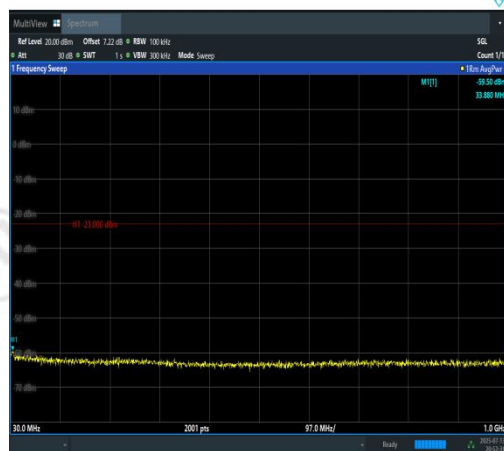
Band2-10MHz-16QAM-19150-50RB#0-30~1000- PASS
