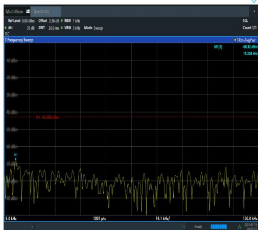
Band2-10MHz-QPSK-19150-50RB#0-0.009~0.1 5-PASS
