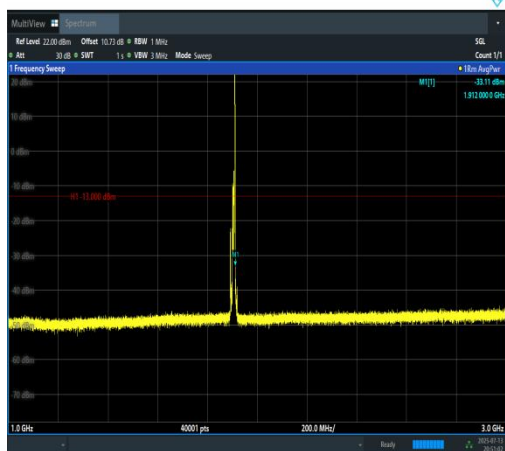
Band2-10MHz-QPSK-19150-1RB#49-1000~300 0-PASS
