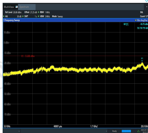
Band2-10MHz-QPSK-19150-1RB#49-3000~200 00-PASS
