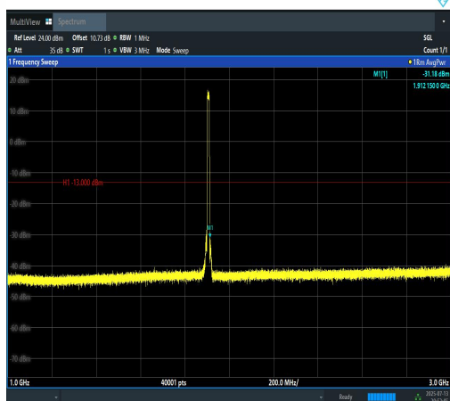
Band2-10MHz-16QAM-19150-50RB#0-1000~30 00-PASS
