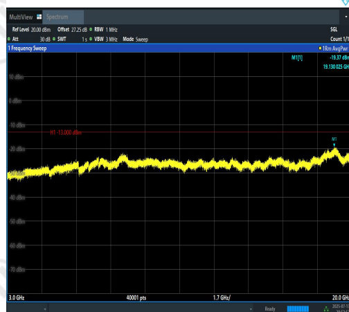
Band2-10MHz-16QAM-19150-50RB#0-3000~20 000-PASS
