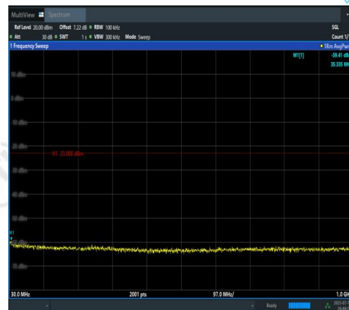
Band2-10MHz-16QAM-18900-50RB#0-30~1000-PASS
