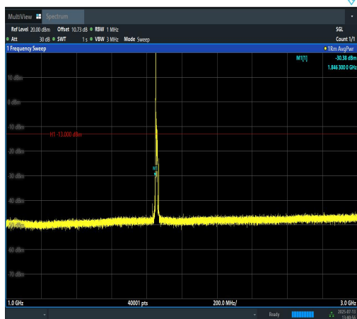
Band2-10MHz-16QAM-18650-1RB#0-1000~300 0-PASS
