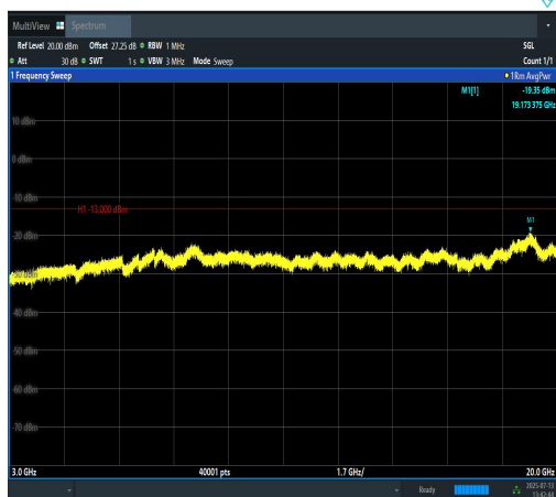
Band2-10MHz-QPSK-18650-50RB#0-3000~200 00-PASS
