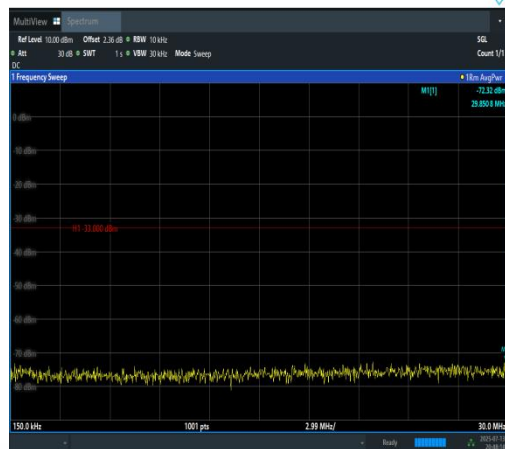
Band2-10MHz-16QAM-18900-50RB#0-0.15~30-PASS
