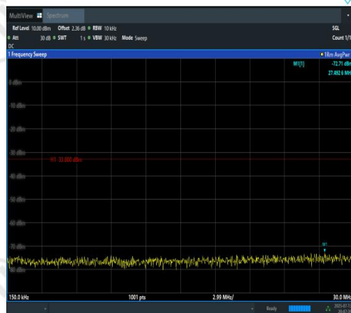
Band2-10MHz-QPSK-18900-50RB#0-0.15~30-P ASS
