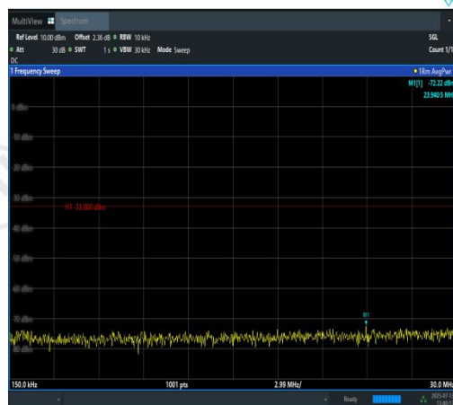
Band2-10MHz-QPSK-18650-1RB#0-0.15~30-PA SS
