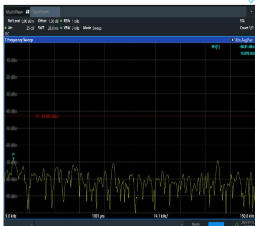
Band2-10MHz-QPSK-18900-1RB#0-0.009~0.15- PASS
