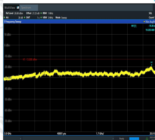
Band2-10MHz-16QAM-18650-50RB#0-3000~20 000-PASS
