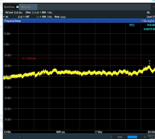
Band2-5MHz-16QAM-19175-25RB#0-3000~200 00-PASS
