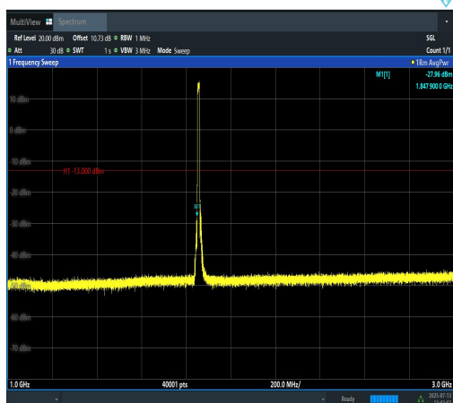
Band2-10MHz-16QAM-18650-50RB#0-1000~30 00-PASS
