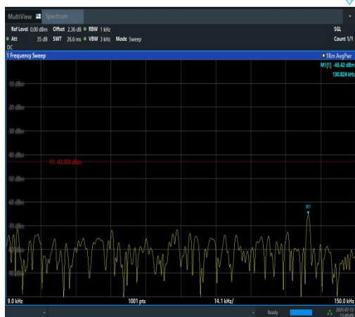
Band2-10MHz-QPSK-18650-1RB#0-0.009~0.15- PASS
