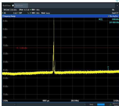
Band2-10MHz-QPSK-18900-1RB#49-1000~300 0-PASS
