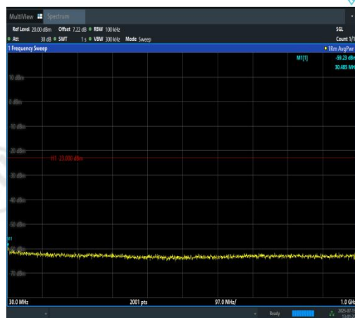
Band2-5MHz-16QAM-19175-25RB#0-30~1000-P ASS
