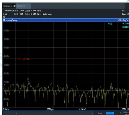
Band2-10MHz-16QAM-18650-1RB#0-0.009~0.1 5-PASS
