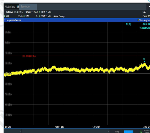
Band2-10MHz-16QAM-18900-50RB#0-3000~20000-PASS
