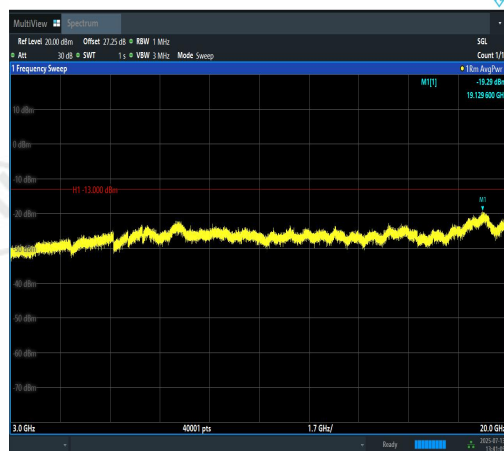
Band2-10MHz-16QAM-18650-1RB#0-3000~200 00-PASS
