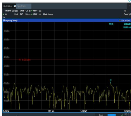
Band2-10MHz-QPSK-19150-1RB#0-0.009~0.15-PASS
