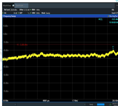
Band2-10MHz-QPSK-18900-1RB#49-3000~200 00-PASS
