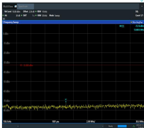
Band2-10MHz-16QAM-18650-1RB#0-0.15~30-P ASS
