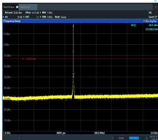
Band2-5MHz-16QAM-19175-25RB#0-1000~300 0-PASS
