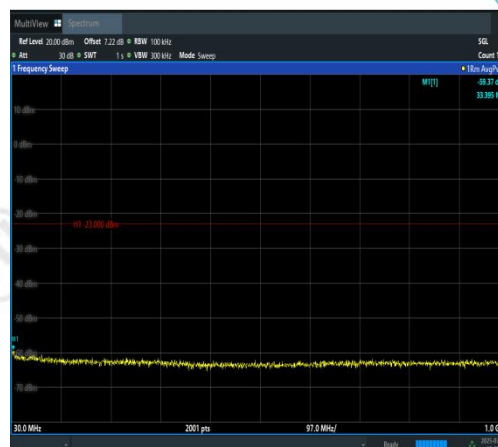
Band2-10MHz-16QAM-18650-50RB#0-30~1000- PASS
