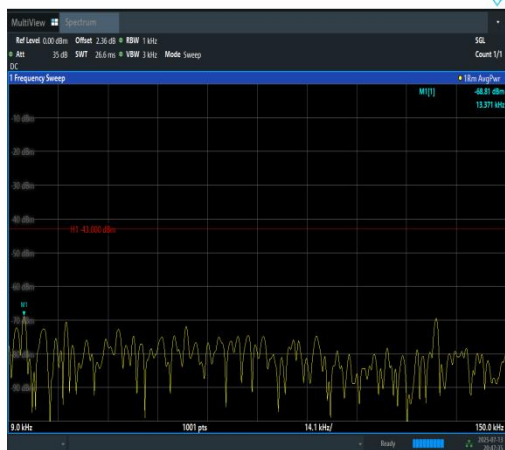
Band2-10MHz-QPSK-18900-50RB#0-0.009~0.1 5-PASS
