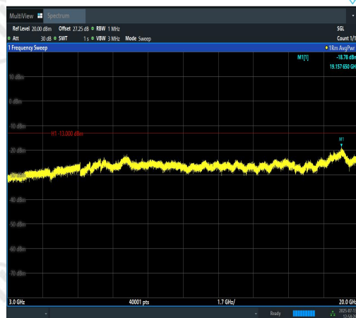
Band2-5MHz-16QAM-18625-25RB#0-3000~200 00-PASS
