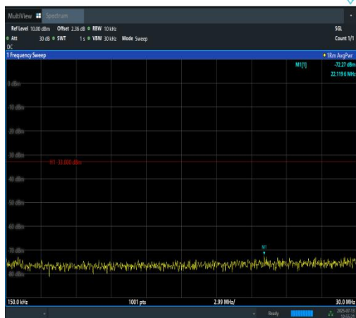
Band2-5MHz-16QAM-18900-1RB#0-0.15~30-PA SS
