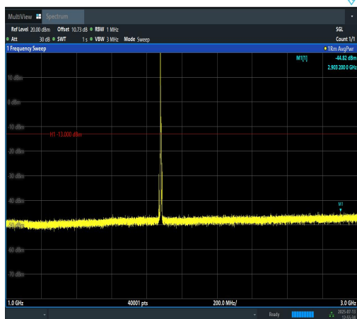
Band2-5MHz-16QAM-18900-1RB#0-1000~3000- PASS
