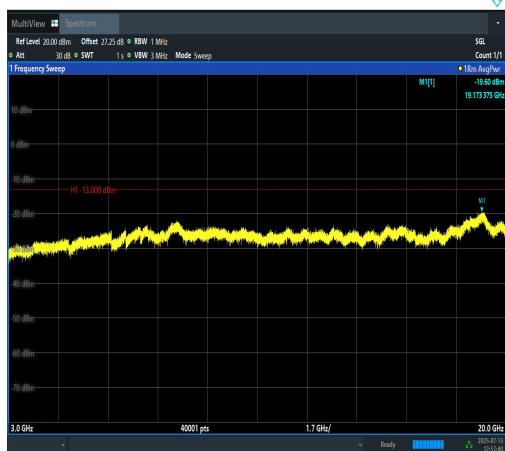
Band2-5MHz-QPSK-18900-25RB#0-3000~2000 0-PASS
