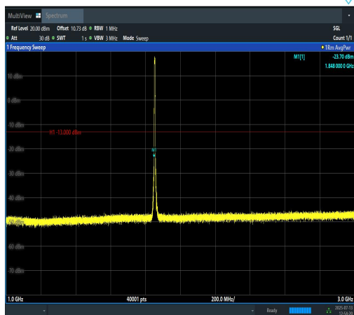
Band2-5MHz-16QAM-18625-25RB#0-1000~300 0-PASS
