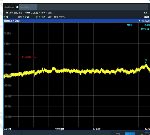
Band2-5MHz-16QAM-18900-25RB#0-3000~200 00-PASS
