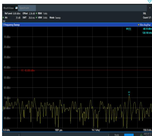
Band2-5MHz-QPSK-19175-1RB#0-0.009~0.15-P ASS
