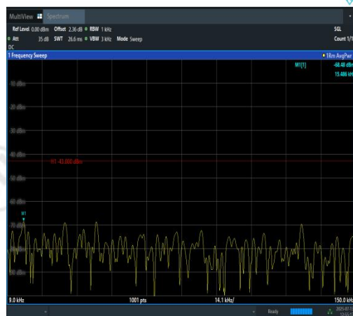
Band2-5MHz-16QAM-18900-1RB#0-0.009~0.15- PASS
