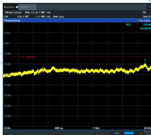
Band2-5MHz-16QAM-18900-1RB#0-3000~2000 0-PASS
