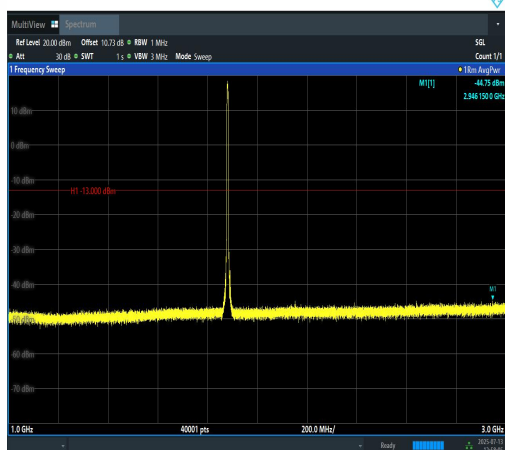
Band2-5MHz-16QAM-18900-25RB#0-1000~300 0-PASS
