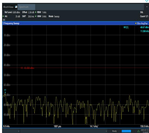
Band2-5MHz-QPSK-18900-1RB#0-0.009~0.15-P ASS
