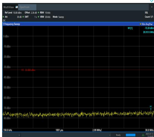
Band2-5MHz-16QAM-18625-25RB#0-0.15~30-P ASS
