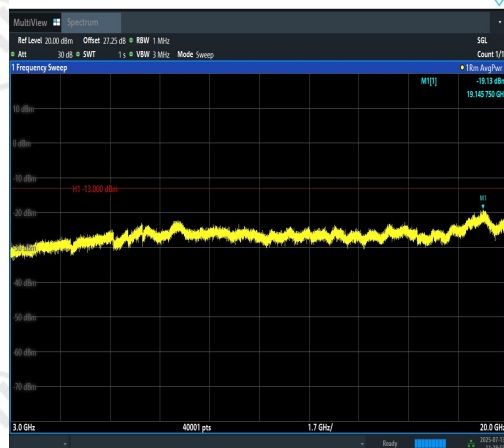
Band2-1.4MHz-16QAM-18900-6RB#0-3000~200 00-PASS
