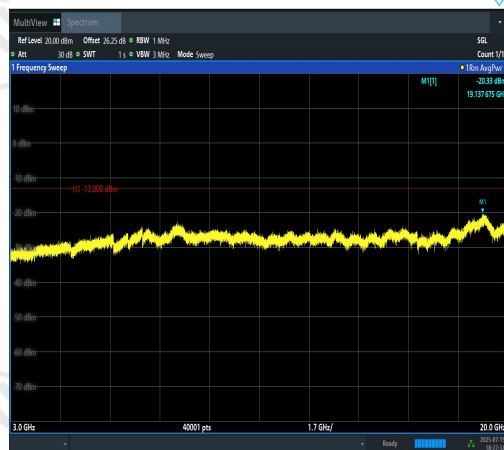
Band2-3MHz-16QAM-18615-15RB#0-3000~200 00-PASS
