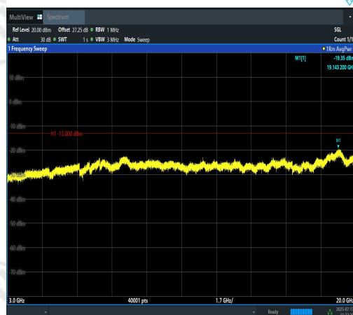
Band2-1.4MHz-16QAM-19193-6RB#0-3000~200 00-PASS
