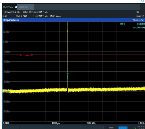
Band2-1.4MHz-16QAM-19193-6RB#0-1000~3000 0-PASS
