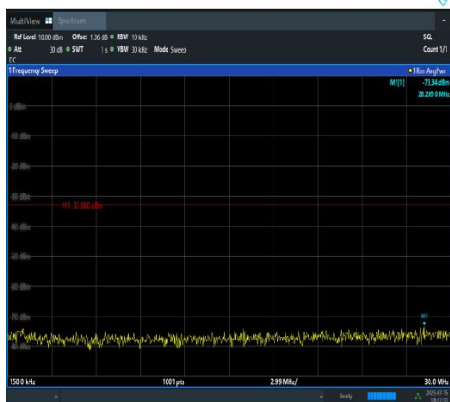
Band2-3MHz-16QAM-18615-15RB#0-0.15~30-P ASS
