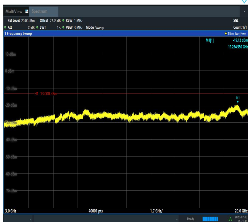
Band2-1.4MHz-QPSK-19193-6RB#0-3000~2000 0-PASS
