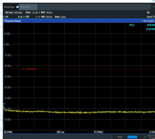
Band2-1.4MHz-16QAM-19193-1RB#0-30~1000- PASS
