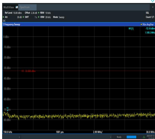
Band2-1.4MHz-16QAM-19193-6RB#0-0.15~30-P ASS
