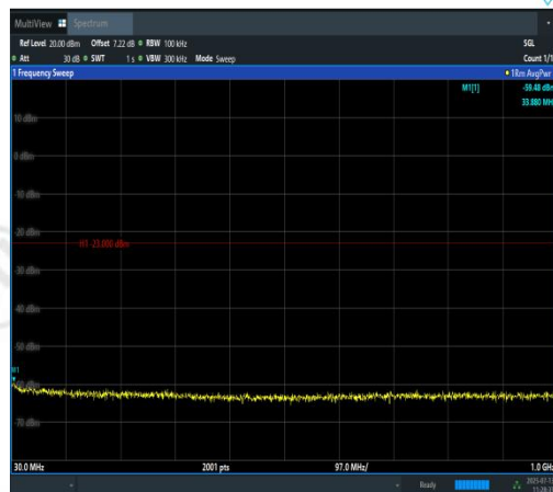
Band2-1.4MHz-16QAM-18900-6RB#0-30~1000- PASS
