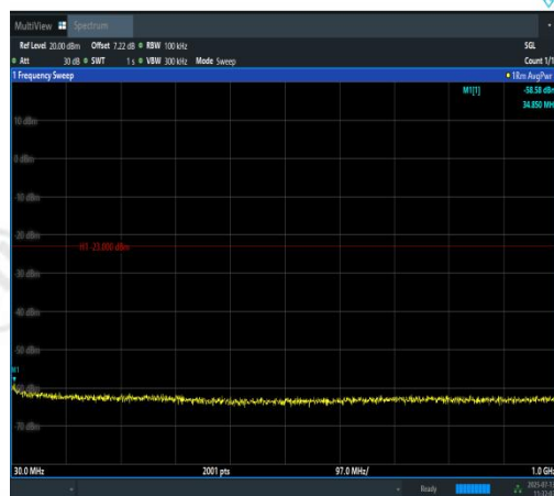
Band2-1.4MHz-16QAM-19193-6RB#0-30~1000- PASS
