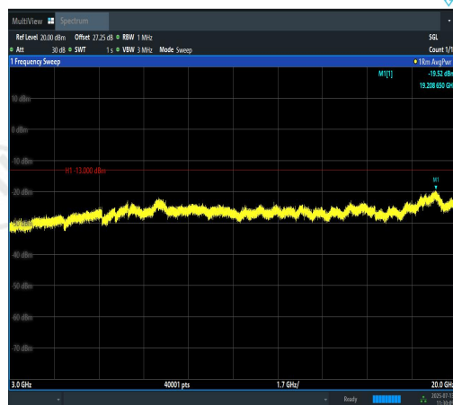
Band2-1.4MHz-16QAM-19193-1RB#0-3000~200 00-PASS
