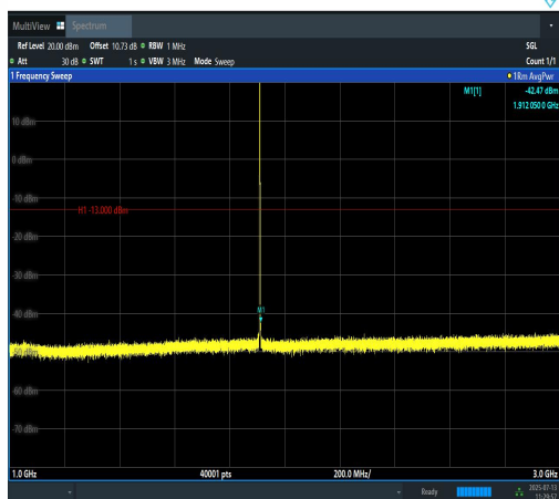
Band2-1.4MHz-16QAM-19193-1RB#0-1000~300 0-PASS
