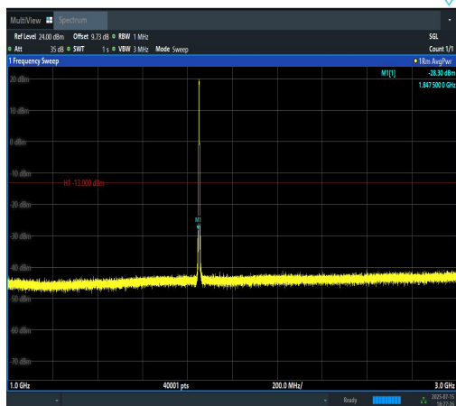
Band2-3MHz-16QAM-18615-15RB#0-1000~300 0-PASS
