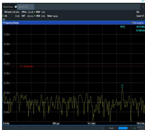
Band2-3MHz-QPSK-18615-1RB#0-0.009~0.15-P ASS
