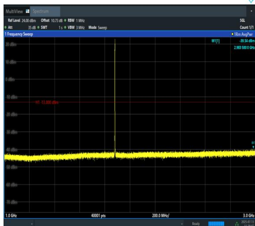
Band2-1.4MHz-16QAM-18900-6RB#0-1000~3000 0-PASS
