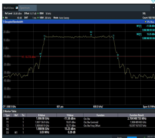
Band2-3MHz-QPSK-19185-15RB#0-PASS
