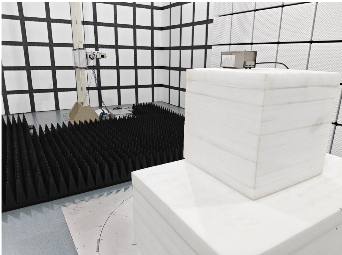
Radiated Spurious Emissions Test View (18GHz-25GHz)
