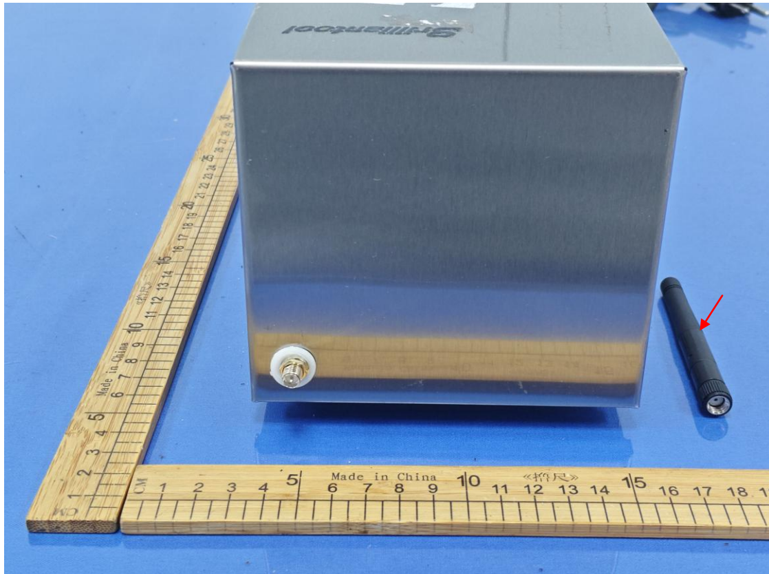
Model: MTM0300-15-WIFI-1-SS, BLE/2.4G WIFI ANT.
