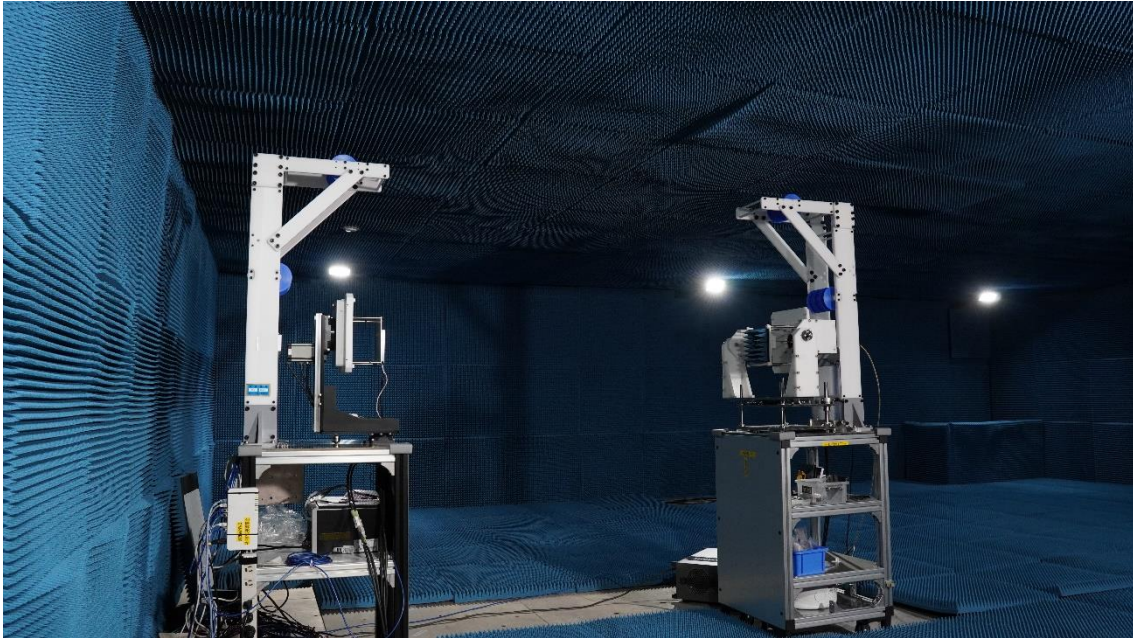
Figure 5-1: Test set up photo
