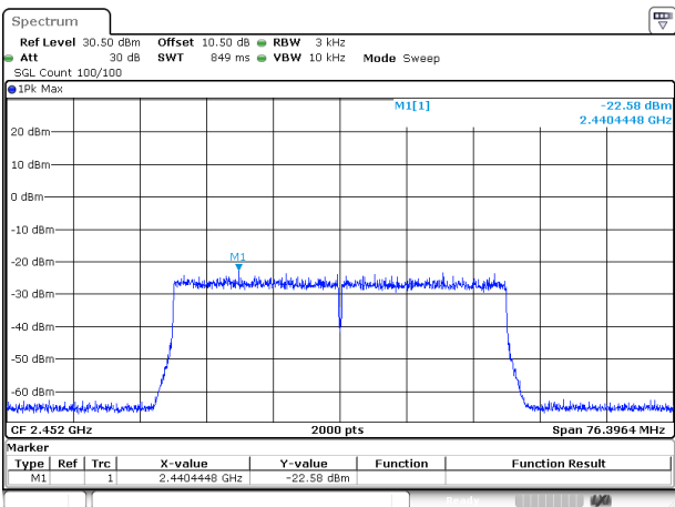
802.11ax40_2452MHz_RU_Full
