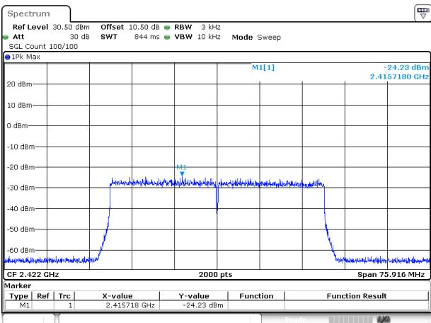
802.11ax40_2422MHz_RU_Full
