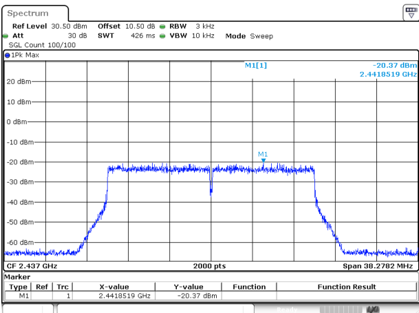
802.11ax20_2437MHz_RU_Full
