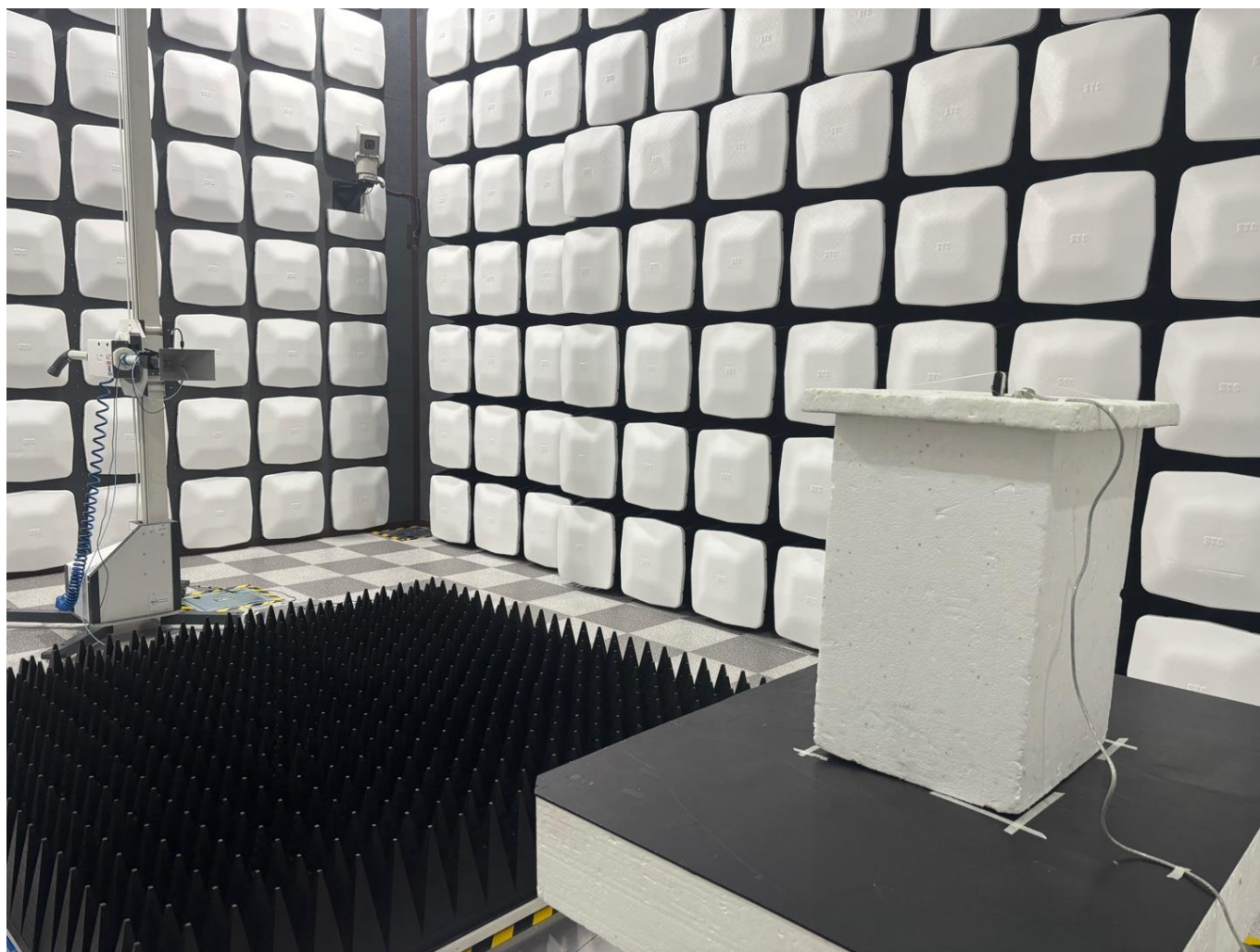
Above 1 GHz
