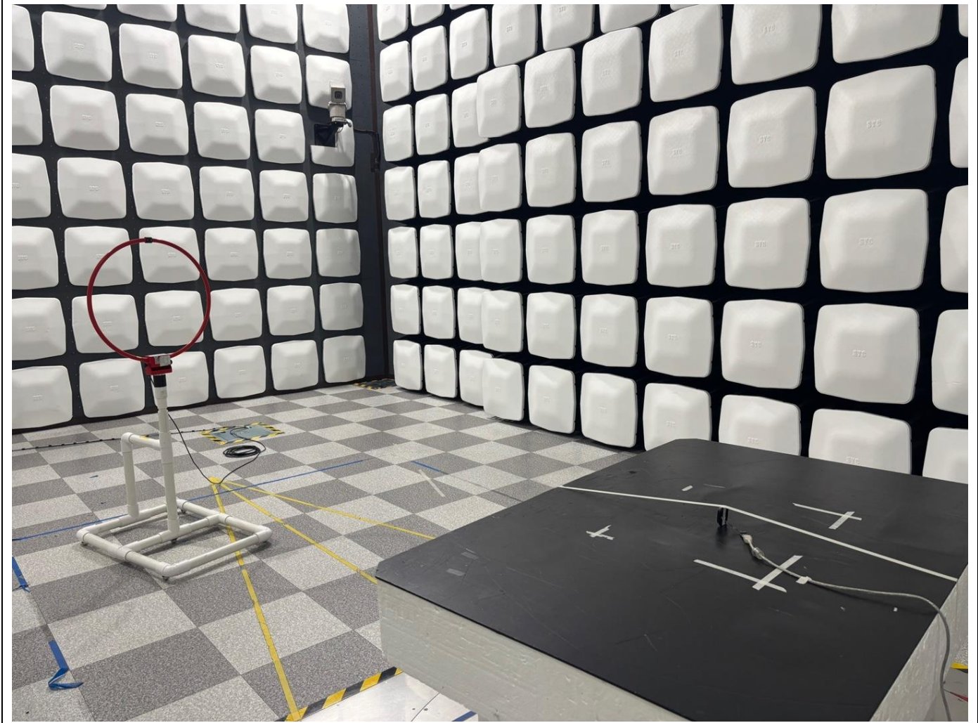
Below 30 MHz
