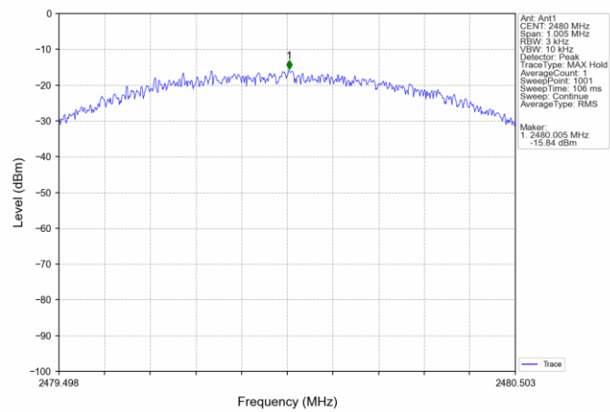
1M_HCH_2480MHz_Ant1_NTNV
