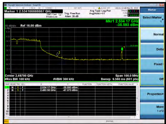
802.11n_Band2.4G_BW40MHz
