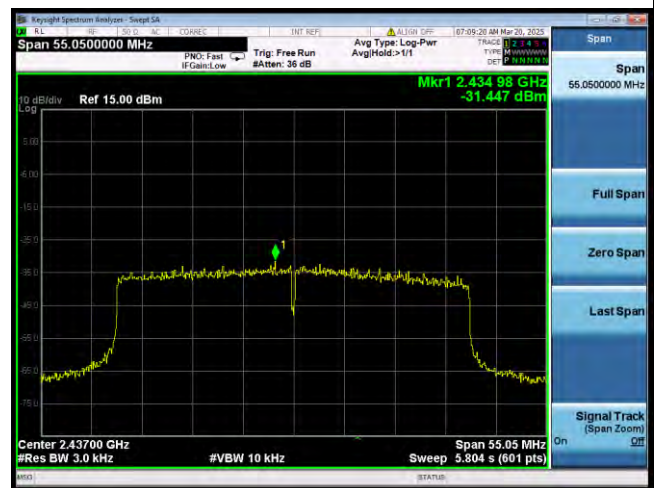
802.11ax_Band2.4G_BW40MHz_2437MHz
