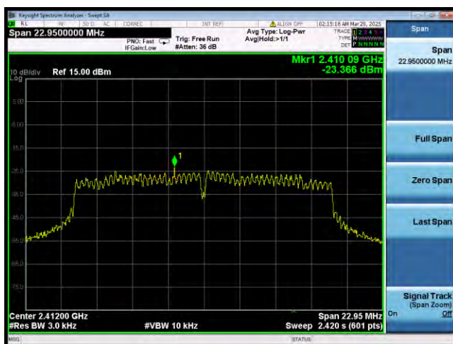
802.11g 2412MHz
