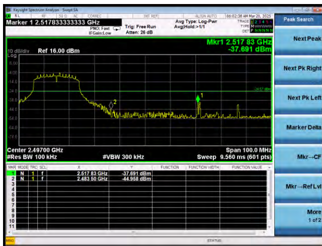
802.11n_Band2.4G_BW20MHz
