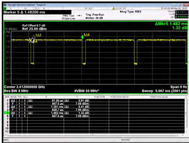
802.11g 2412MHz
