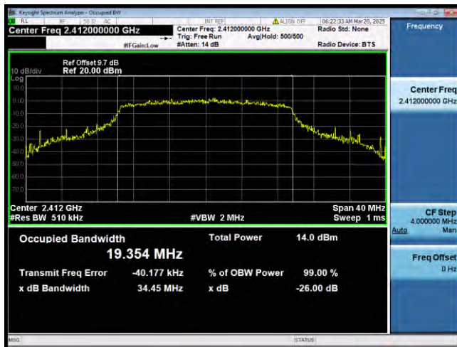
802.11ax_Band2.4G_BW20MHz MHz
