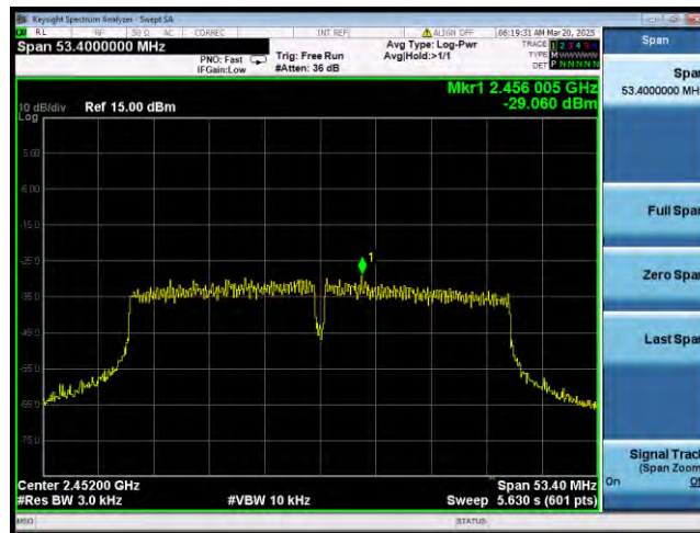
802.11n_Band2.4G_BW40MHz_2452MHz
