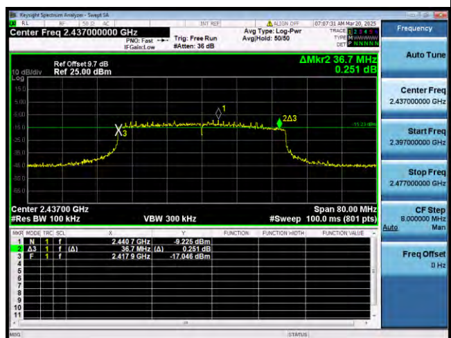
802.11ax_Band2.4G_BW40MHz MHz
