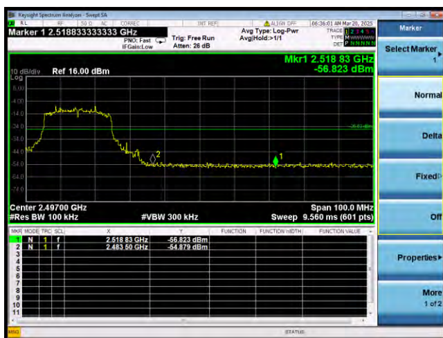
802.11ax_Band2.4G_BW20MHz
