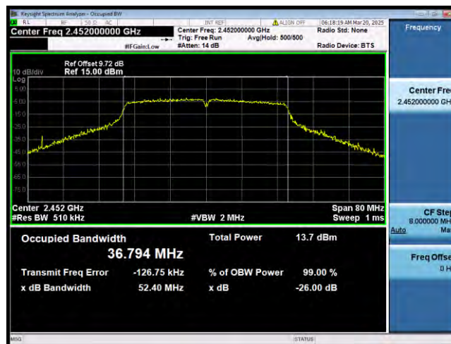
802.11n_Band2.4G_BW40MHz MHz
