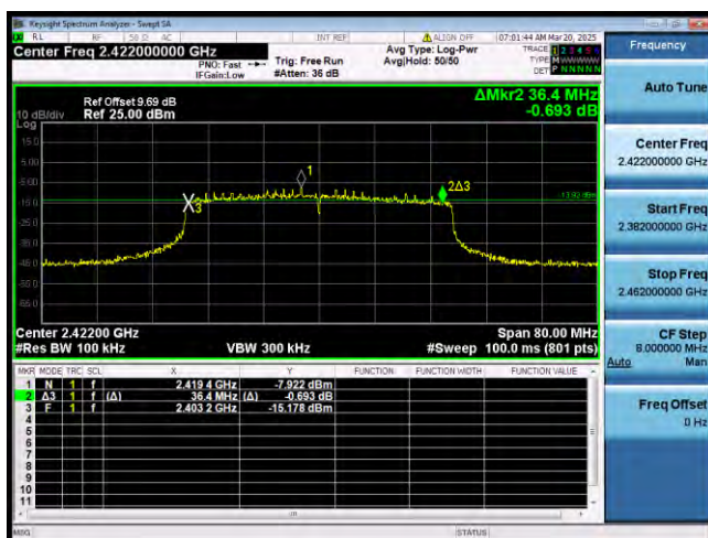
802.11ax_Band2.4G_BW40MHz MHz
