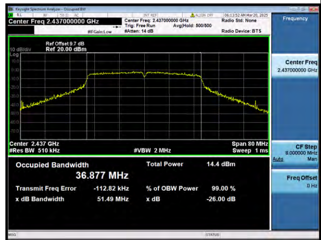
802.11n_Band2.4G_BW40MHz MHz
