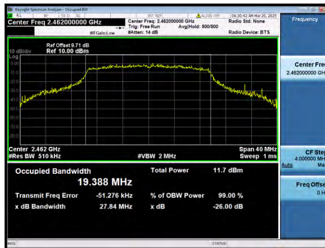
802.11ax_Band2.4G_BW20MHz MHz
