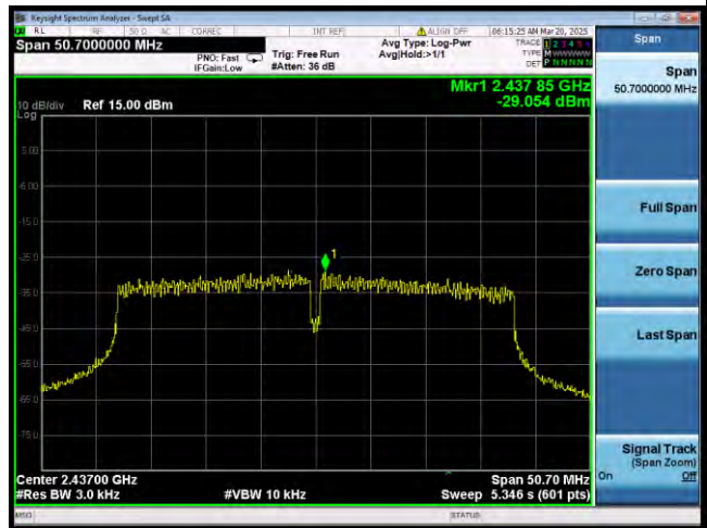
802.11n_Band2.4G_BW40MHz_2437MHz
