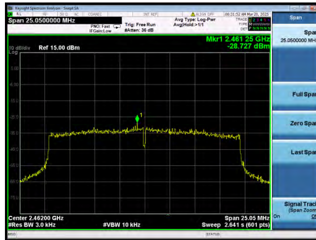
802.11ax_Band2.4G_BW20MHz_2462MHz
