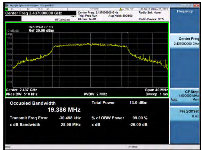
802.11ax_Band2.4G_BW20MHz MHz
