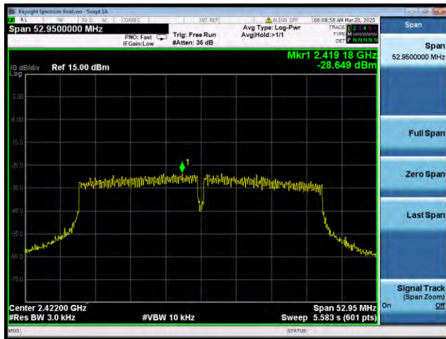
802.11n_Band2.4G_BW40MHz_2422MHz
