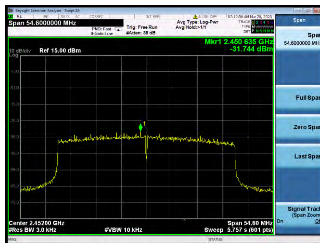
802.11ax_Band2.4G_BW40MHz_2452MHz
