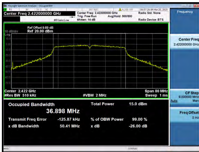
802.11n_Band2.4G_BW40MHz MHz
