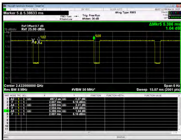
802.11n_Band2.4G BW40MHz 2422MHz
