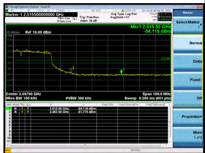
802.11ax_Band2.4G_BW40MHz
