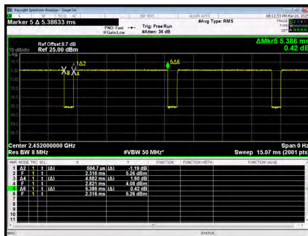
802.11n_Band2.4G BW40MHz 2452MHz
