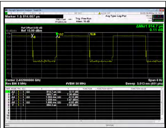
Bluetooth Low Energy 2Mbps 2402MHz
