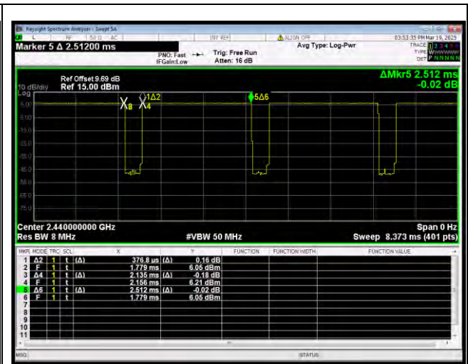
Bluetooth Low Energy 1Mbps 2440MHz
