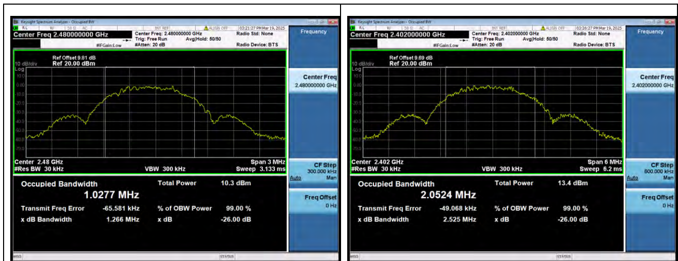
Bluetooth Low Energy 1Mbps 2480MHz
