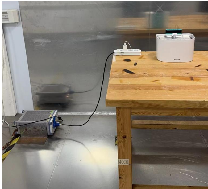
Radiated Spurious Emissions Test Frequency From Below 30MHz
