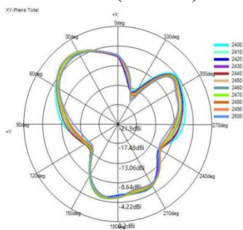
X-Y Plane(unit:dBi):
