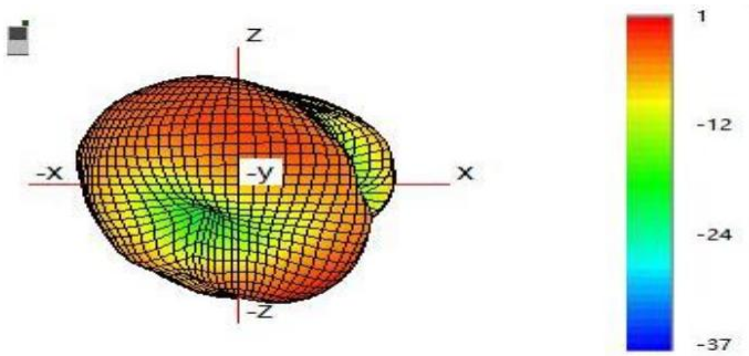
Typicall Free Space 3D Radiation Pattern at 2400MHz(unit:dBi)
