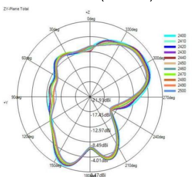
Y-Z Plane(unit:dBi):
