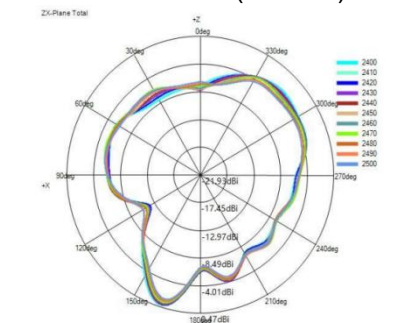
X-Z Plane(unit:dBi):
