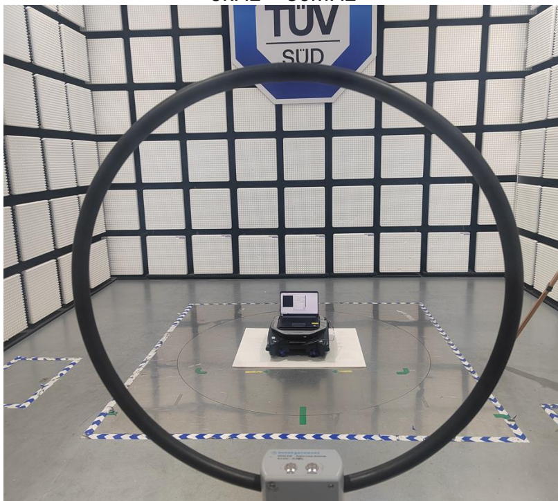
Radiated Emission Setup 9kHz ~ 30MHz
