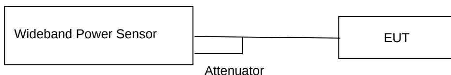
Power meter conducted test setup
