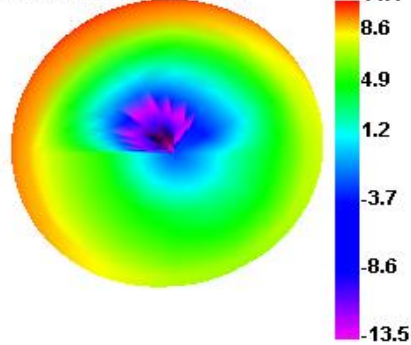
Bluetooth 0 TRP
