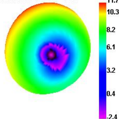
Bluetooth 78 TRP
