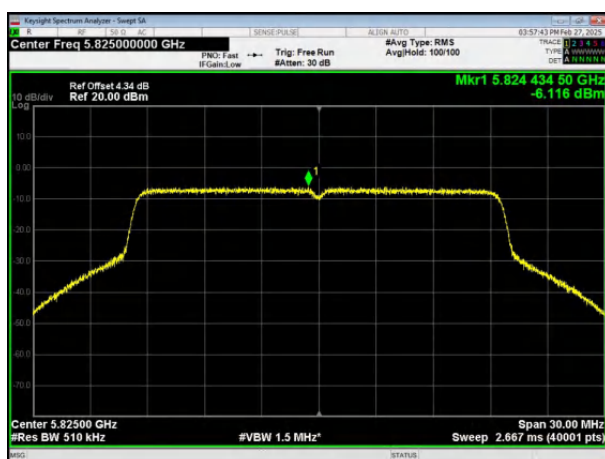
(802.11ax20) PSD plot on channel 165
