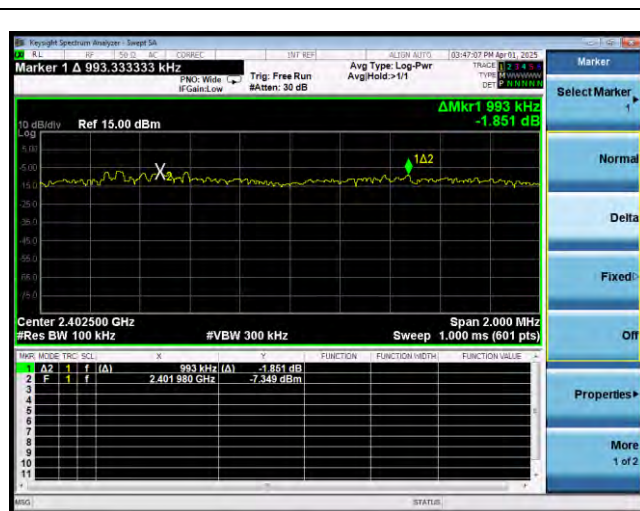
Bluetooth For Classic 2-DH5 2402MHz
