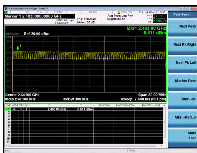
Bluetooth For Classic 1-DH5
