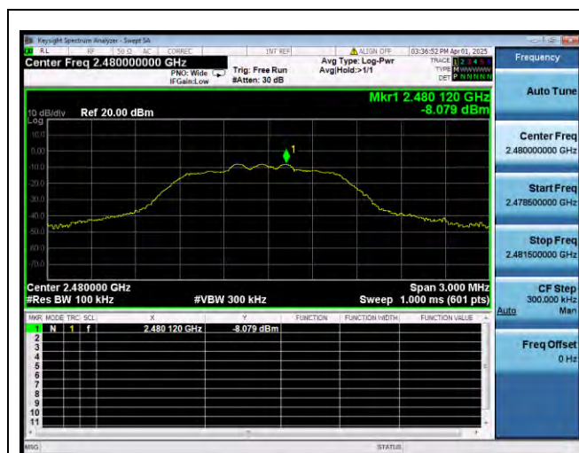
Bluetooth For Classic 2-DH5
