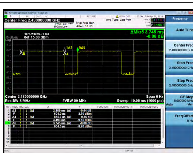
Bluetooth For Classic 2-DH5 2480MHz
