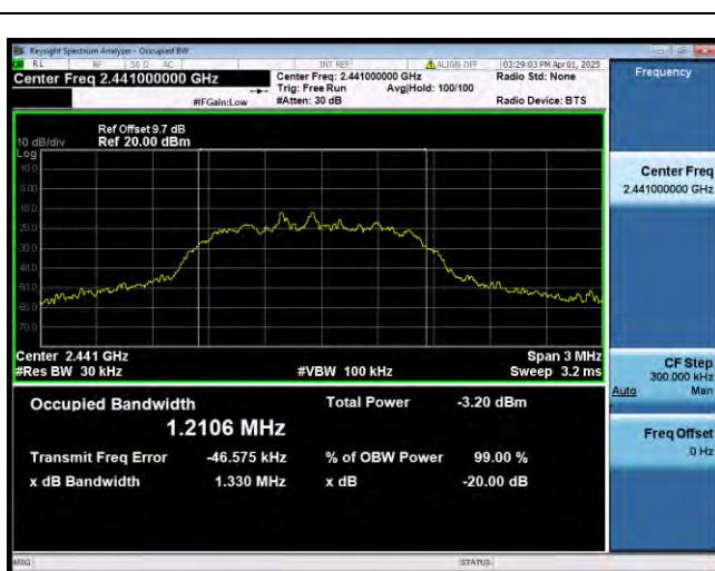
Bluetooth For Classic 2-DH5 2441MHz
