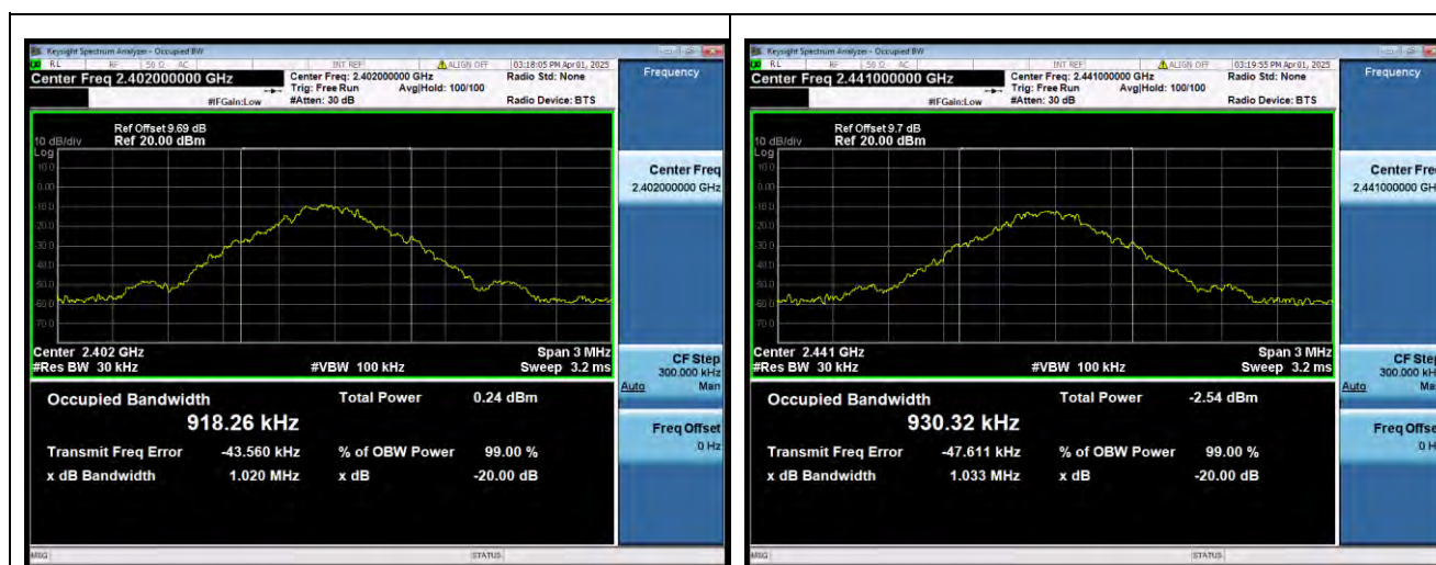
Bluetooth For Classic 1-DH5 2402MHz
