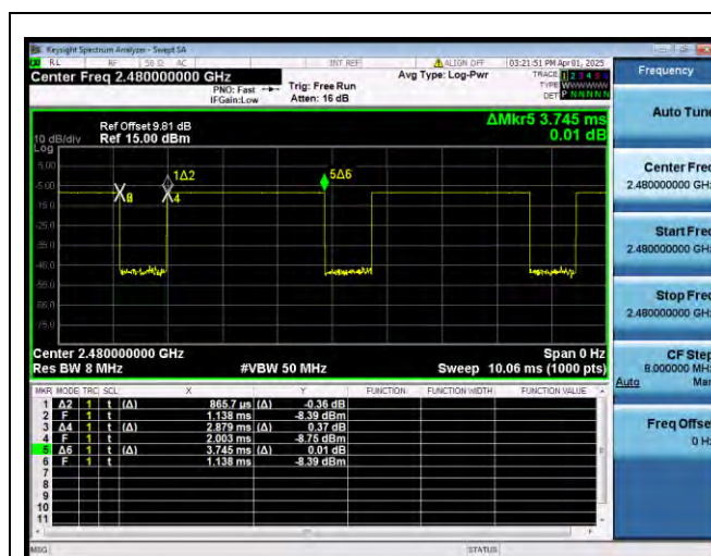
Bluetooth For Classic 1-DH5 2480MHz
