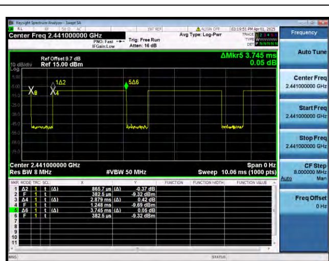
Bluetooth For Classic 1-DH5 2441MHz
