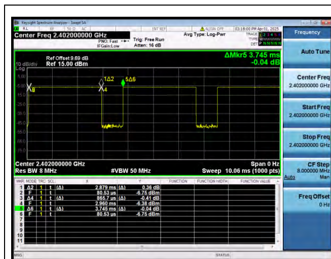
Bluetooth For Classic 1-DH5 2402MHz
