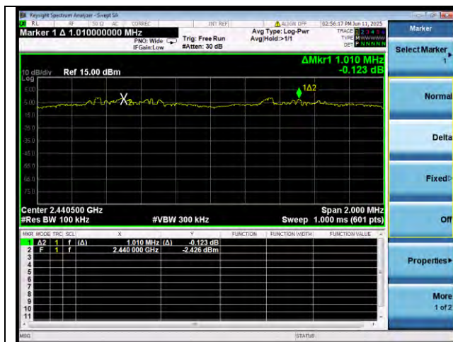
Bluetooth 2DH5 2440MHz
