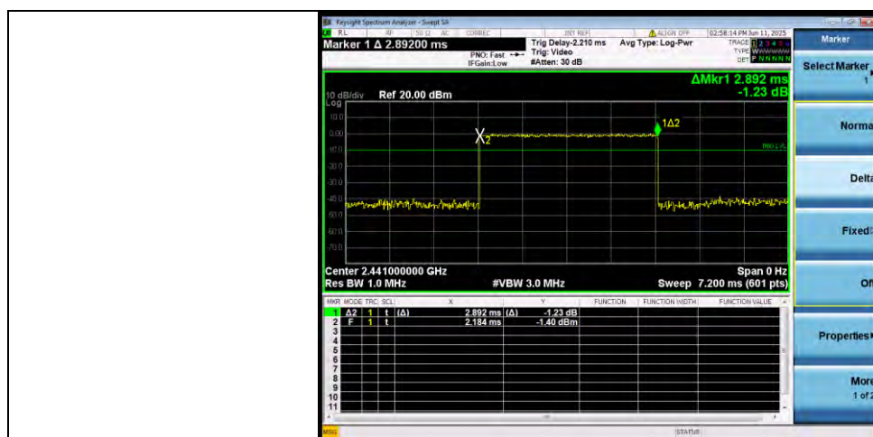
Bluetooth For Classic 3DH5 2441MHz
