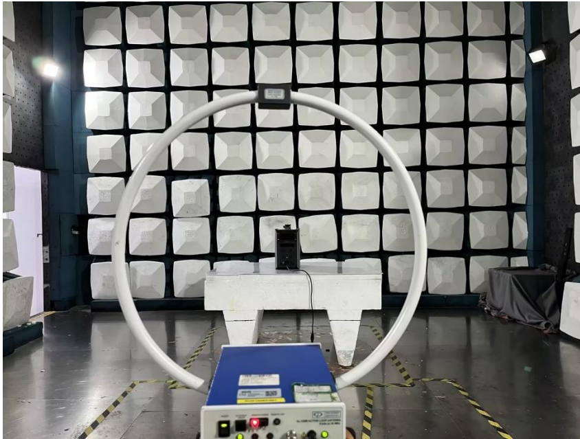
Radiated Emissions (9kHz-30MHz)
