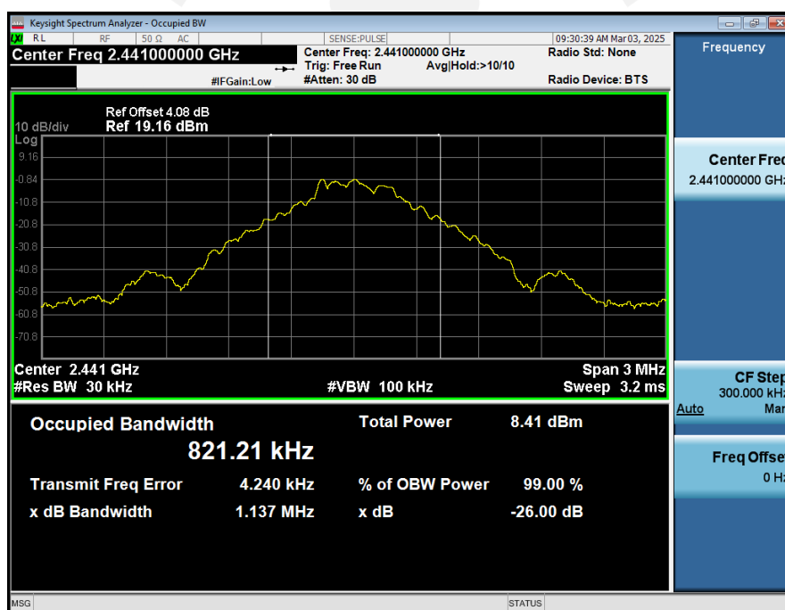
99%_Occupied_Bandwidth_NVNT_ANT1_1-DH1_2441_00
