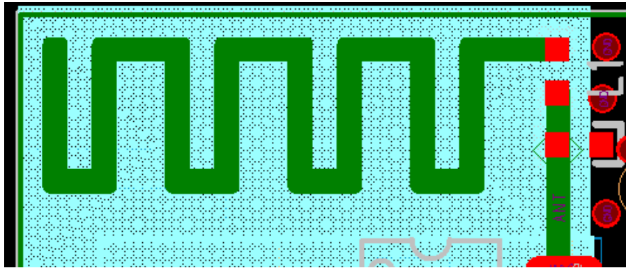
Figure 2 : Antenna
