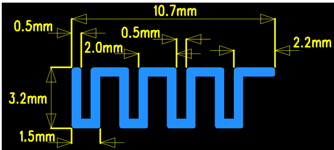
Figure 1 : Antenna size
