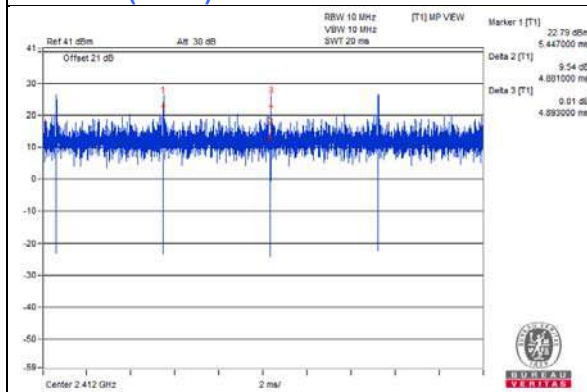
802.11ax (RU26)
