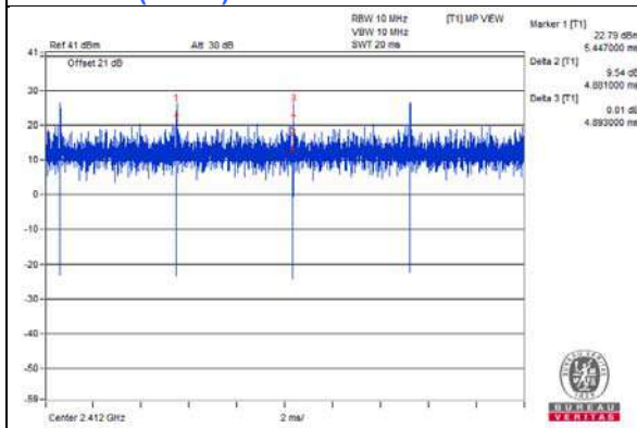
802.11ax (RU26)
