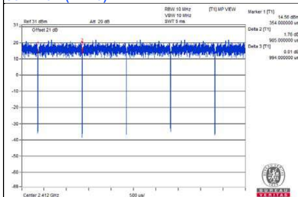
802.11ax (RU26)
