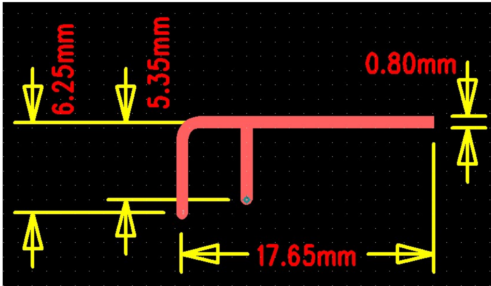
Antenna1 Photo & Length (mm)
