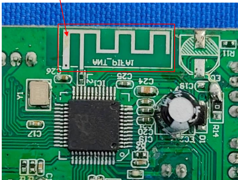
PCB Antenna
