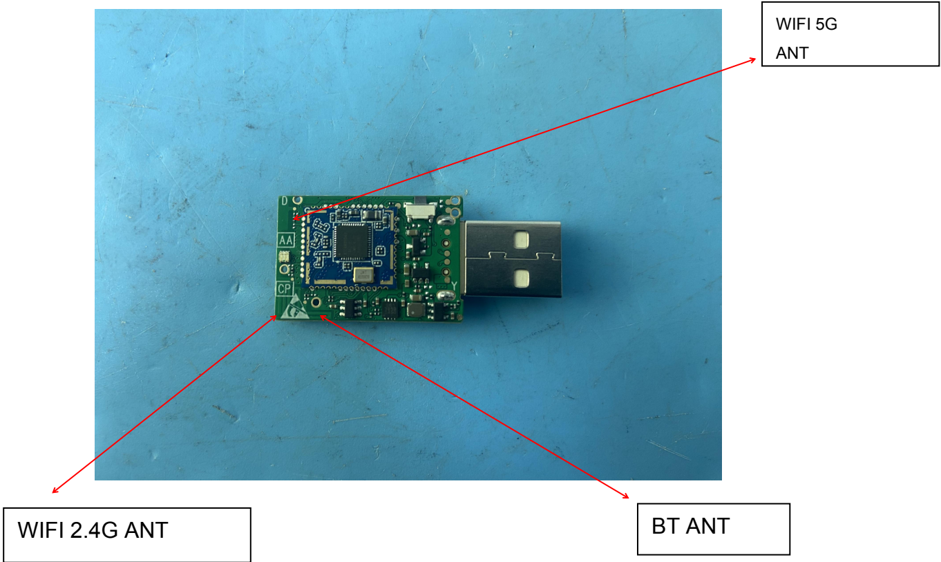
INTERNAL PHOTO OF SAMPLE PCB
