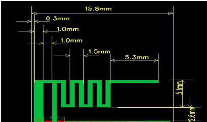
Antenna Photo & Length (mm)
