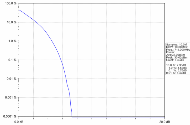
Band12 10MHz QPSK HCH 711MHz RB 50 0 NTN
