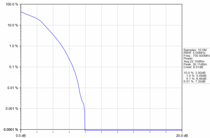
Band12 3MHz 16QAM LCH 700.5MHz RB 15 0 NTNV
