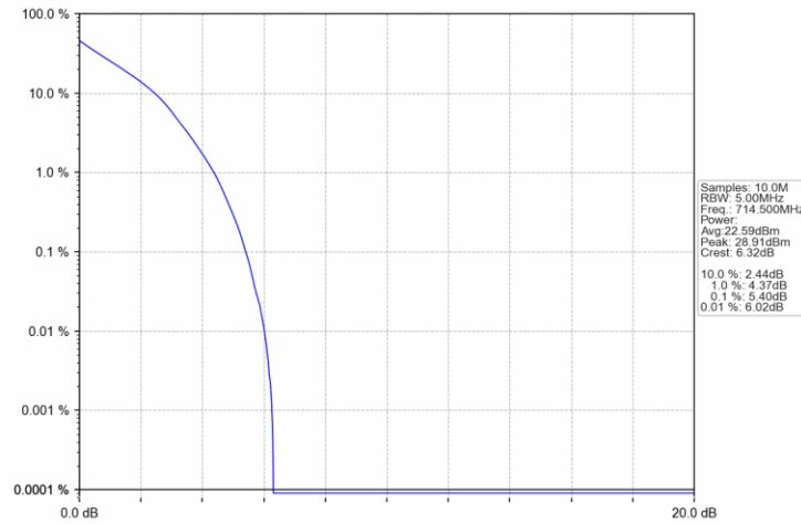
Band12 3MHz QPSK HCH 714.5MHz RB 15 0 NTNV
