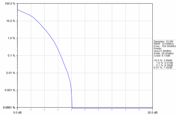
Band12 10MHz 16QAM LCH 704MHz RB 50 0 NTN
