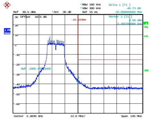
802.11g_2462MHz
