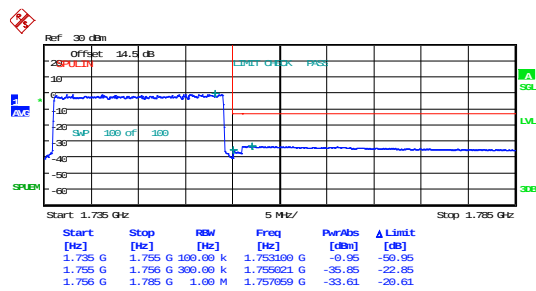
20MHz_High_16QAM_100@0
