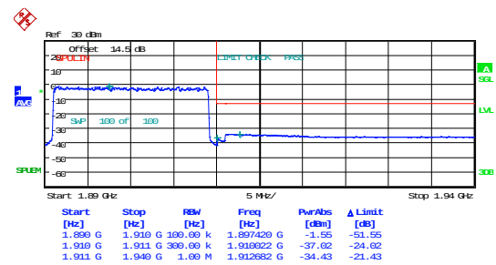
20MHz_High_16QAM_100@0
