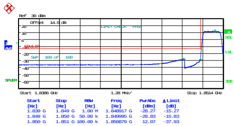
1.4MHz_Low_QPSK_6@0
