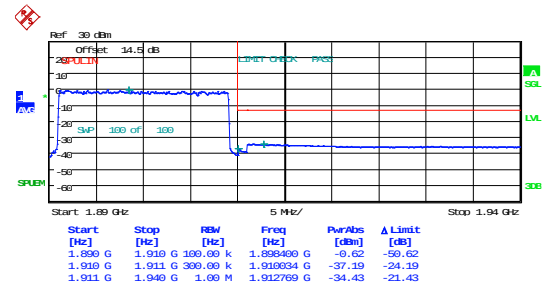
20MHz_High_QPSK_100@0
