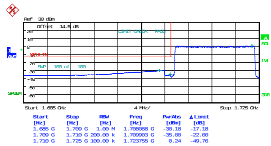
15MHz_Low_QPSK_75@0
