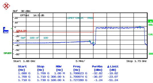
20MHz_Low_16QAM_100@0
