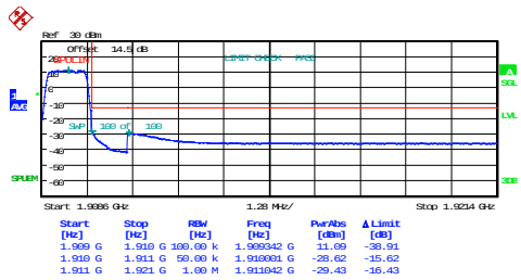
1.4MHz_High_QPSK_6@0
