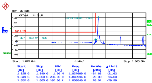
15MHz_Low_16QAM_1@0
