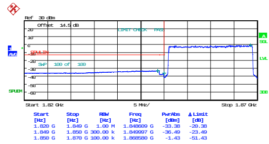
20MHz_Low_16QAM_100@0
