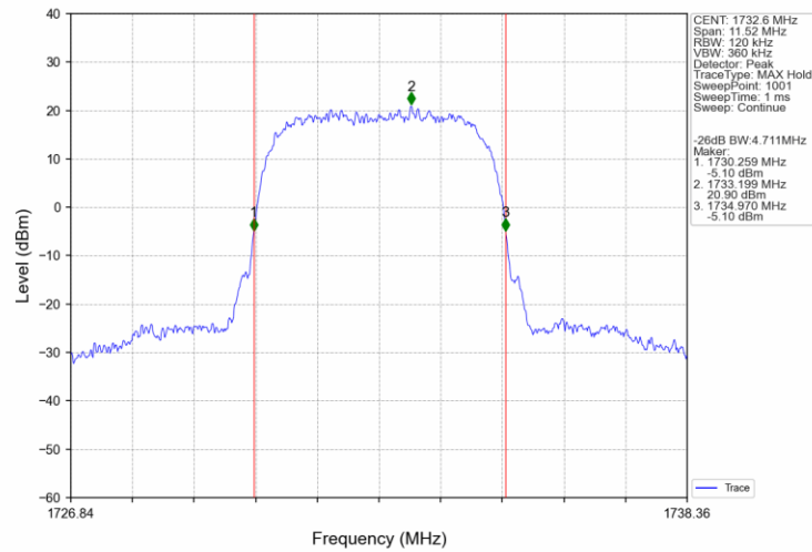
Band4 RMC MCH 1732.6MHz 12.2kbps RMC NTN
